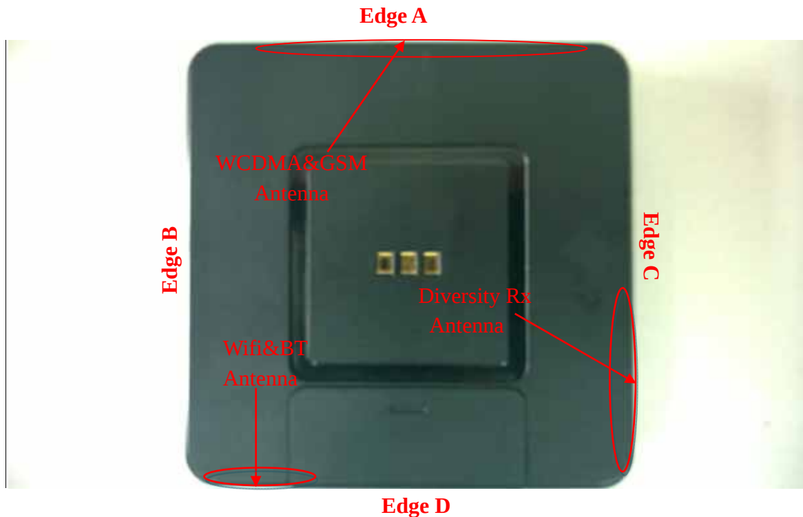
Stand-alone SAR
