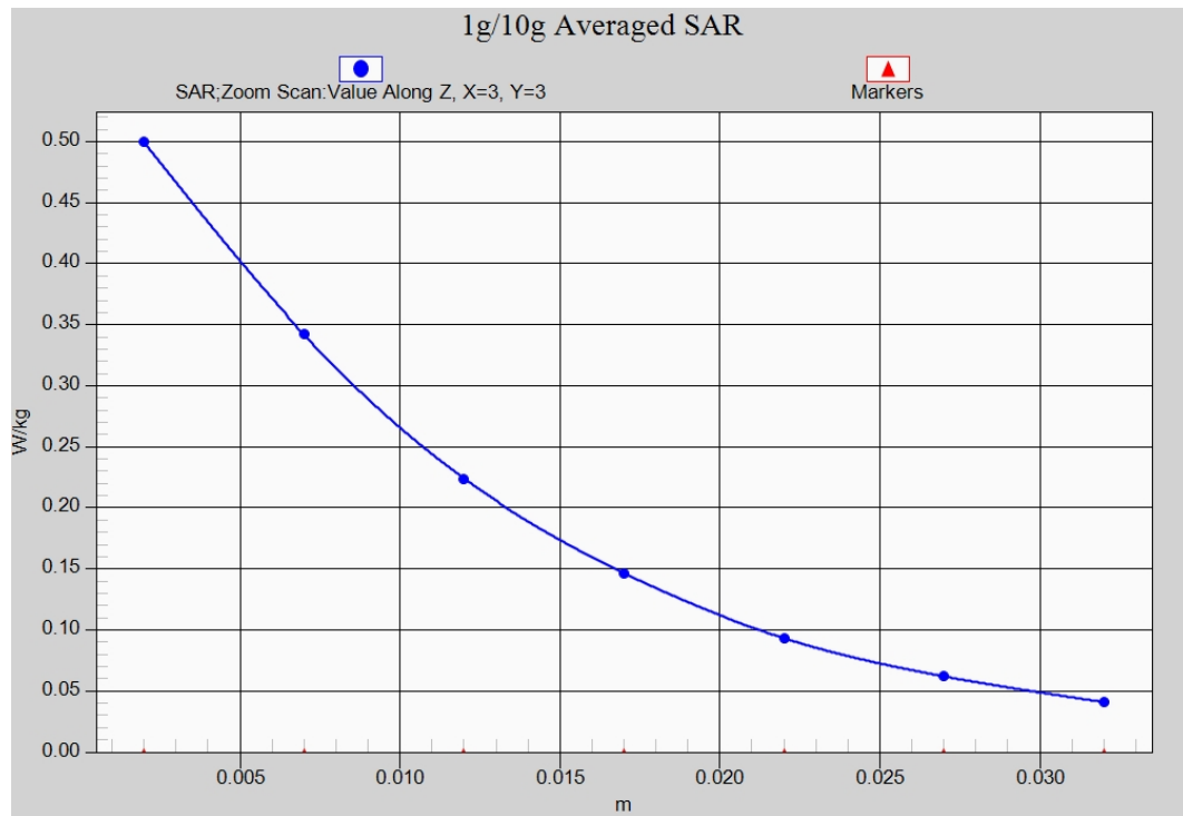
Fig. 13-1 Z-Scan at power reference point (LTE Band2 CH18700)
