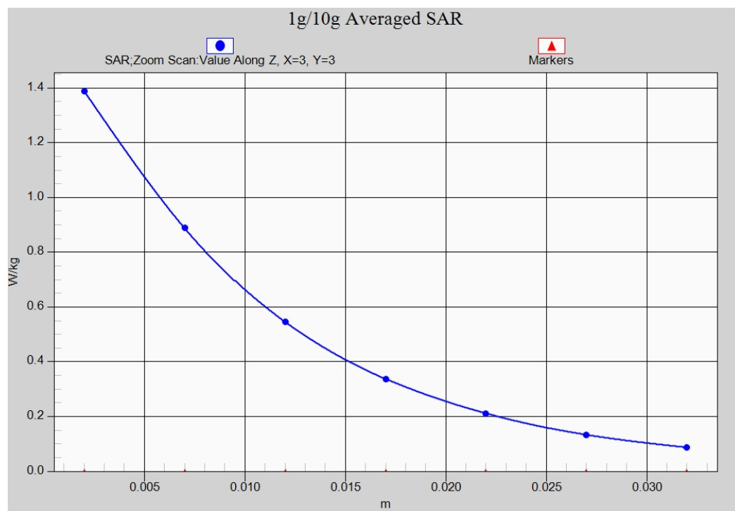
Fig. 16-1 Z-Scan at power reference point (LTE Band4 CH20300)
