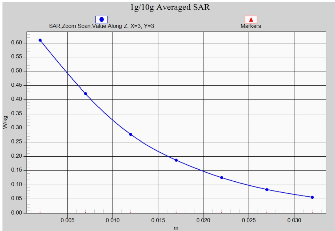
Fig. 15-1 Z-Scan at power reference point (LTE Band4 CH20300)
