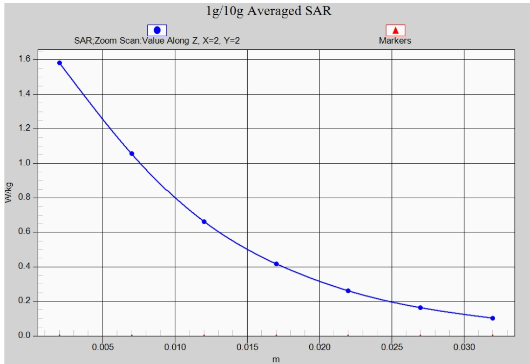
Fig. 14-1 Z-Scan at power reference point (LTE Band2 CH19100)
