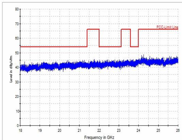
FCC-RSE-18-26G
