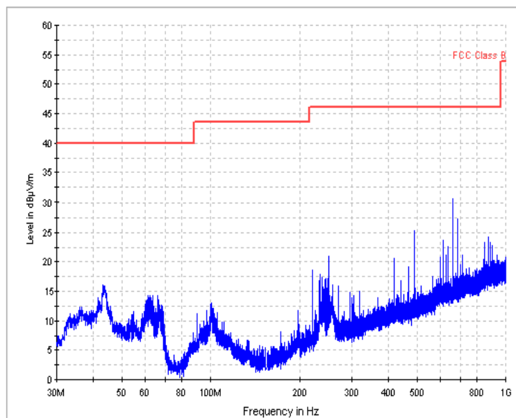
FCC-RE1-Part 15-30M-1G
