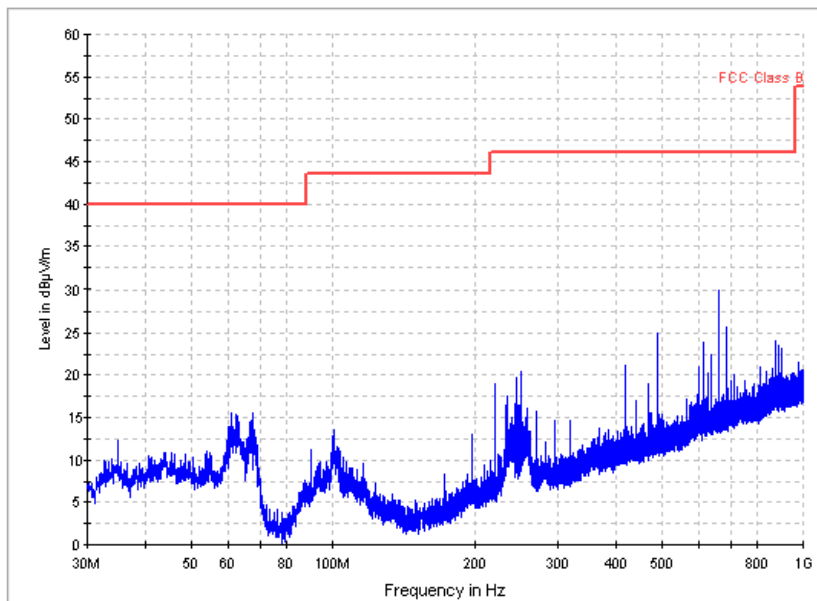
FCC-RE1-Part 15-30M-1G
