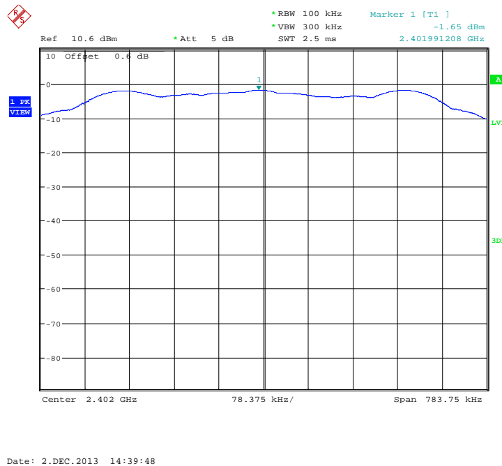
Fig.33. Maximum Power Spectral Density Level Function: GFSK, 2402 MHz
