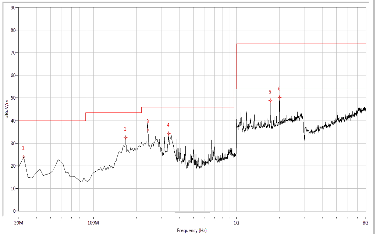
(Plot C: 30MHz – 8GHz Test Antenna Horizontal)
