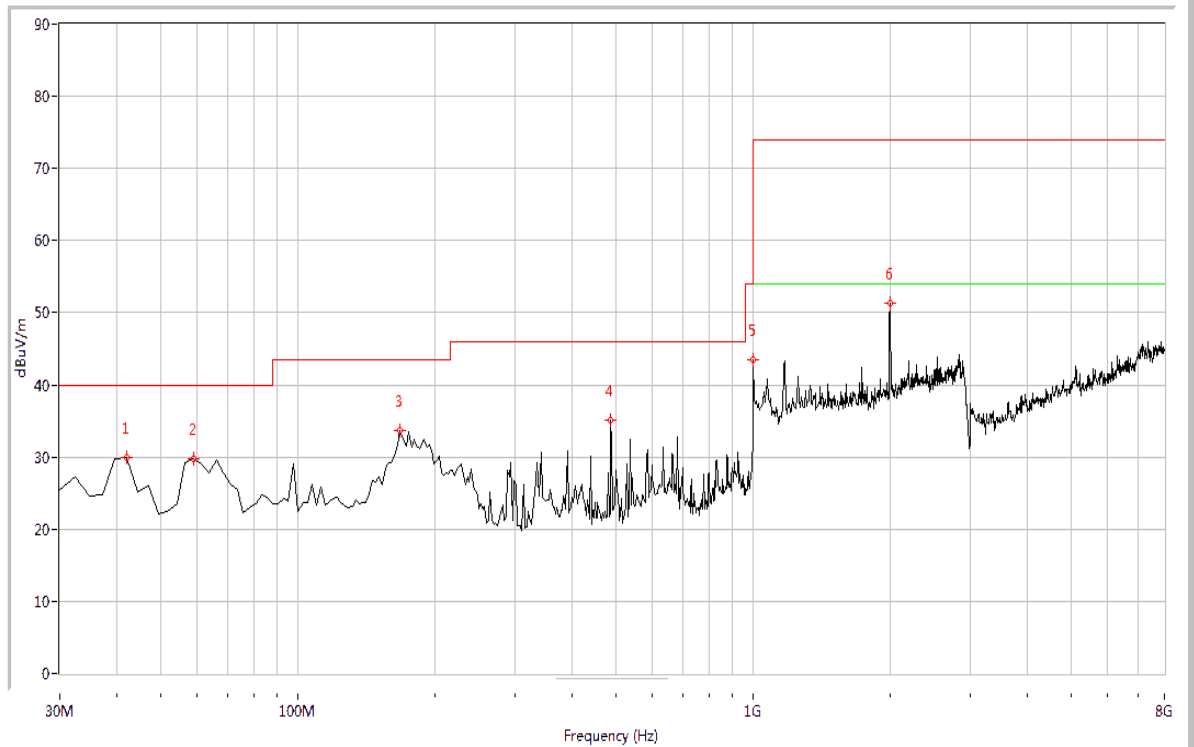
(Plot B: 30MHz – 8GHz Test Antenna Vertical)
