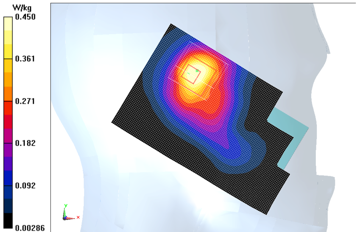
Fig.7 2450 MHz CH11
