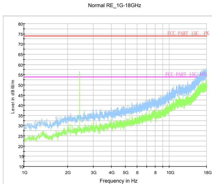
Fig.63. Radiated emission: GFSK, Channel 78, 1 GHz - 18 GHz
