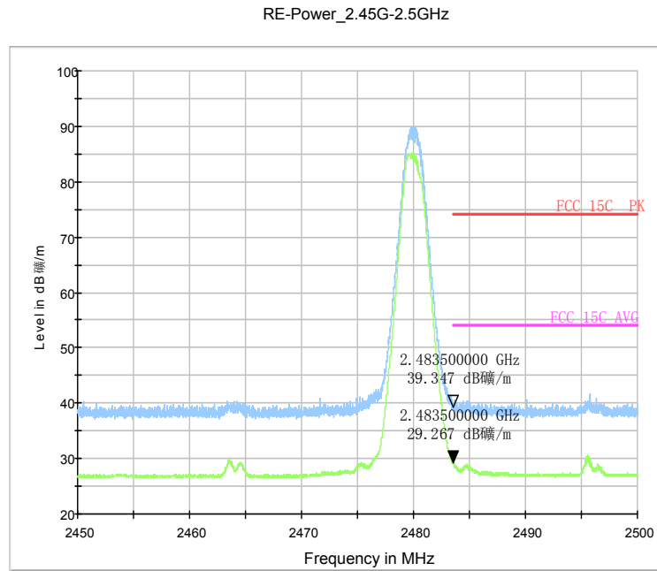
Fig.83. Radiated emission (Power): 8DPSK, high channel
