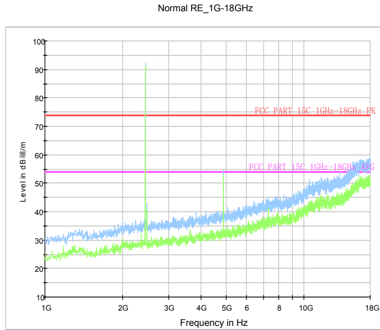
Fig.61. Radiated emission: GFSK, Channel 39, 1 GHz - 18 GHz
