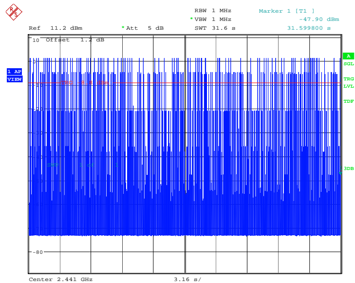
Fig.99. Time of occupancy (Dwell Time): Channel 39, Packet 3-DH3
