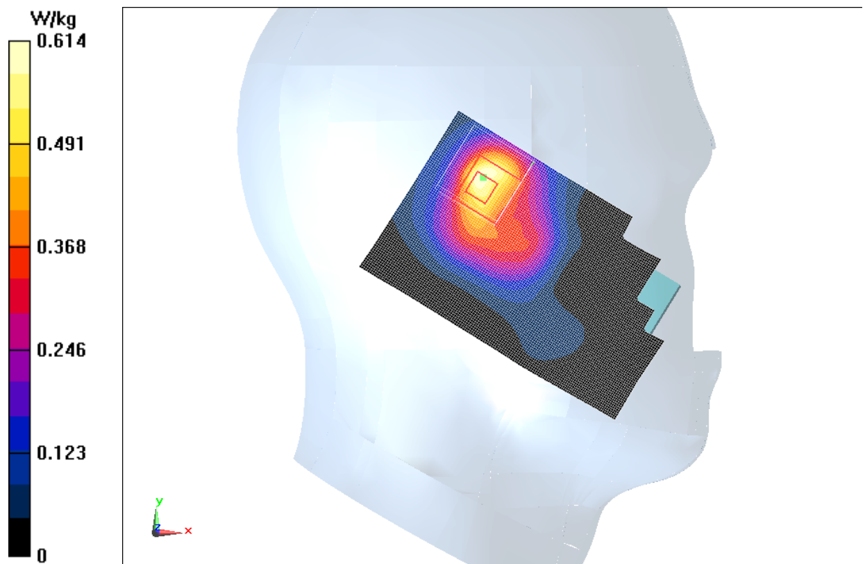
Fig.9 2450 MHz CH11
