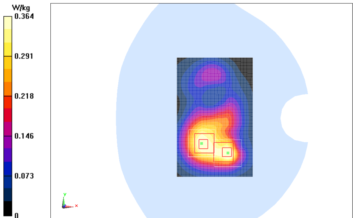
Fig.10 2450 MHz CH11
