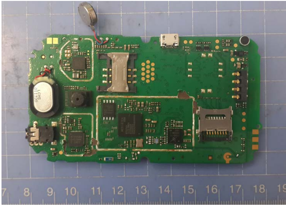
Mobile Phone Disassembly
