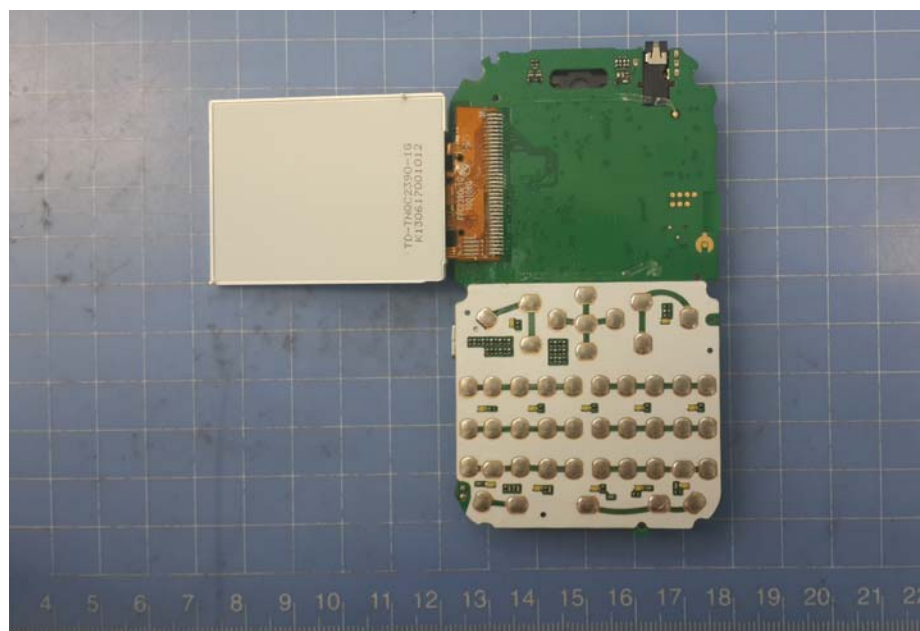
Mobile Phone Disassembly
