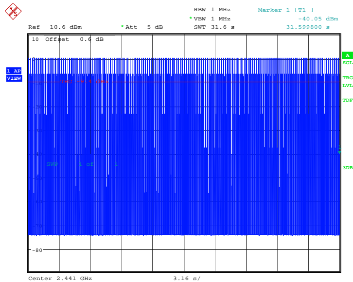
Fig.100. Time of occupancy (Dwell Time): Channel 39, Packet DH1
