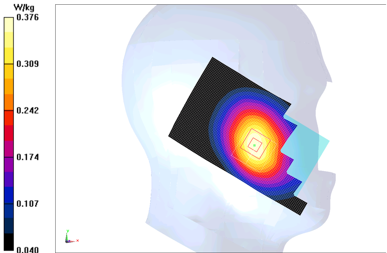
Fig.J.5 WCDMA 850MHz Head CH4233
