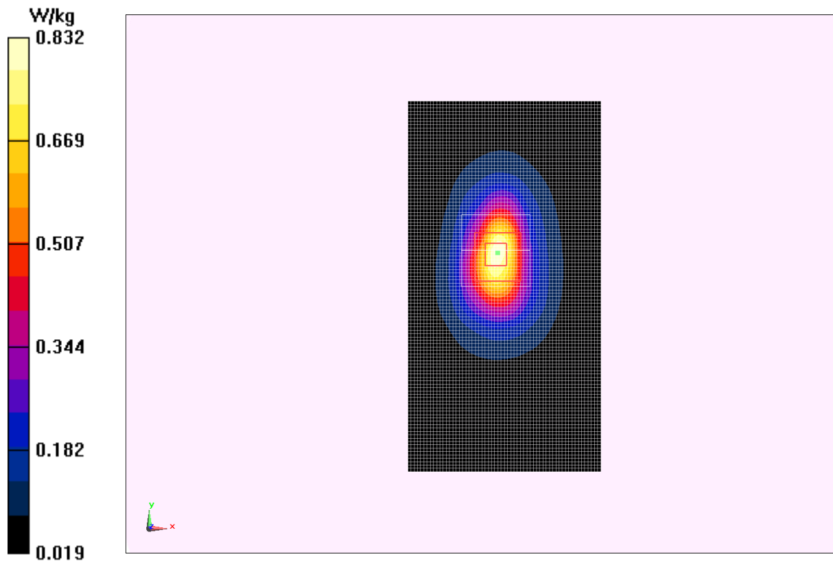
Fig.4 1900 MHz CH810
