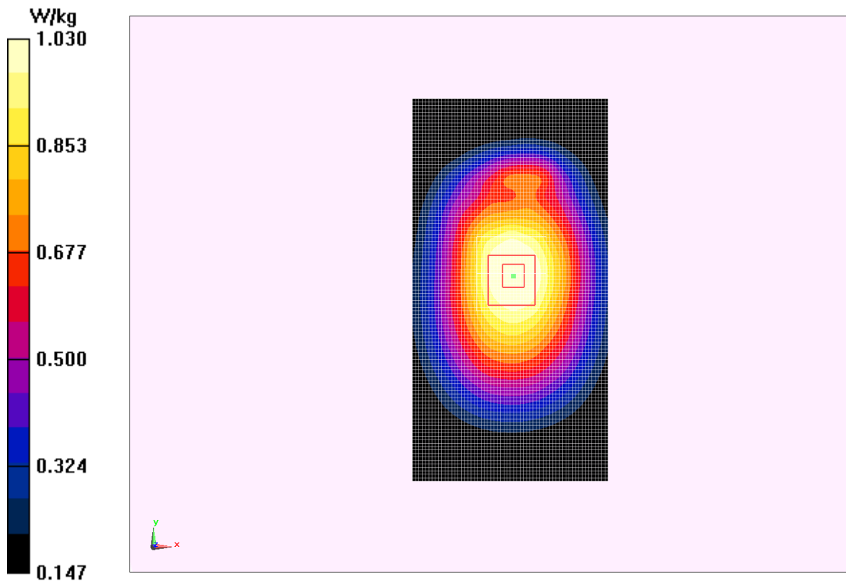
Fig.2 850 MHz CH251
