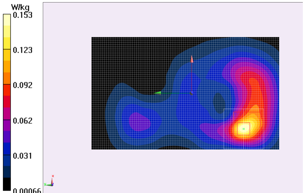
Fig.10 2450 MHz CH6
