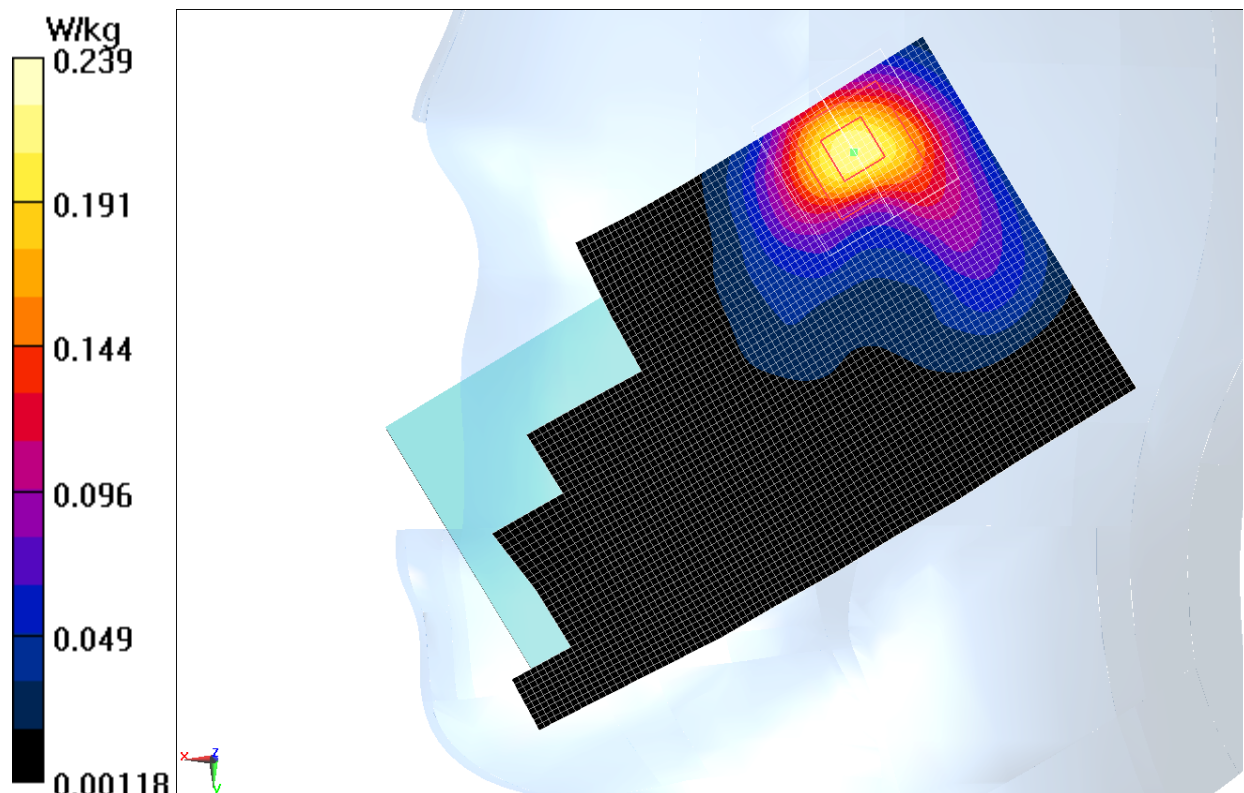
Fig.9 2450 MHz CH6
