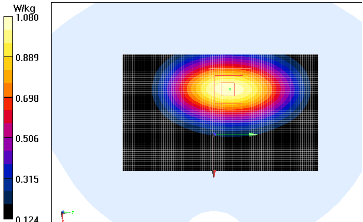
Fig.2 850 MHz CH251
