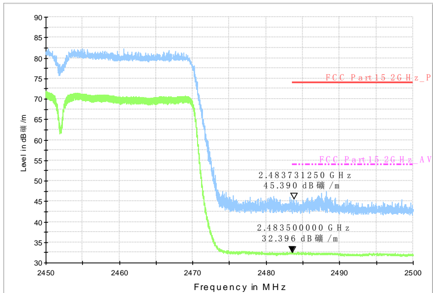
RE-Power_2.45G-2.5GHz
