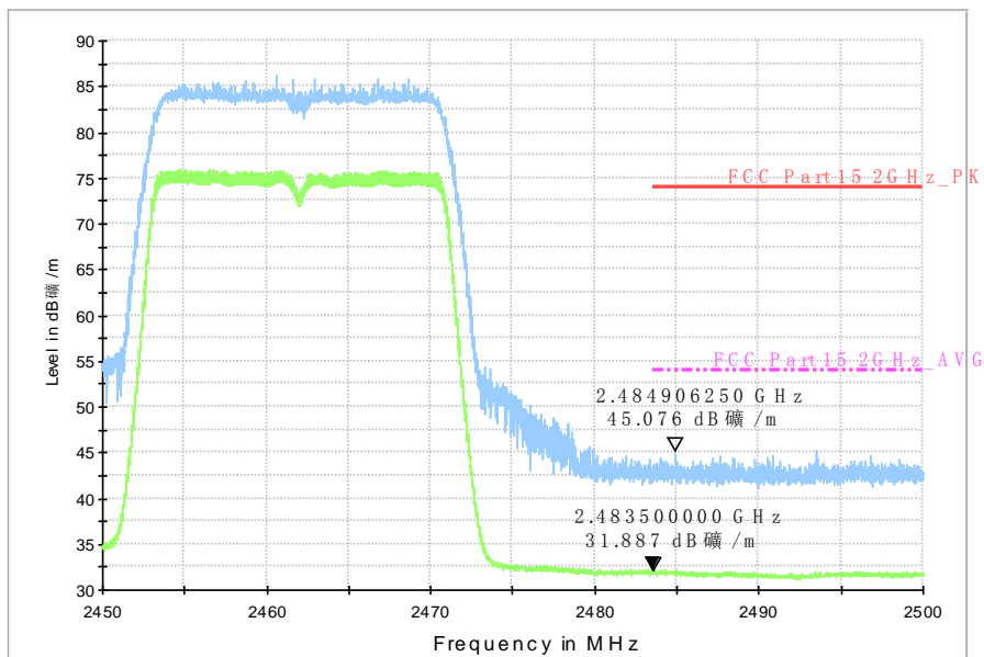
RE-Power_2.45G-2.5GHz
