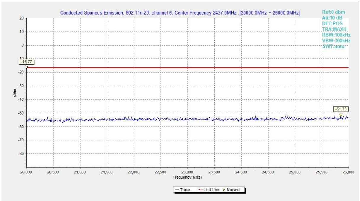
Fig.A.6.1.63 Transmitter Spurious Emission - Conducted (802.11n-HT20, Ch6, 20 GHz-26 GHz)
