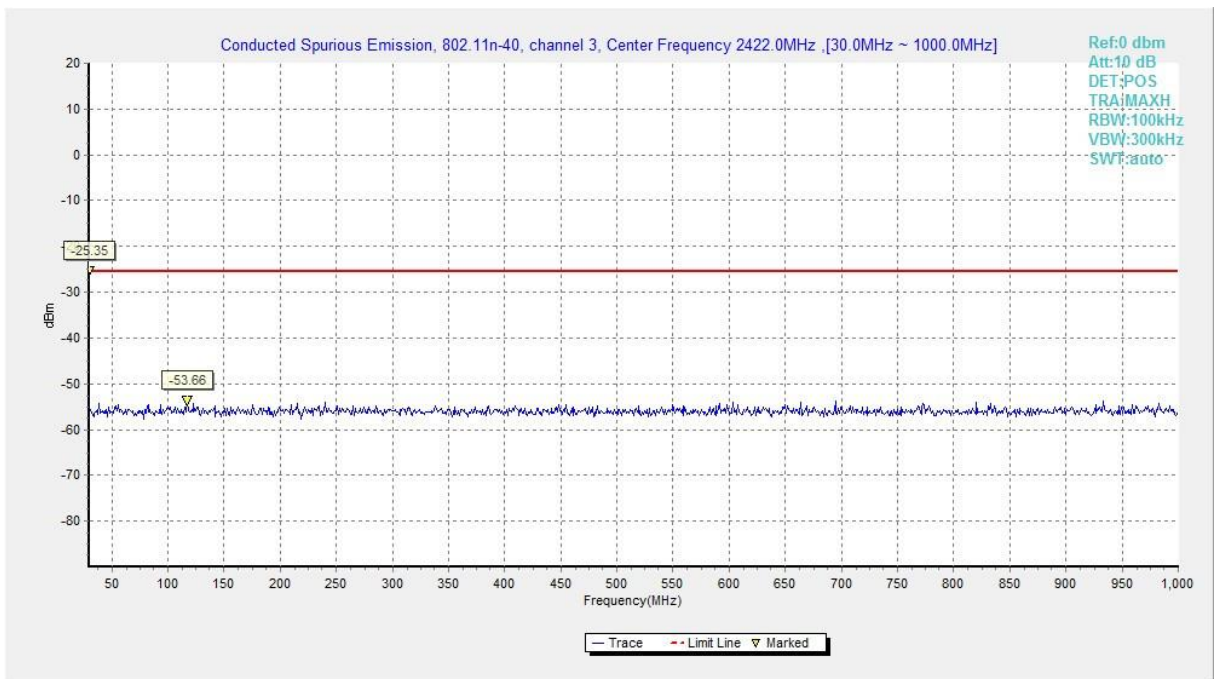
Fig.A.6.1.73 Transmitter Spurious Emission - Conducted (802.11n-HT40, Ch3, 30 MHz-1 GHz)
