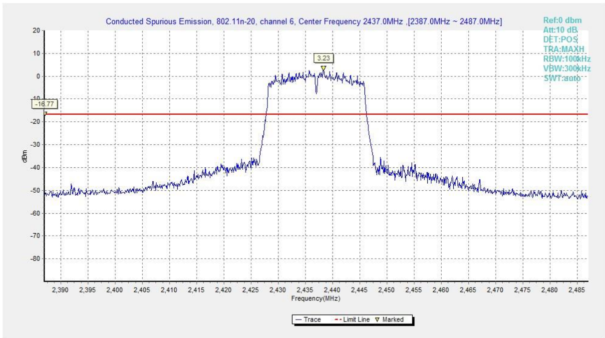
Fig.A.6.1.56 Transmitter Spurious Emission - Conducted (802.11n-HT20, Ch6, Center Frequency)
