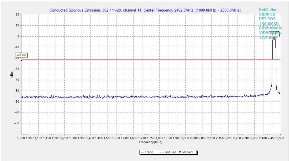
Fig.A.6.1.66 Transmitter Spurious Emission - Conducted (802.11n-HT20, Ch11, 1 GHz-2.5 GHz)
