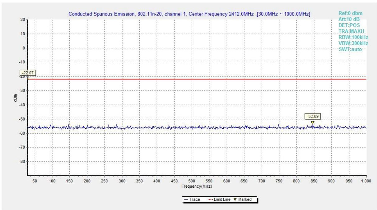
Fig.A.6.1.49 Transmitter Spurious Emission - Conducted (802.11n-HT20, Ch1, 30 MHz-1 GHz)
