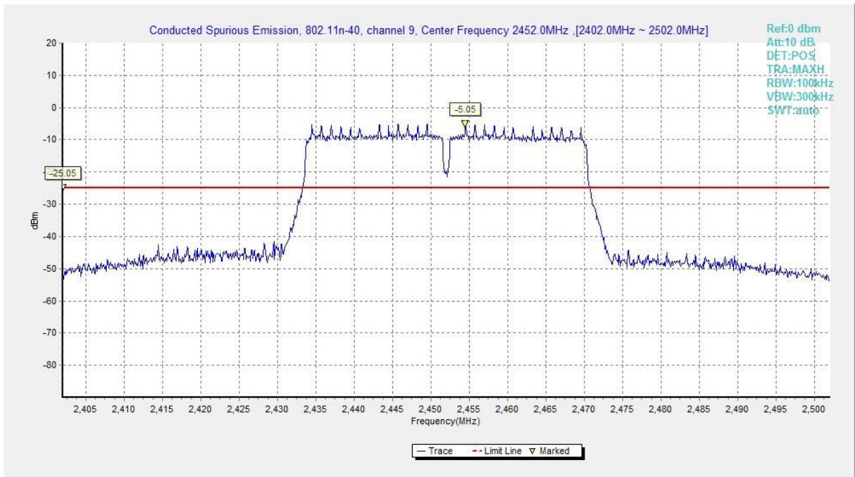
Fig.A.6.1.88 Transmitter Spurious Emission - Conducted (802.11n-HT40, Ch9, Center Frequency)
