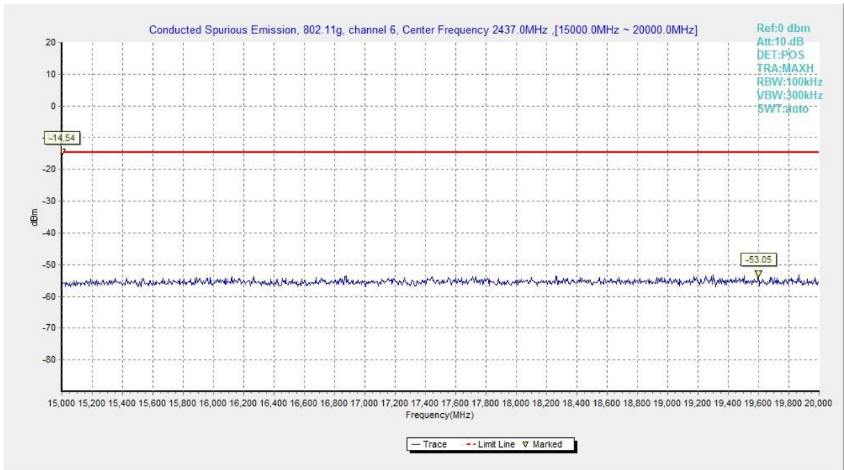
Fig.A.6.1.38 Transmitter Spurious Emission - Conducted (802.11g, Ch6, 15 GHz-20 GHz)
