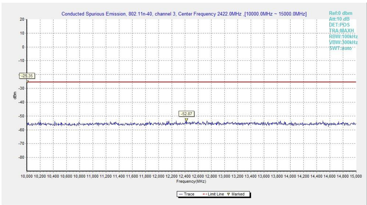
Fig.A.6.1.77 Transmitter Spurious Emission - Conducted (802.11n-HT40, Ch3, 10 GHz-15 GHz)
