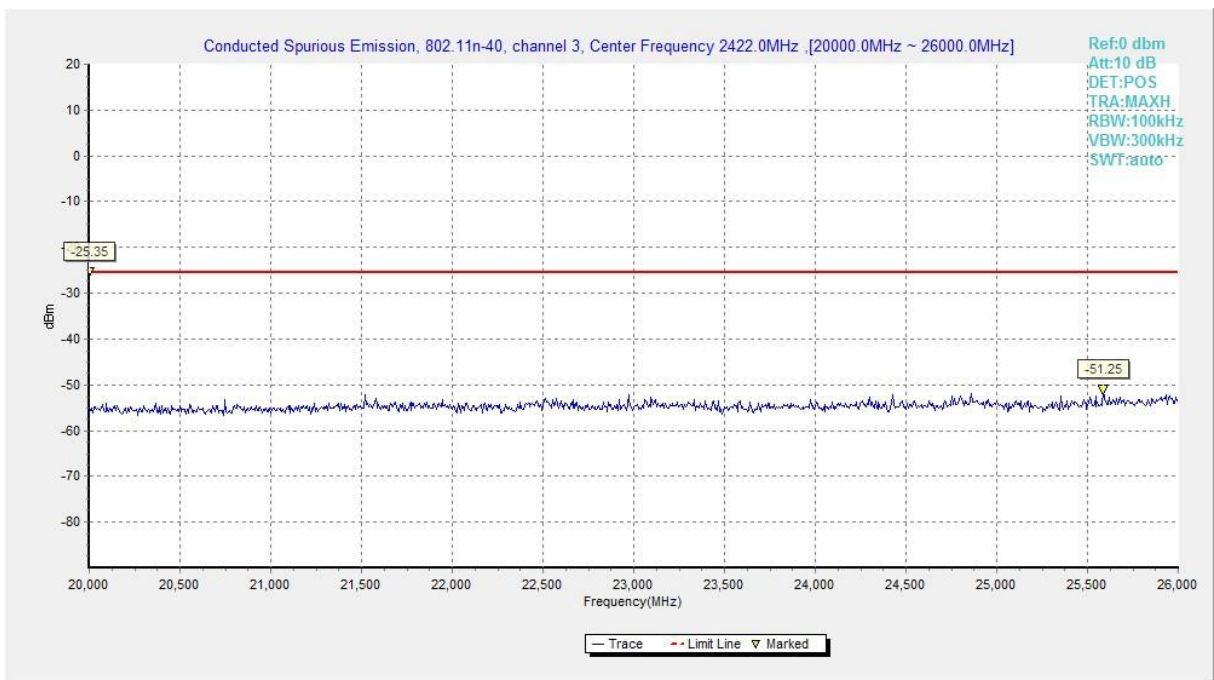
Fig.A.6.1.79 Transmitter Spurious Emission - Conducted (802.11n-HT40, Ch3, 20 GHz-26 GHz)
