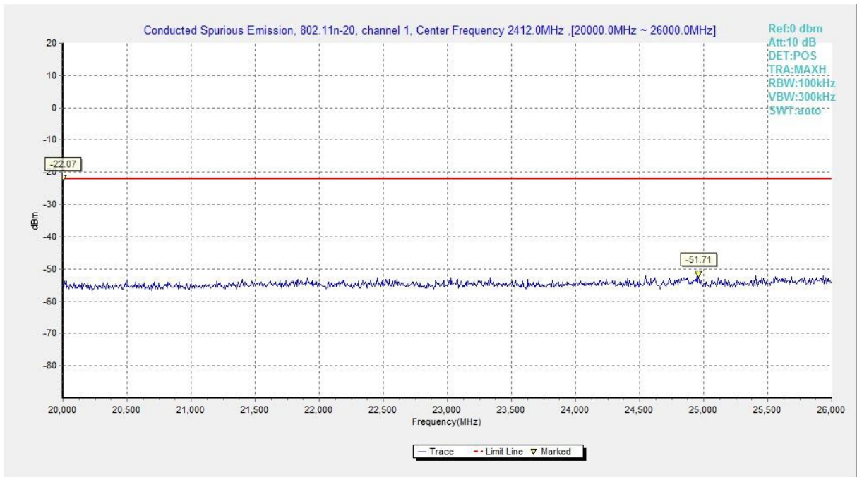
Fig.A.6.1.55 Transmitter Spurious Emission - Conducted (802.11n-HT20, Ch1, 20 GHz-26 GHz)
