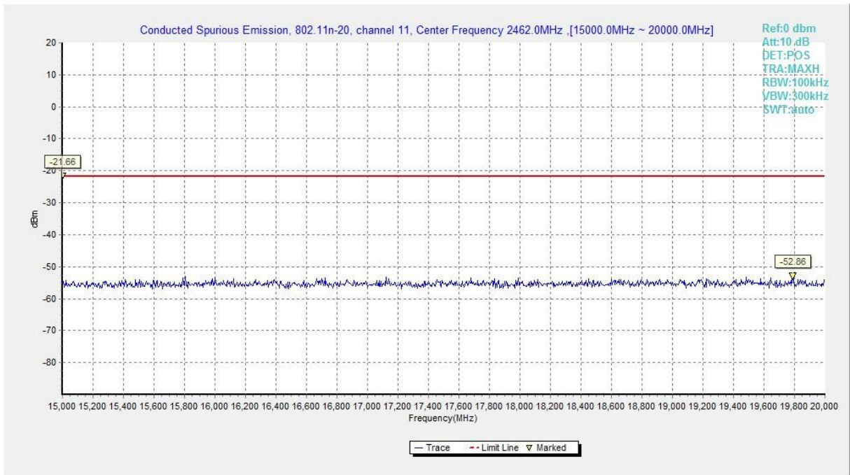
Fig.A.6.1.70 Transmitter Spurious Emission - Conducted (802.11n-HT20, Ch11, 15 GHz-20 GHz)
