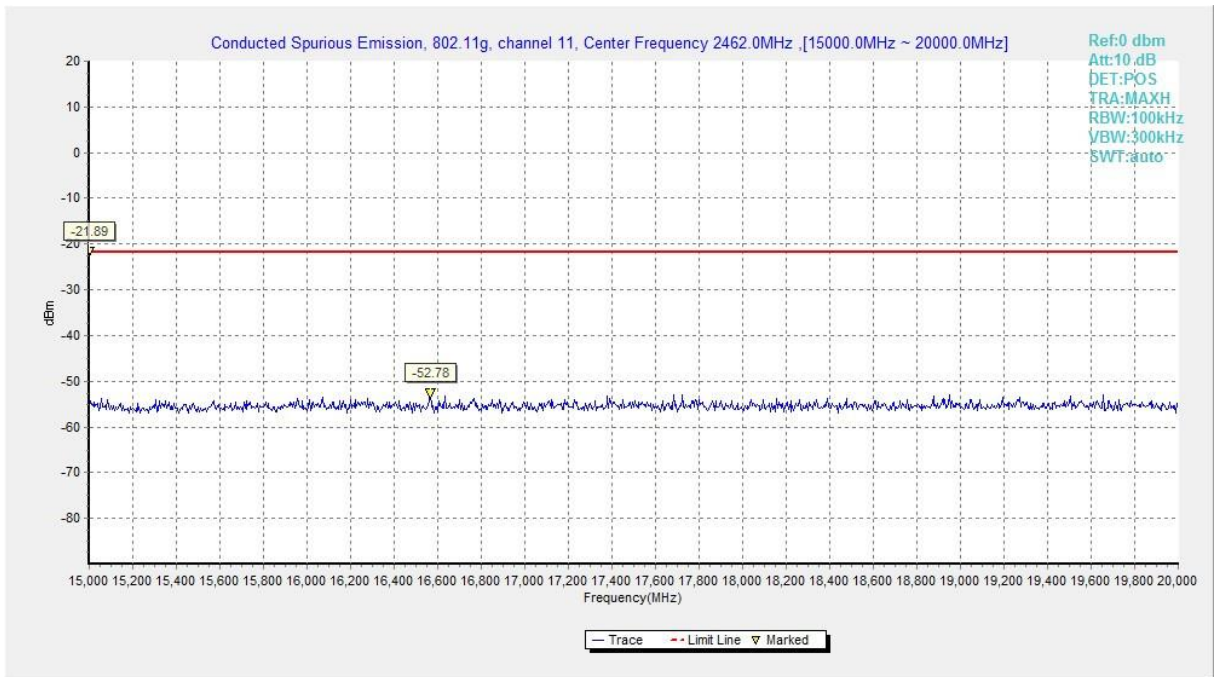
Fig.A.6.1.46 Transmitter Spurious Emission - Conducted (802.11g, Ch11, 15 GHz-20 GHz)
