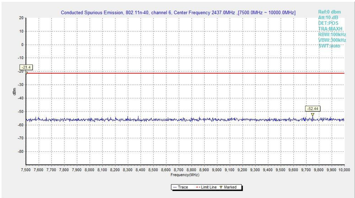
Fig.A.6.1.84 Transmitter Spurious Emission - Conducted (802.11n-HT40, Ch6, 7.5 GHz-10 GHz)
