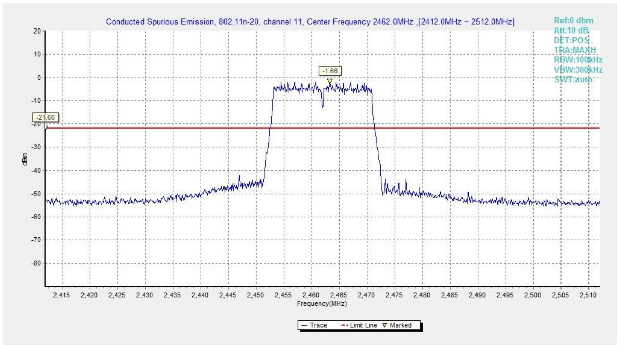
Fig.A.6.1.64 Transmitter Spurious Emission - Conducted (802.11n-HT20, Ch11, Center Frequency)
