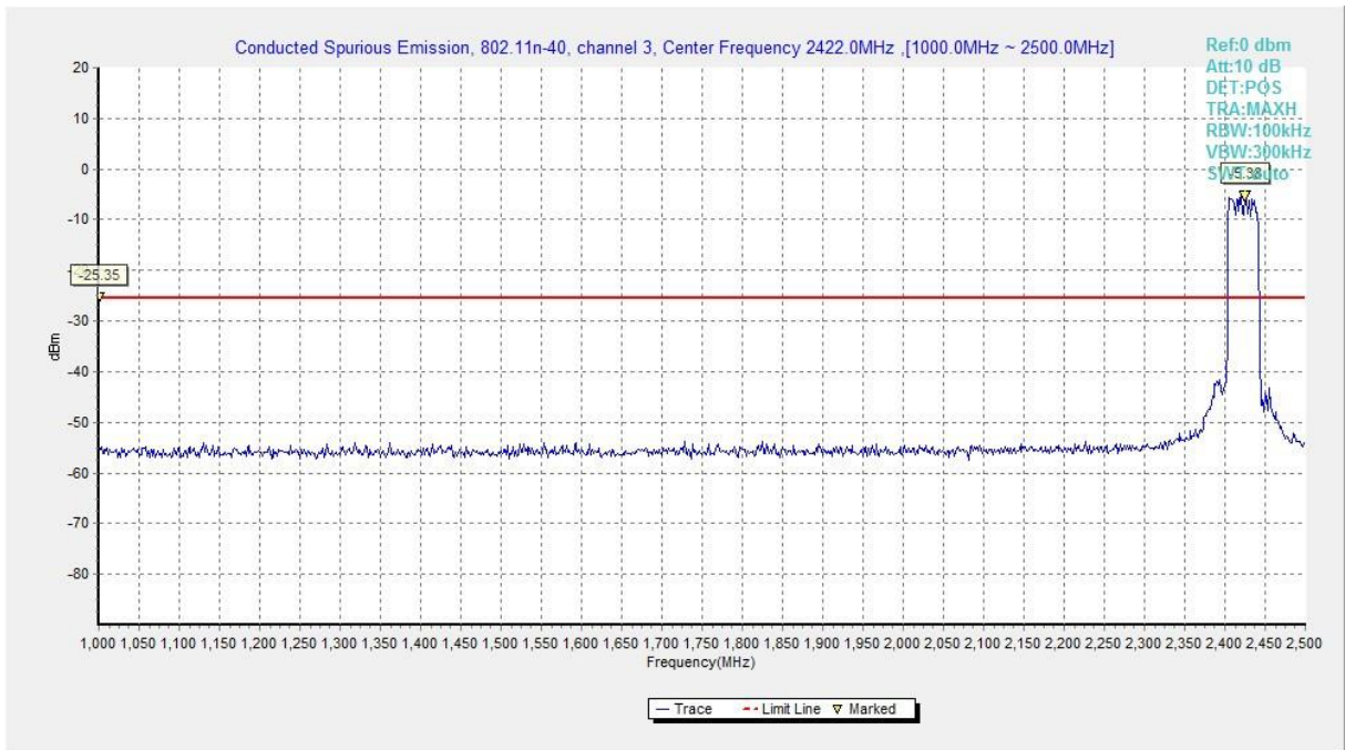
Fig.A.6.1.74 Transmitter Spurious Emission - Conducted (802.11n-HT40, Ch3, 1 GHz-2.5 GHz)
