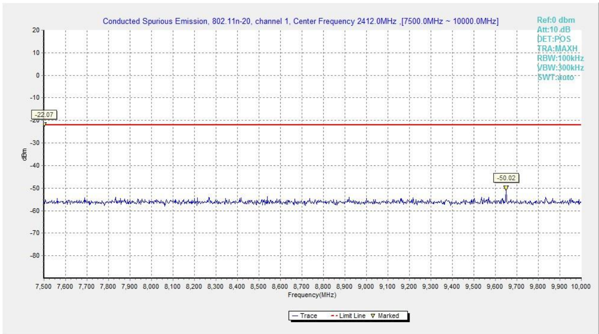
Fig.A.6.1.52 Transmitter Spurious Emission - Conducted (802.11n-HT20, Ch1, 7.5 GHz-10 GHz)
