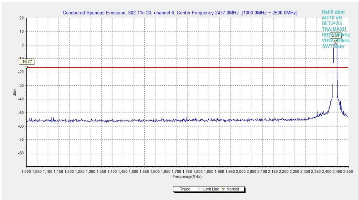
Fig.A.6.1.58 Transmitter Spurious Emission - Conducted (802.11n-HT20, Ch6, 1 GHz-2.5 GHz)
