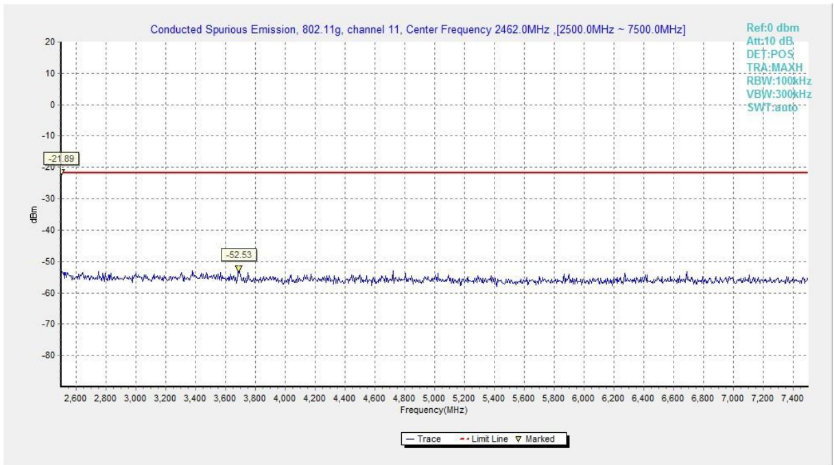
Fig.A.6.1.43 Transmitter Spurious Emission - Conducted (802.11g, Ch11, 2.5 GHz-7.5 GHz)
