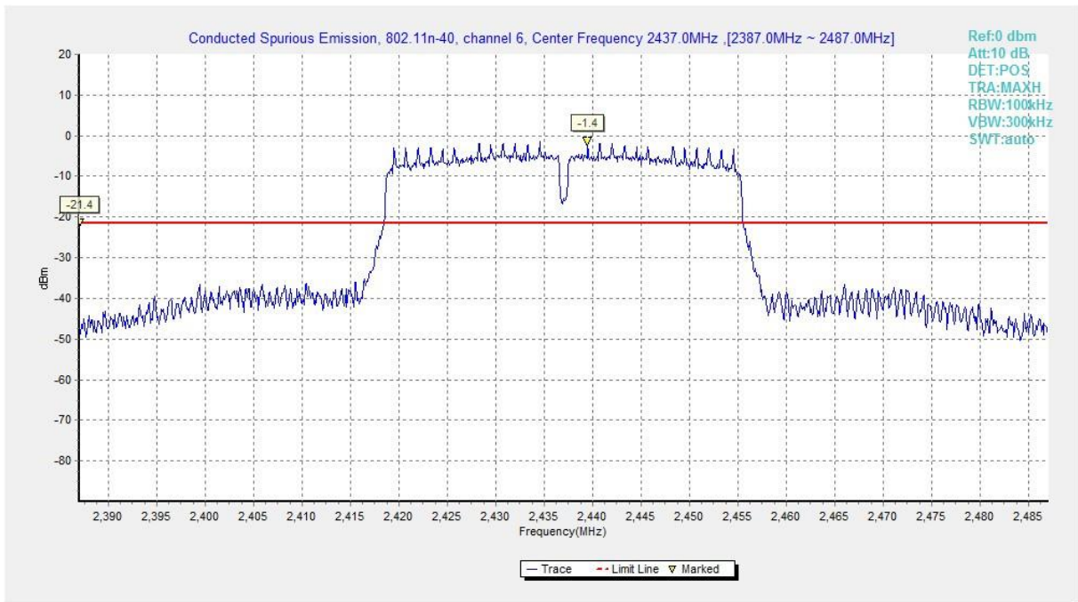
Fig.A.6.1.80 Transmitter Spurious Emission - Conducted (802.11n-HT40, Ch6, Center Frequency)
