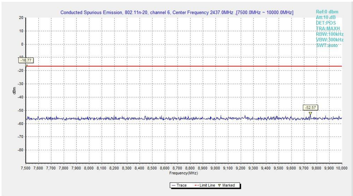
Fig.A.6.1.60 Transmitter Spurious Emission - Conducted (802.11n-HT20, Ch6, 7.5 GHz-10 GHz)
