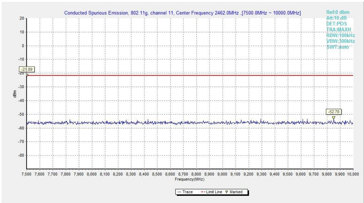
Fig.A.6.1.44 Transmitter Spurious Emission - Conducted (802.11g, Ch11, 7.5 GHz-10 GHz)
