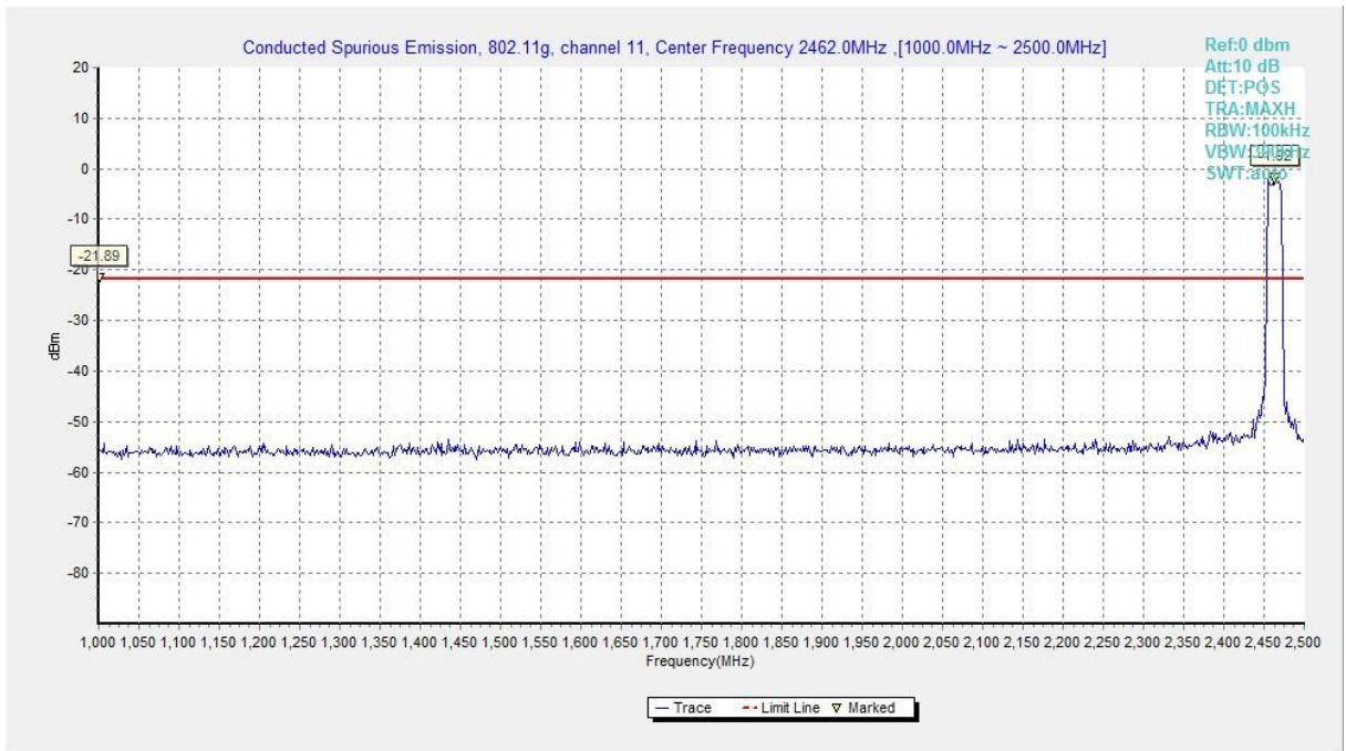
Fig.A.6.1.42 Transmitter Spurious Emission - Conducted (802.11g, Ch11, 1 GHz-2.5 GHz)
