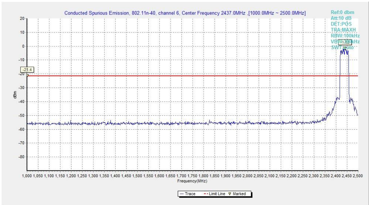
Fig.A.6.1.82 Transmitter Spurious Emission - Conducted (802.11n-HT40, Ch6, 1 GHz-2.5 GHz)
