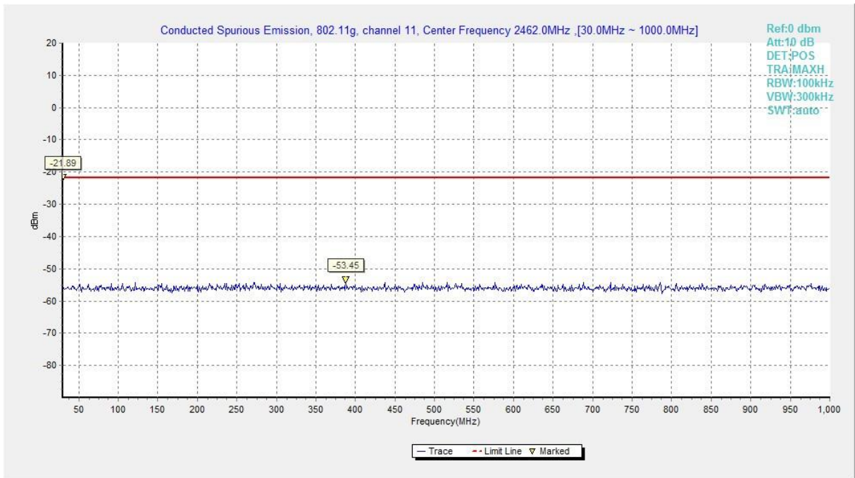
Fig.A.6.1.41 Transmitter Spurious Emission - Conducted (802.11g, Ch11, 30 MHz-1 GHz)
