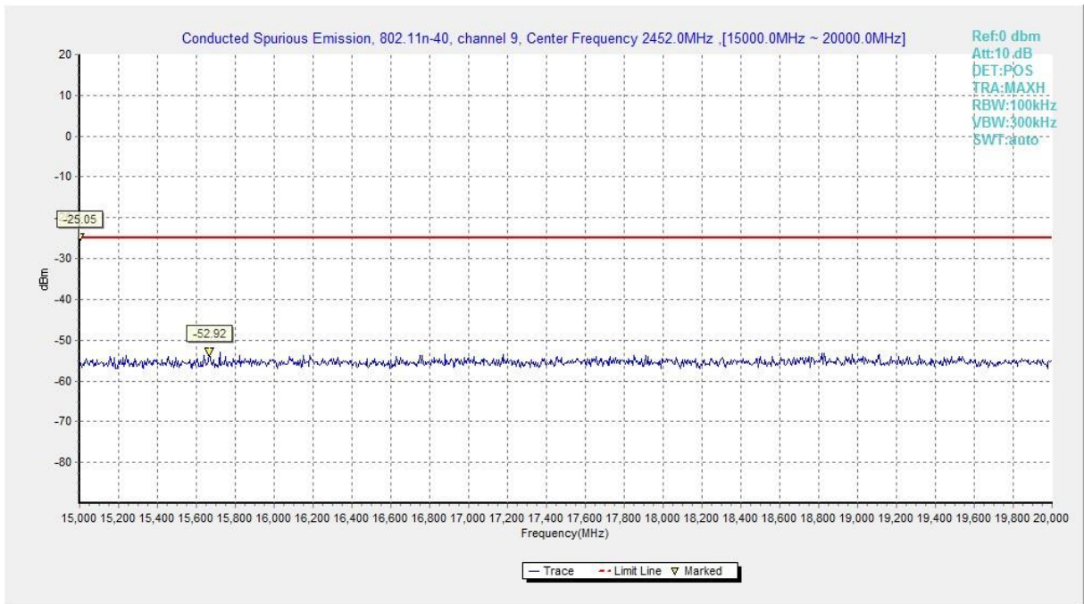
Fig.A.6.1.94 Transmitter Spurious Emission - Conducted (802.11n-HT40, Ch9, 15 GHz-20 GHz)
