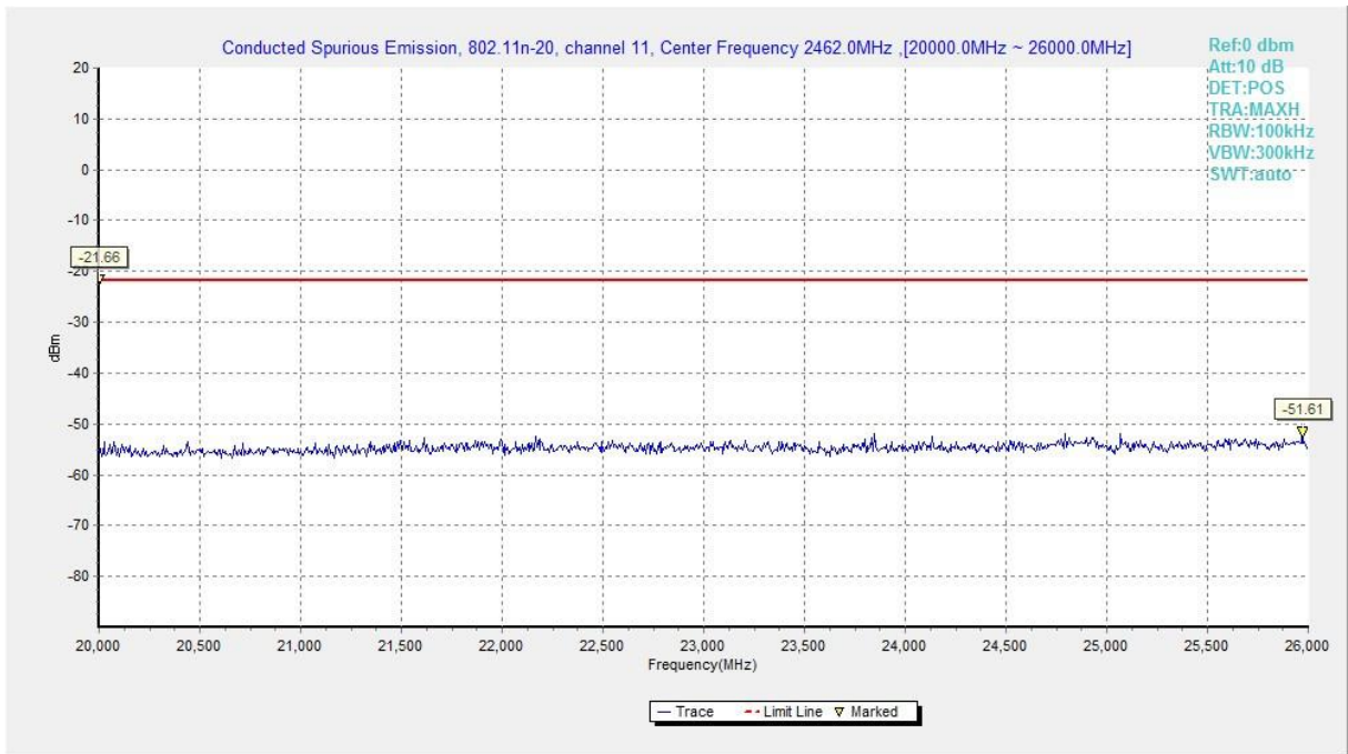
Fig.A.6.1.71 Transmitter Spurious Emission - Conducted (802.11n-HT20, Ch11, 20 GHz-26 GHz)
