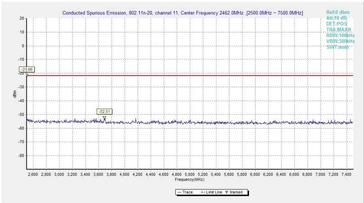
Fig.A.6.1.67 Transmitter Spurious Emission - Conducted (802.11n-HT20, Ch11, 2.5 GHz-7.5 GHz)
