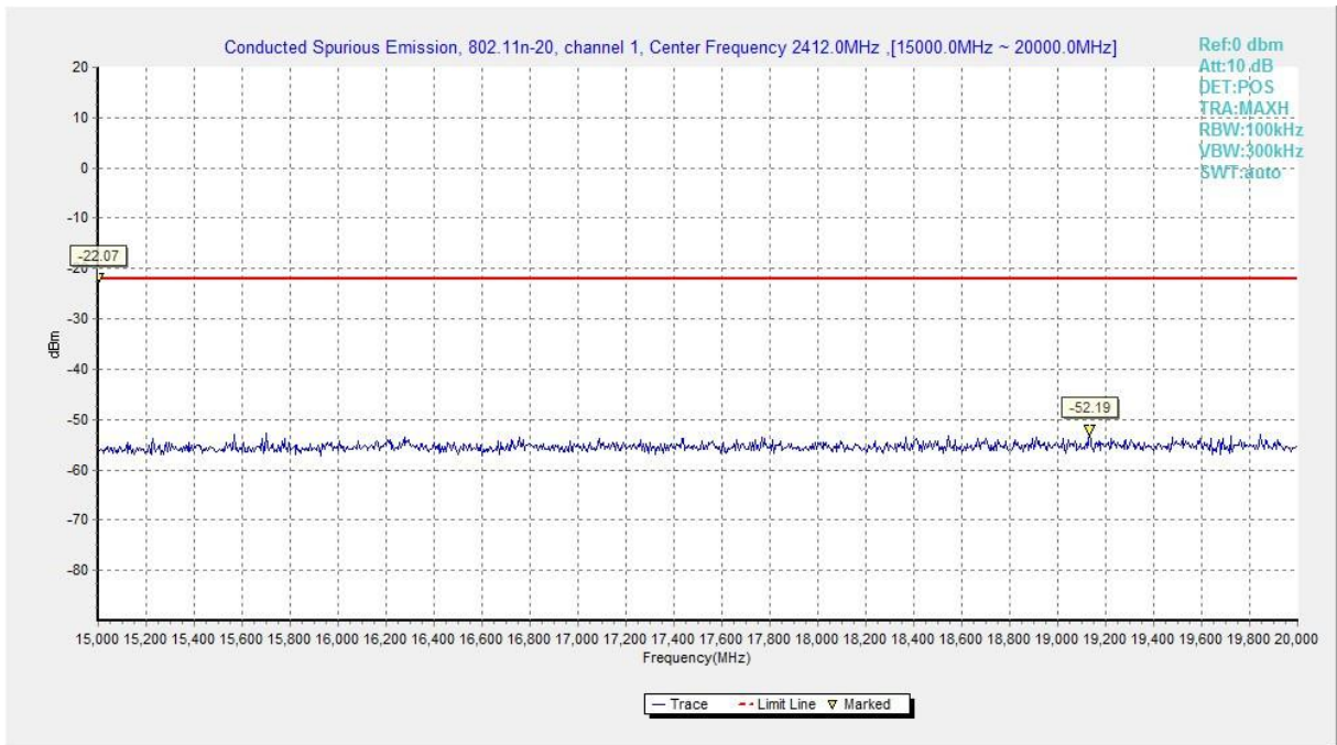
Fig.A.6.1.54 Transmitter Spurious Emission - Conducted (802.11n-HT20, Ch1, 15 GHz-20 GHz)
