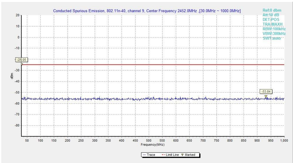
Fig.A.6.1.89 Transmitter Spurious Emission - Conducted (802.11n-HT40, Ch9, 30 MHz-1 GHz)
