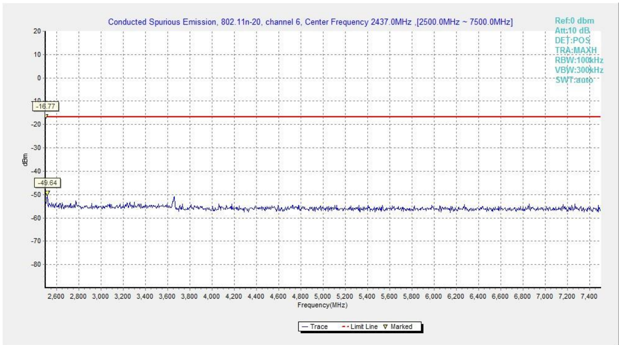
Fig.A.6.1.59 Transmitter Spurious Emission - Conducted (802.11n-HT20, Ch6, 2.5 GHz-7.5 GHz)
