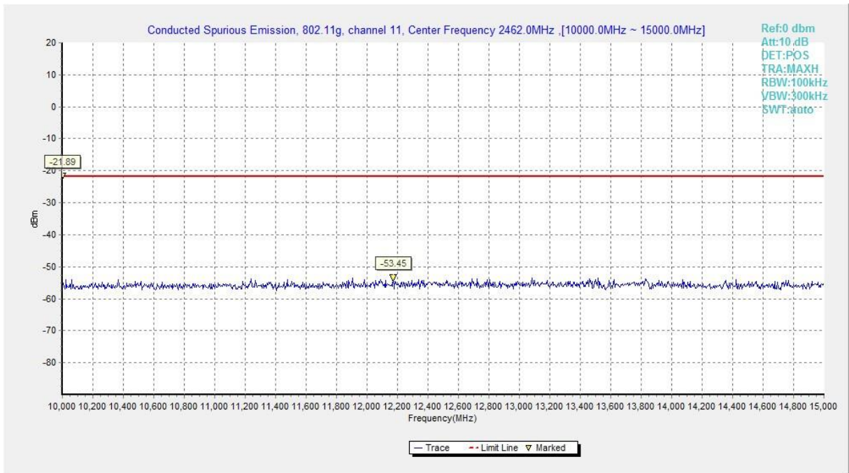
Fig.A.6.1.45 Transmitter Spurious Emission - Conducted (802.11g, Ch11, 10 GHz-15 GHz)
