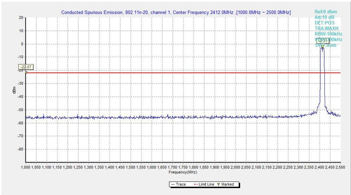
Fig.A.6.1.50 Transmitter Spurious Emission - Conducted (802.11n-HT20, Ch1, 1 GHz-2.5 GHz)
