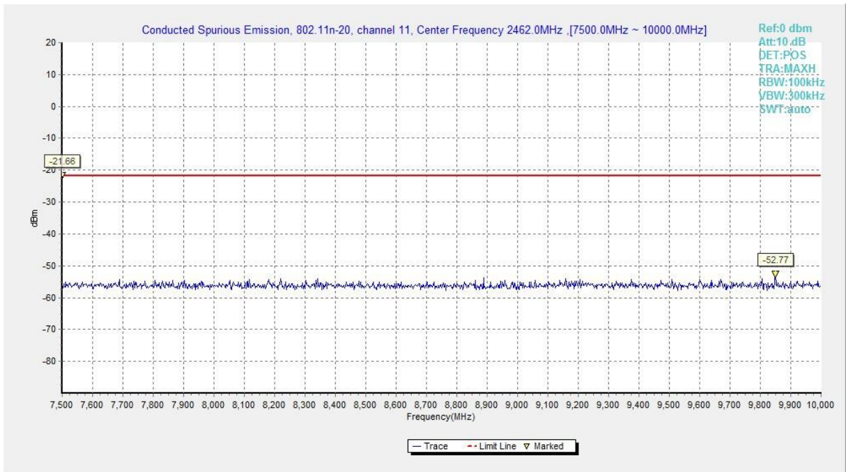
Fig.A.6.1.68 Transmitter Spurious Emission - Conducted (802.11n-HT20, Ch11, 7.5 GHz-10 GHz)
