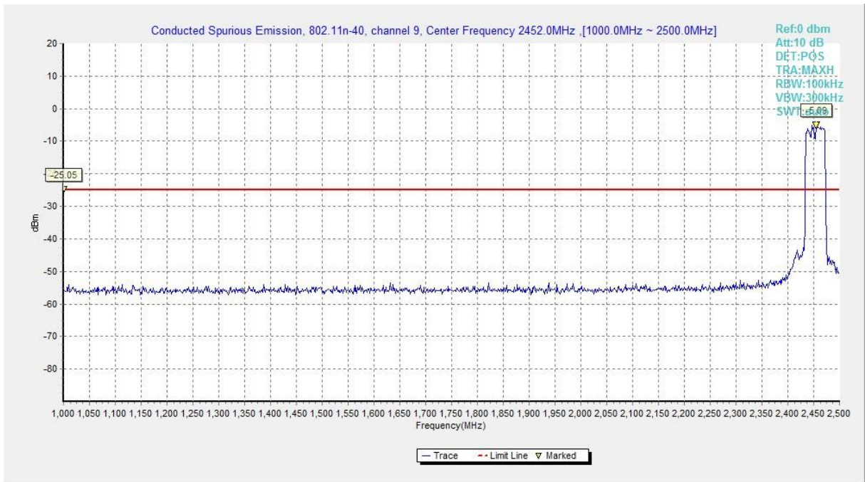
Fig.A.6.1.90 Transmitter Spurious Emission - Conducted (802.11n-HT40, Ch9, 1 GHz-2.5 GHz)
