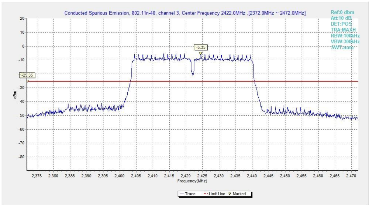
Fig.A.6.1.72 Transmitter Spurious Emission - Conducted (802.11n-HT40, Ch3, Center Frequency)
