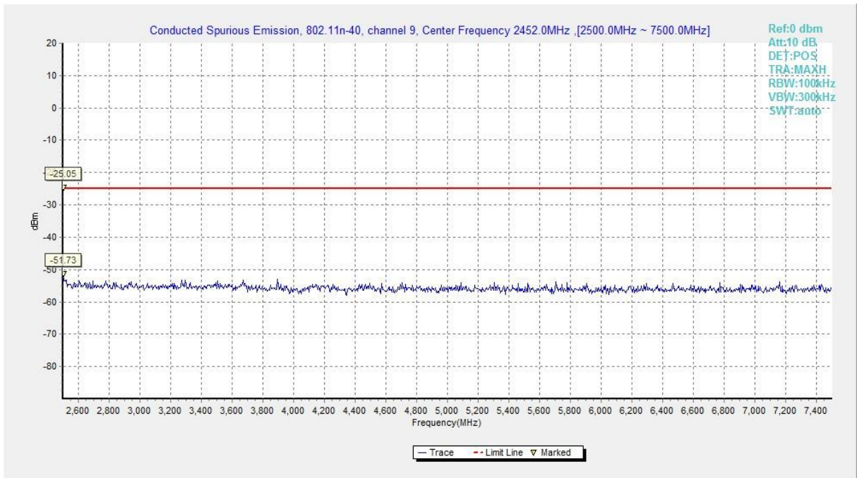
Fig.A.6.1.91 Transmitter Spurious Emission - Conducted (802.11n-HT40, Ch9, 2.5 GHz-7.5 GHz)
