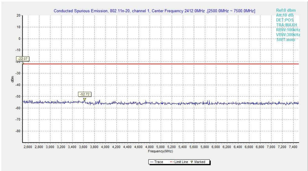
Fig.A.6.1.51 Transmitter Spurious Emission - Conducted (802.11n-HT20, Ch1, 2.5 GHz-7.5 GHz)
