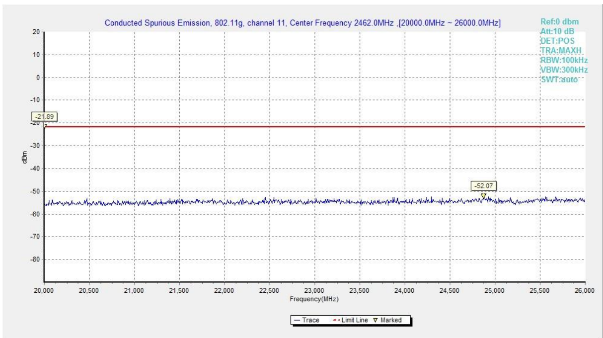
Fig.A.6.1.47 Transmitter Spurious Emission - Conducted (802.11g, Ch11, 20 GHz-26 GHz)
