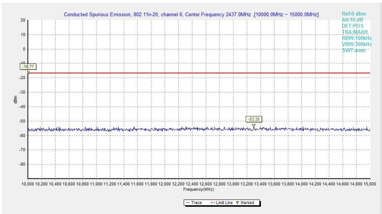
Fig.A.6.1.61 Transmitter Spurious Emission - Conducted (802.11n-HT20, Ch6, 10 GHz-15 GHz)
