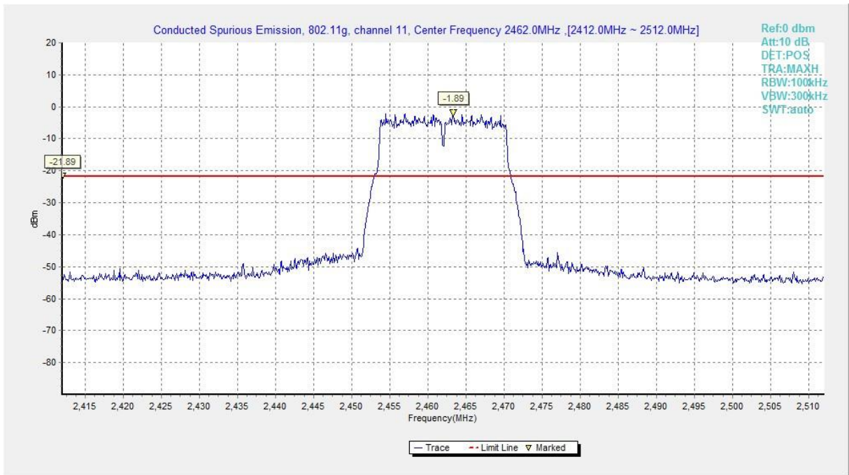
Fig.A.6.1.40 Transmitter Spurious Emission - Conducted (802.11g, Ch11, Center Frequency)
