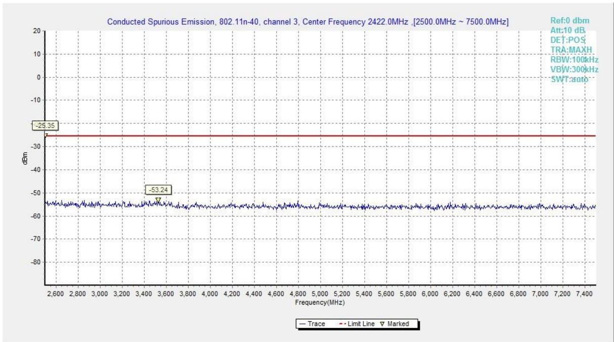
Fig.A.6.1.75 Transmitter Spurious Emission - Conducted (802.11n-HT40, Ch3, 2.5 GHz-7.5 GHz)
