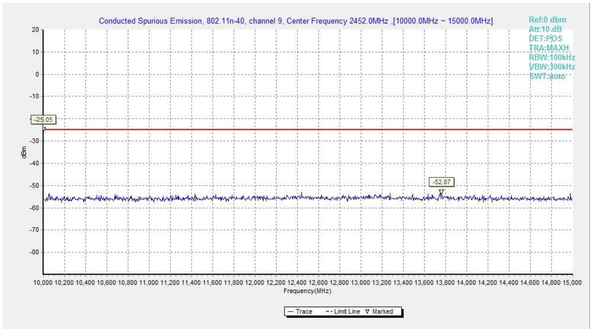
Fig.A.6.1.93 Transmitter Spurious Emission - Conducted (802.11n-HT40, Ch9, 10 GHz-15 GHz)
