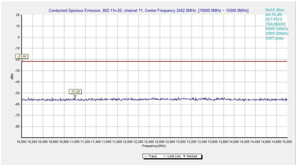
Fig.A.6.1.69 Transmitter Spurious Emission - Conducted (802.11n-HT20, Ch11, 10 GHz-15 GHz)
