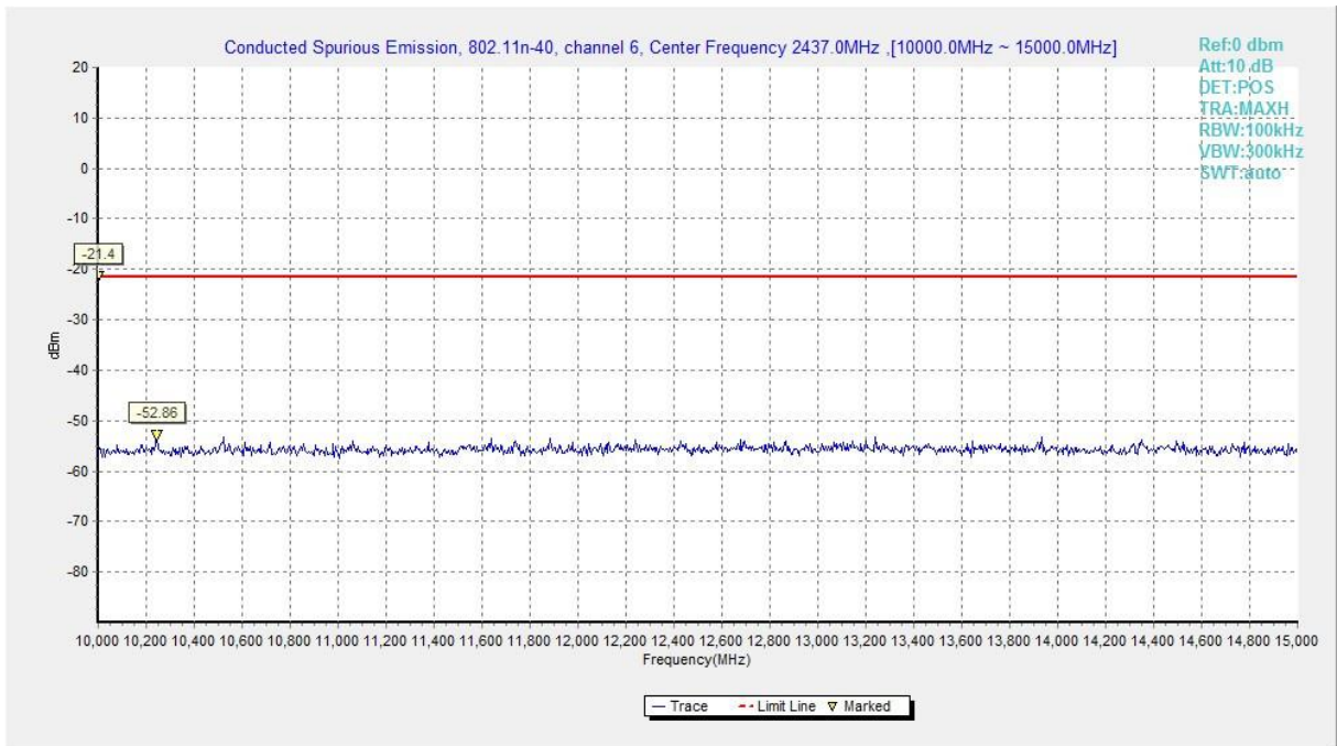
Fig.A.6.1.85 Transmitter Spurious Emission - Conducted (802.11n-HT40, Ch6, 10 GHz-15 GHz)
