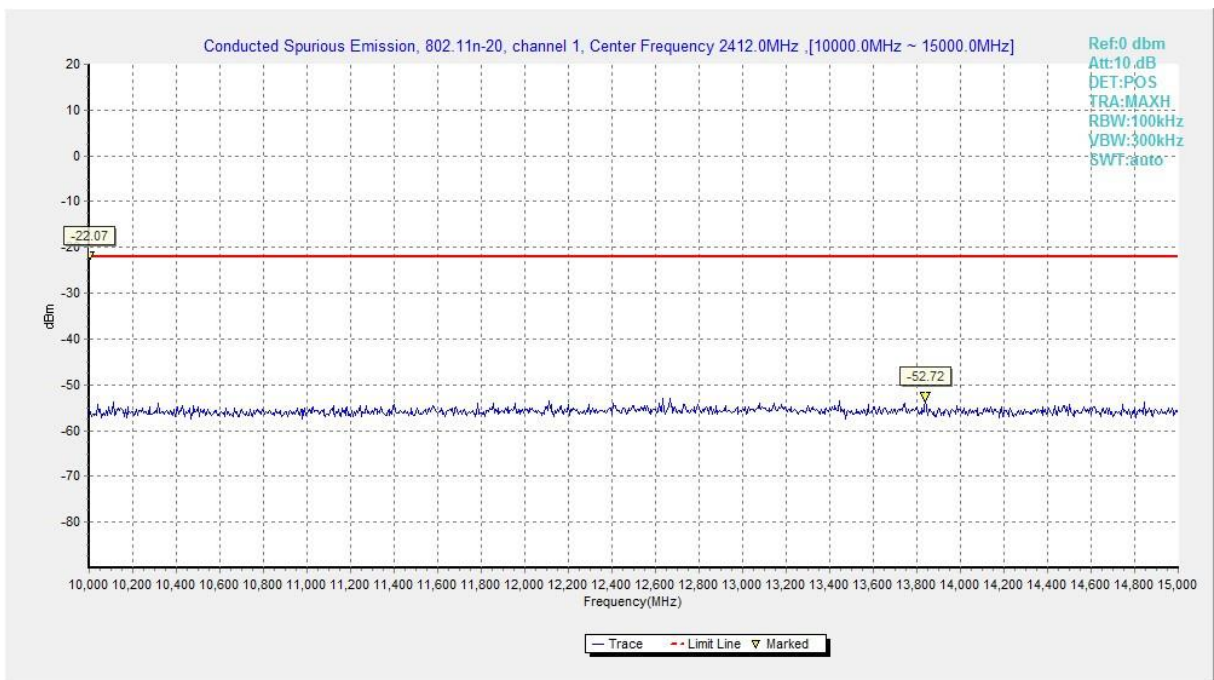
Fig.A.6.1.53 Transmitter Spurious Emission - Conducted (802.11n-HT20, Ch1, 10 GHz-15 GHz)
