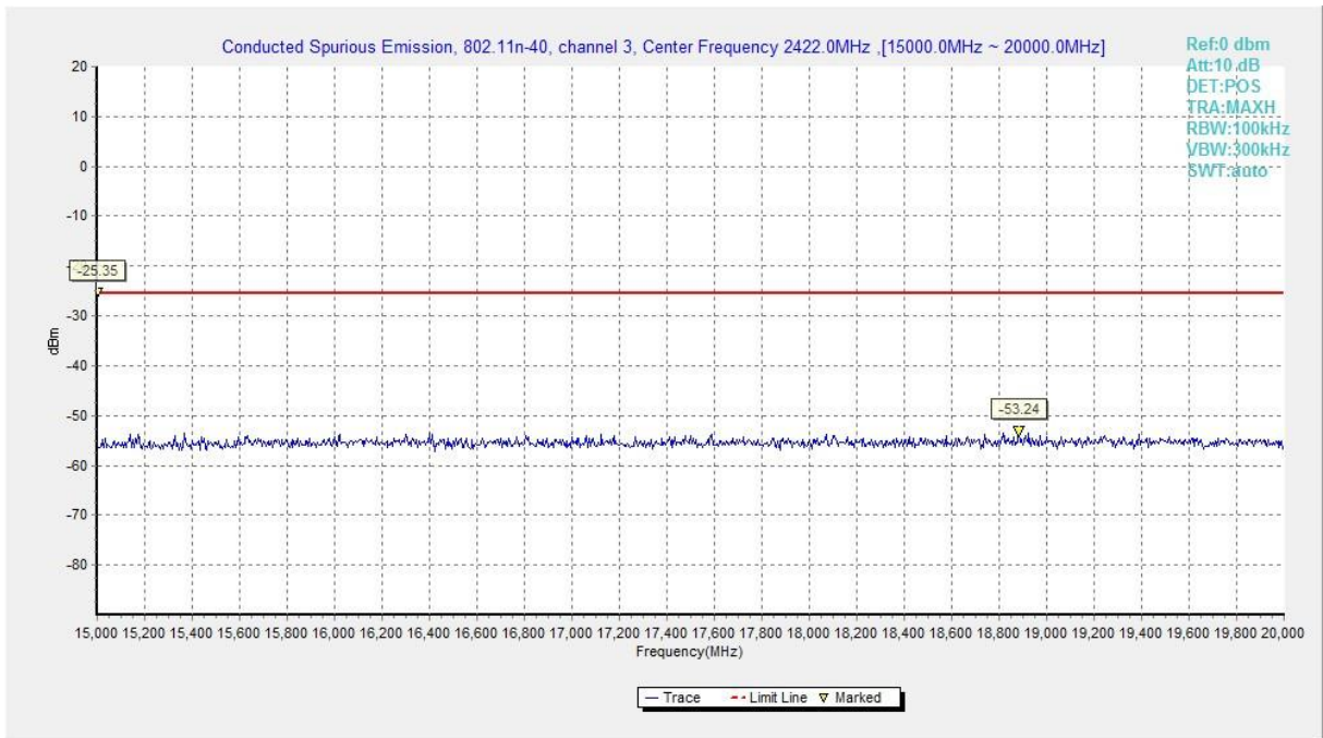
Fig.A.6.1.78 Transmitter Spurious Emission - Conducted (802.11n-HT40, Ch3, 15 GHz-20 GHz)
