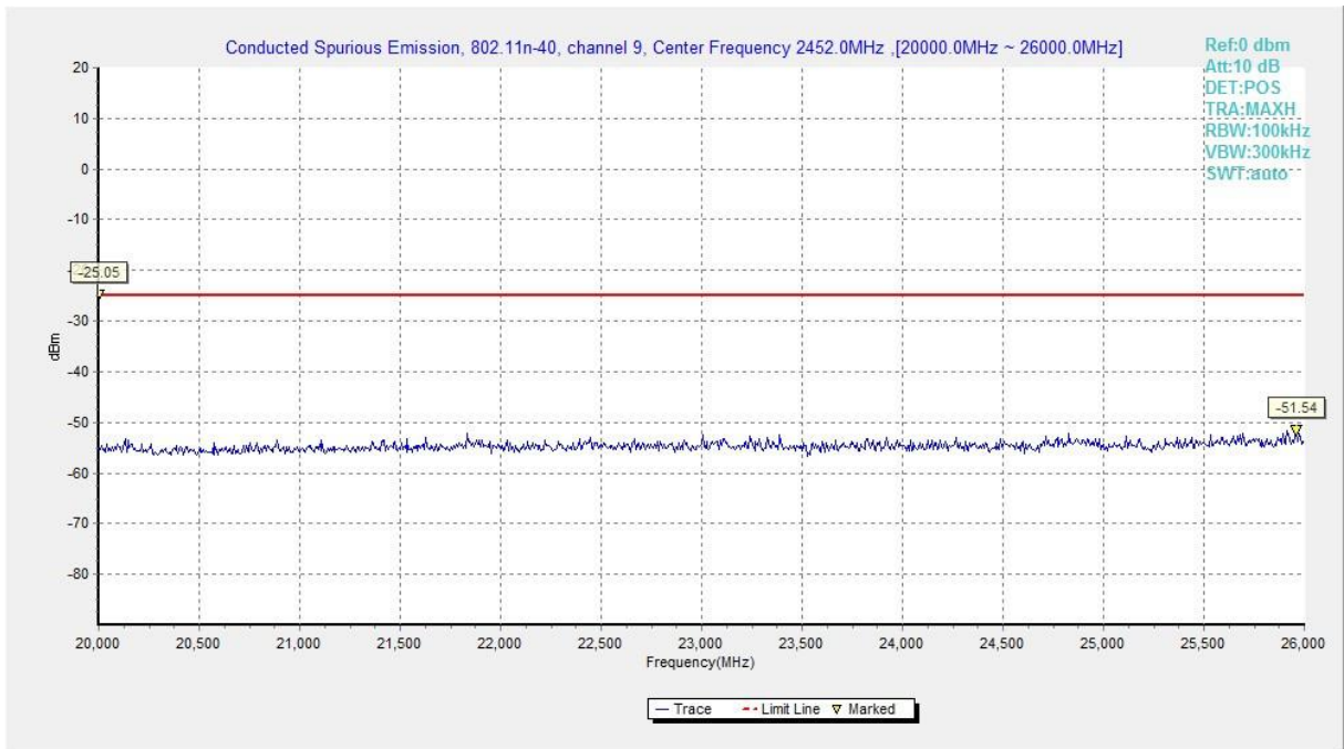
Fig.A.6.1.95 Transmitter Spurious Emission - Conducted (802.11n-HT40, Ch9, 20 GHz-26 GHz)
