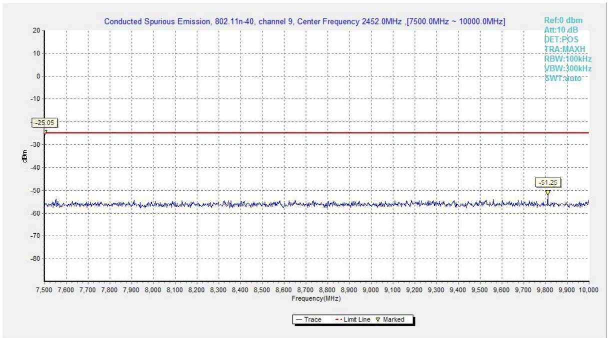
Fig.A.6.1.92 Transmitter Spurious Emission - Conducted (802.11n-HT40, Ch9, 7.5 GHz-10 GHz)
