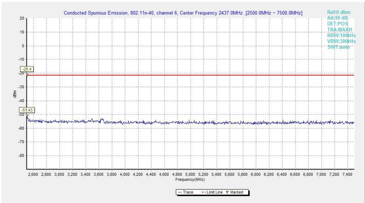
Fig.A.6.1.83 Transmitter Spurious Emission - Conducted (802.11n-HT40, Ch6, 2.5 GHz-7.5 GHz)
