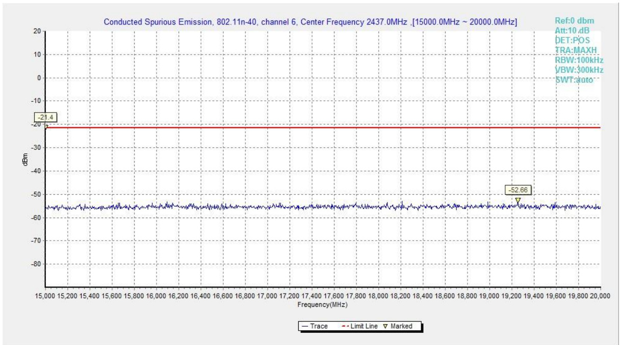
Fig.A.6.1.86 Transmitter Spurious Emission - Conducted (802.11n-HT40, Ch6, 15 GHz-20 GHz)
