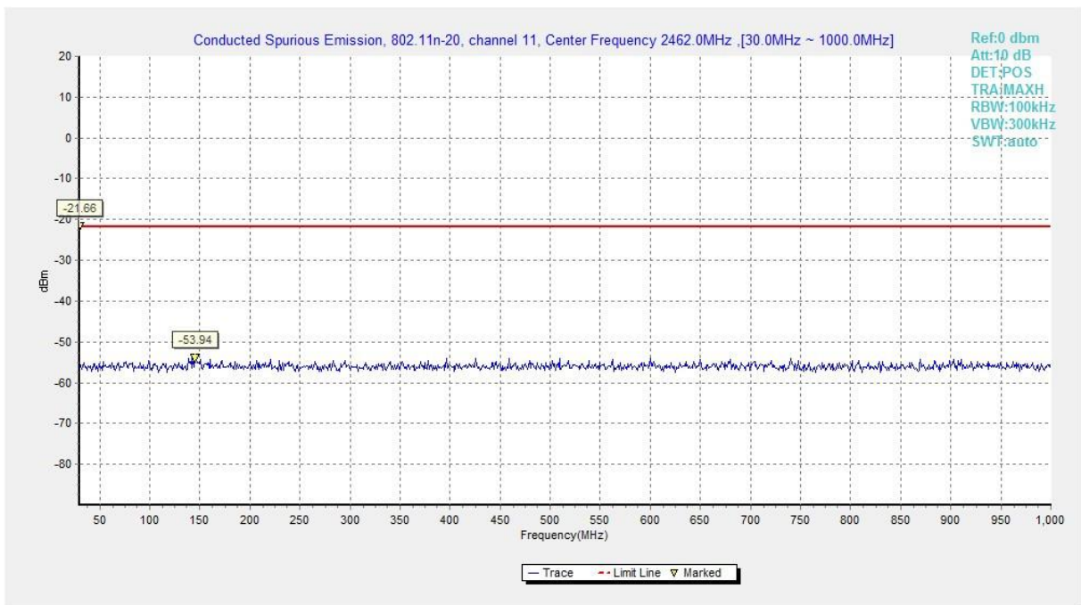
Fig.A.6.1.65 Transmitter Spurious Emission - Conducted (802.11n-HT20, Ch11, 30 MHz-1 GHz)
