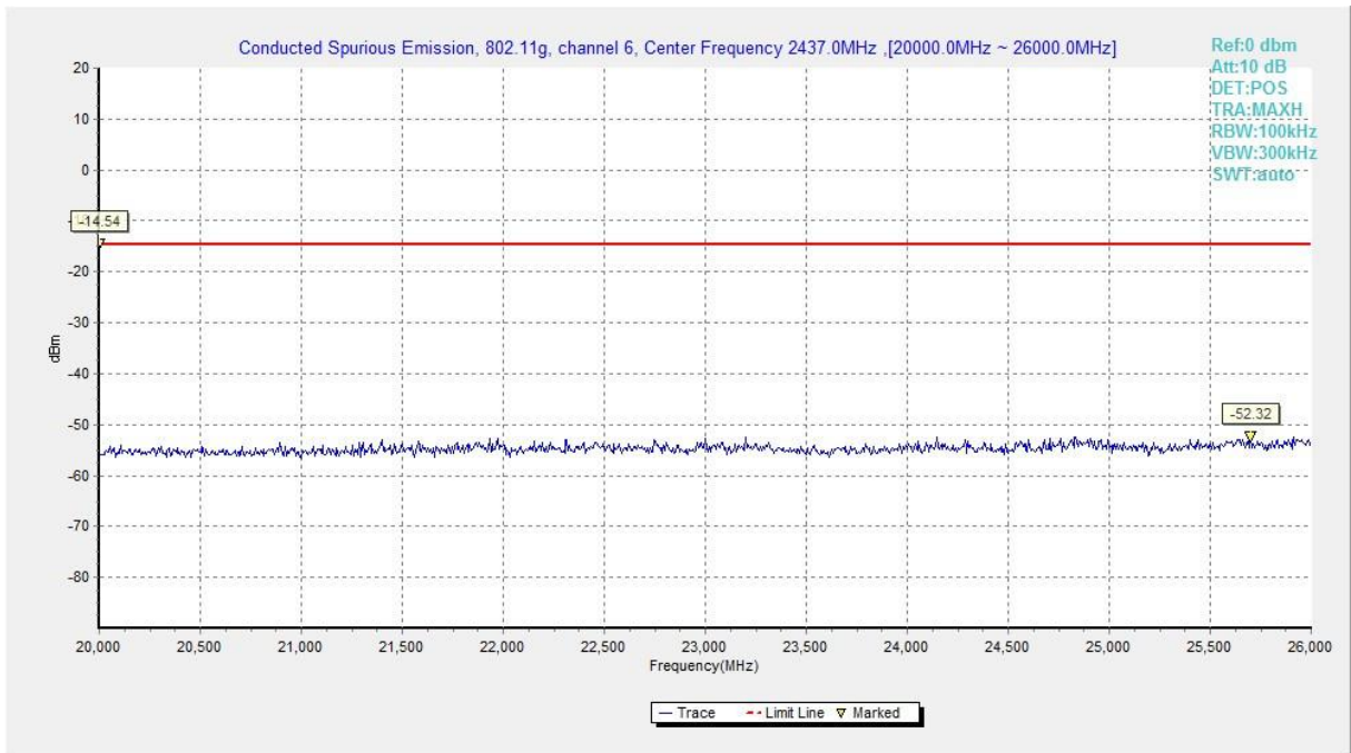
Fig.A.6.1.39 Transmitter Spurious Emission - Conducted (802.11g, Ch6, 20 GHz-26 GHz)
