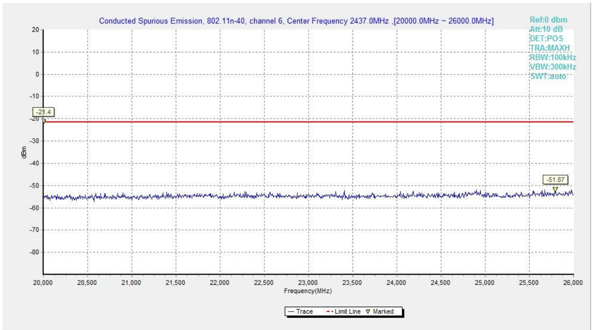
Fig.A.6.1.87 Transmitter Spurious Emission - Conducted (802.11n-HT40, Ch6, 20 GHz-26 GHz)
