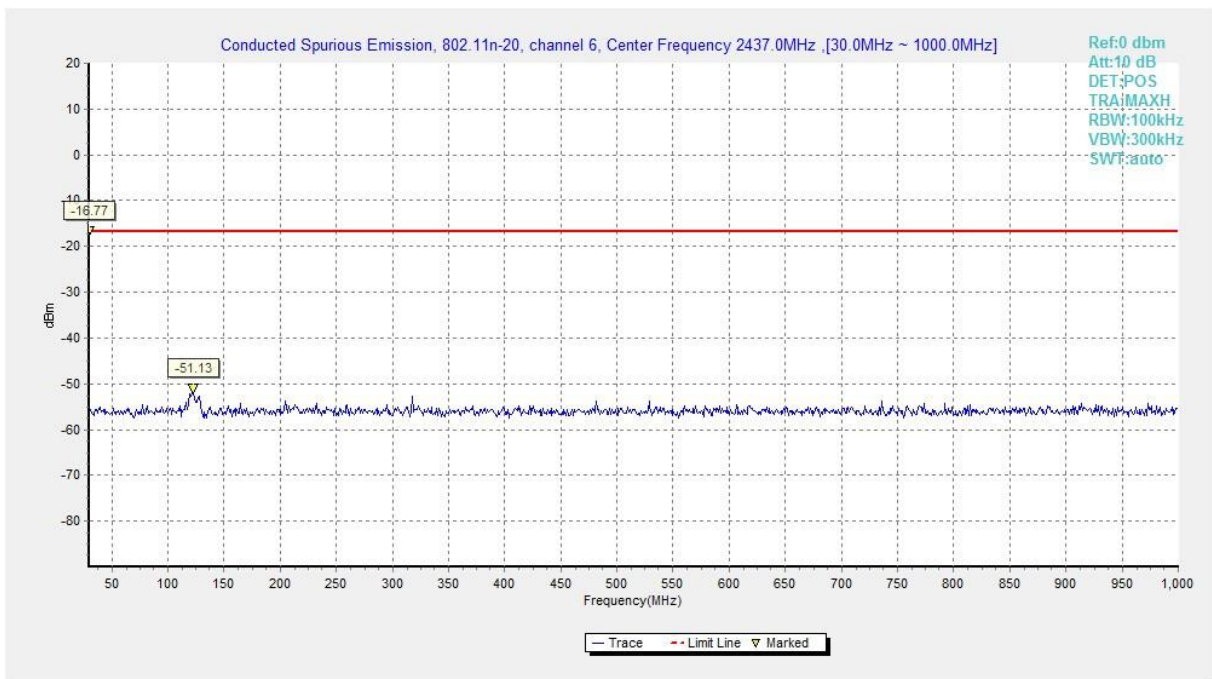
Fig.A.6.1.57 Transmitter Spurious Emission - Conducted (802.11n-HT20, Ch6, 30 MHz-1 GHz)
