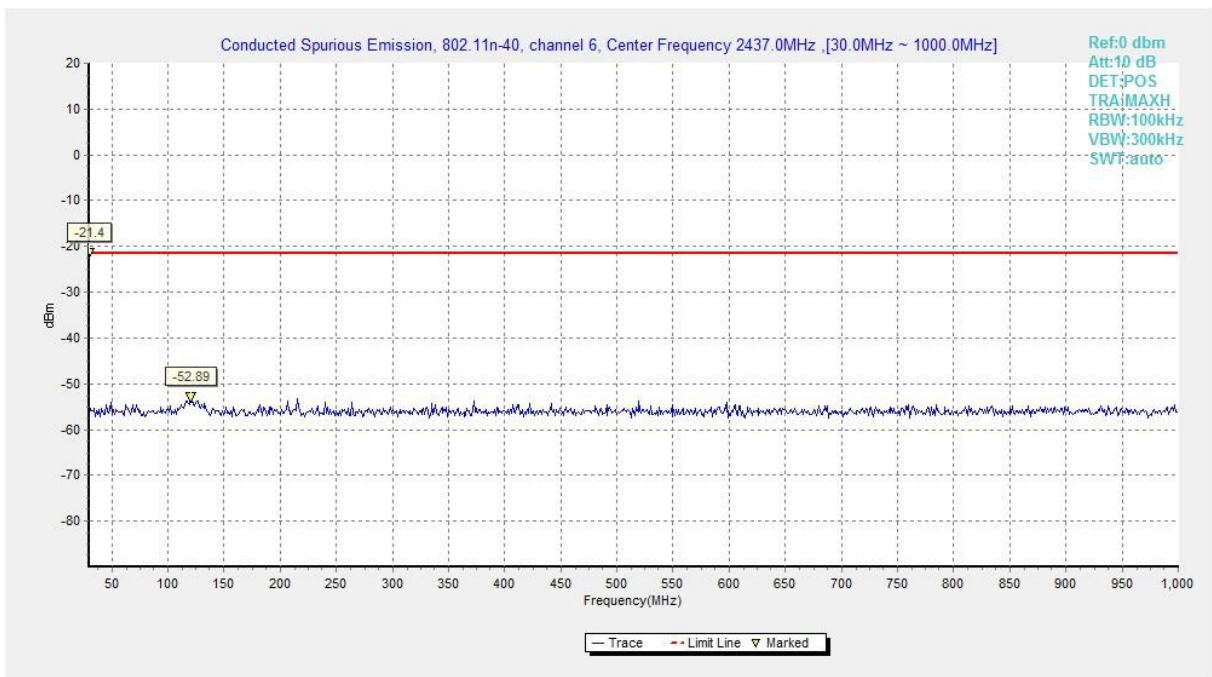
Fig.A.6.1.81 Transmitter Spurious Emission - Conducted (802.11n-HT40, Ch6, 30 MHz-1 GHz)
