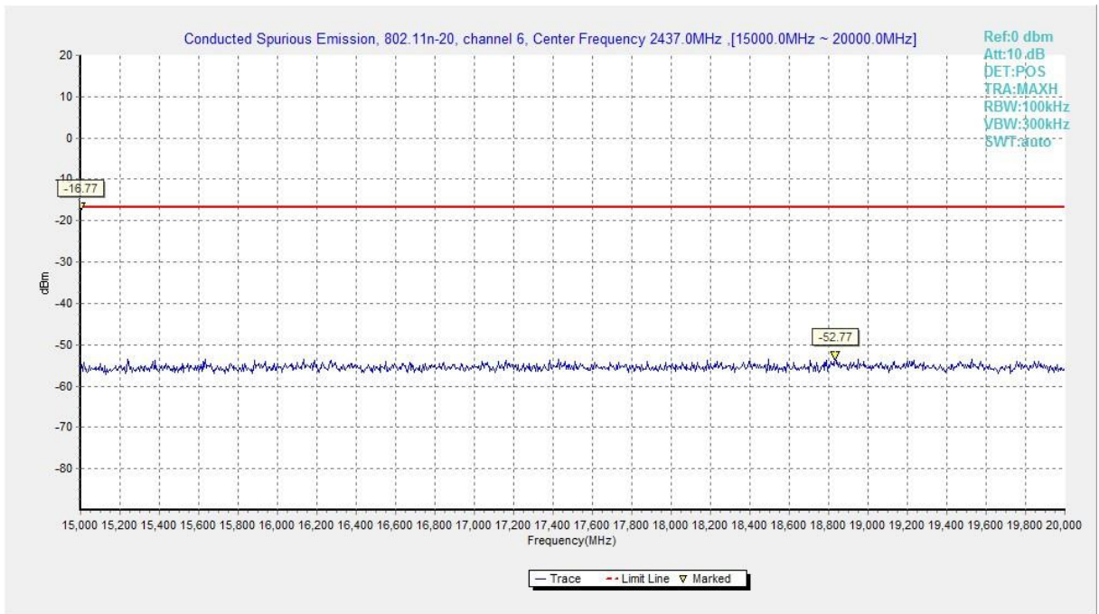
Fig.A.6.1.62 Transmitter Spurious Emission - Conducted (802.11n-HT20, Ch6, 15 GHz-20 GHz)
