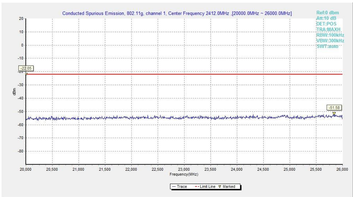
Fig.A.6.1.31 Transmitter Spurious Emission - Conducted (802.11g, Ch1, 20 GHz-26 GHz)
