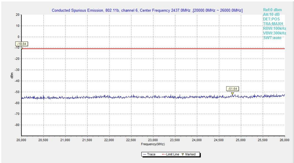
Fig.A.6.1.15 Transmitter Spurious Emission - Conducted (802.11b, Ch6, 20 GHz-26 GHz)
