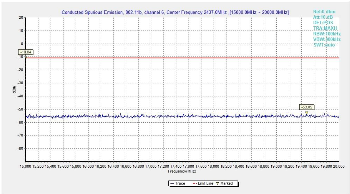
Fig.A.6.1.14 Transmitter Spurious Emission - Conducted (802.11b, Ch6, 15 GHz-20 GHz)
