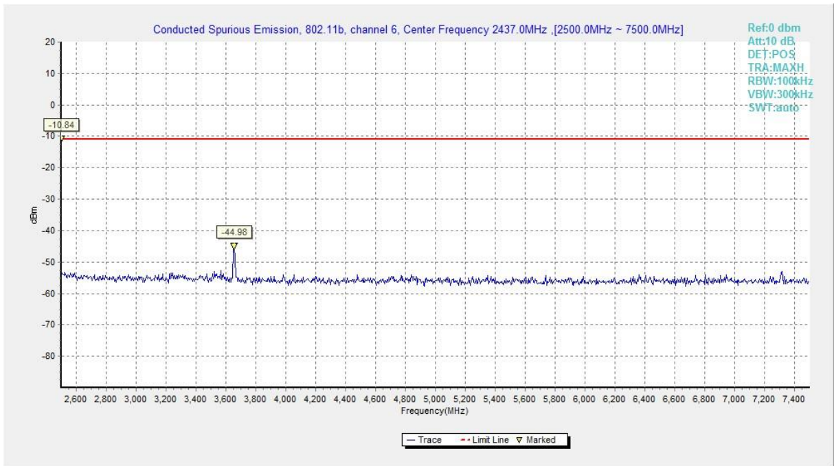
Fig.A.6.1.11 Transmitter Spurious Emission - Conducted (802.11b, Ch6, 2.5 GHz-7.5 GHz)
