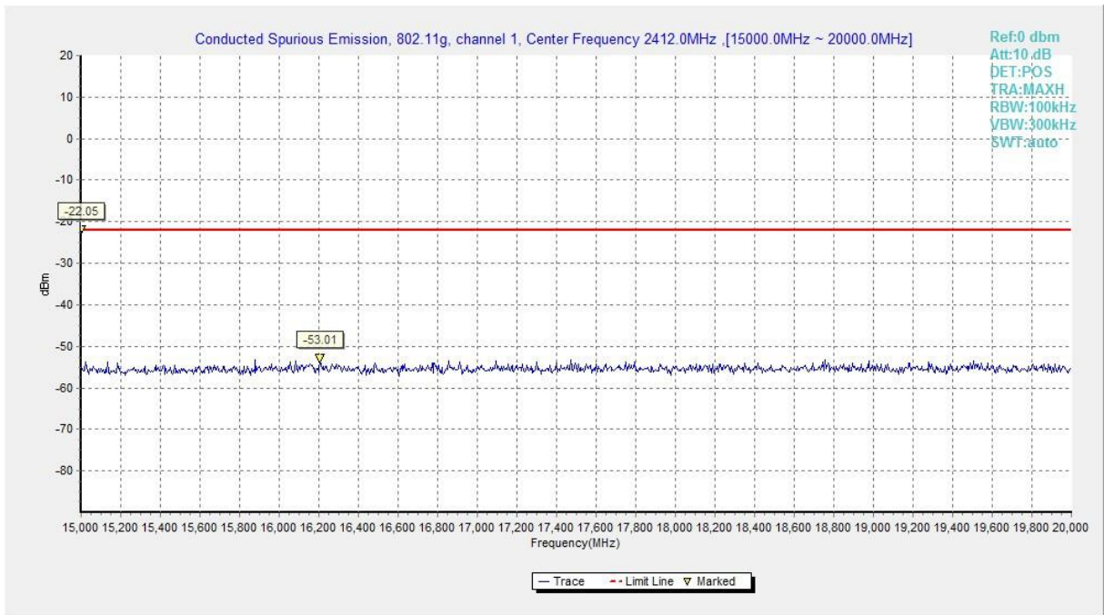
Fig.A.6.1.30 Transmitter Spurious Emission - Conducted (802.11g, Ch1, 15 GHz-20 GHz)
