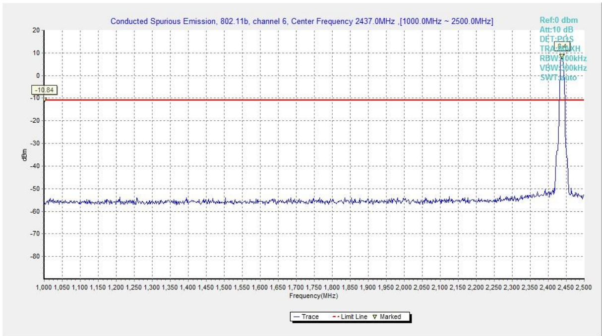
Fig.A.6.1.10 Transmitter Spurious Emission - Conducted (802.11b, Ch6, 1 GHz-2.5 GHz)
