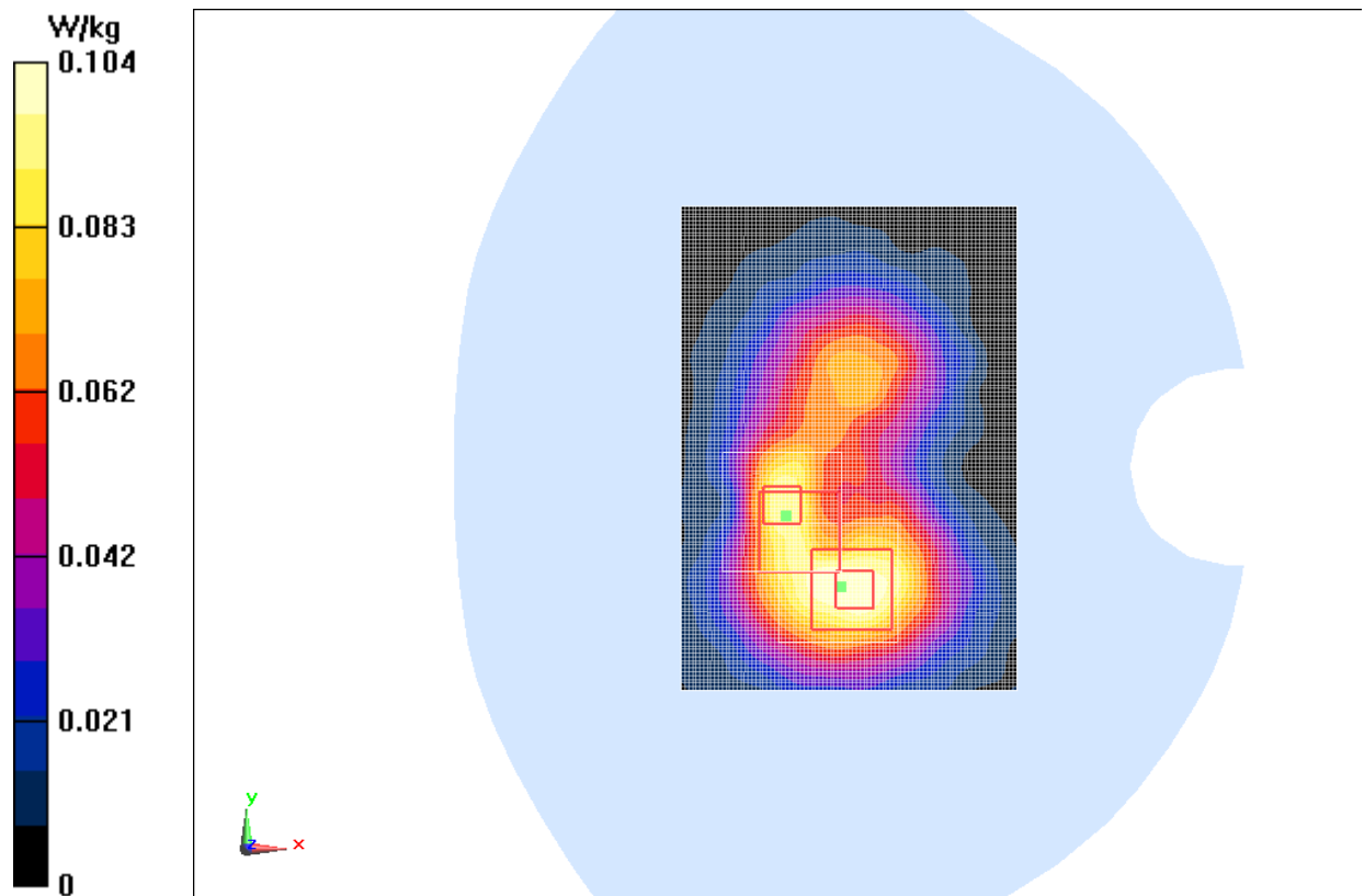
Fig.6 2450 MHz CH6
