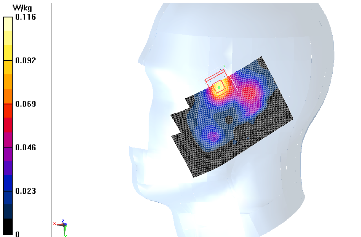
Fig.5 2450 MHz CH6
