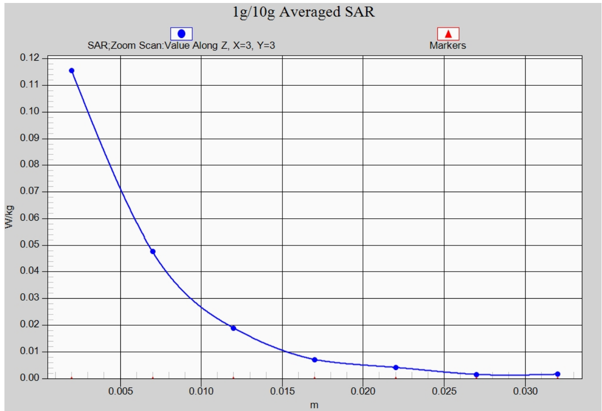
Fig. 5-1 Z-Scan at power reference point (2450 MHz CH6)
