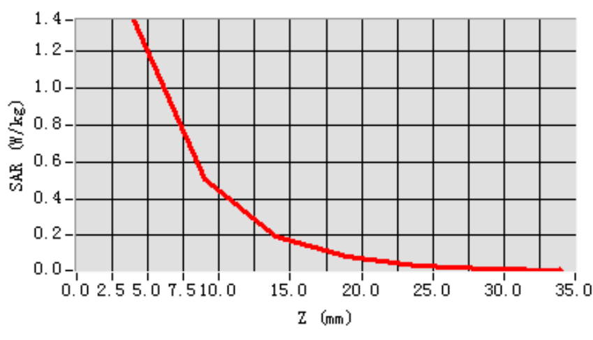
SAR, Z Axis Scan (X = -2, Y = -14)
