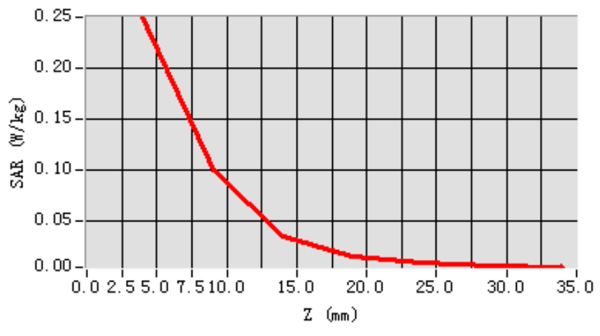
SAR, Z Axis Scan (X = 0, Y = 18)
