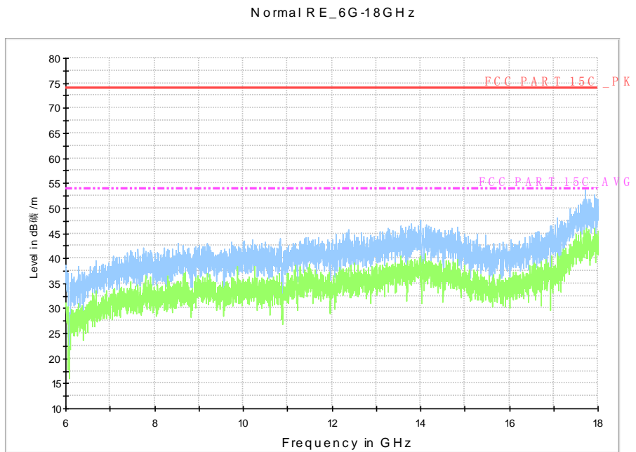
Fig. 60 Radiated Spurious Emission (802.11a, Ch157, 6 GHz-18 GHz)
