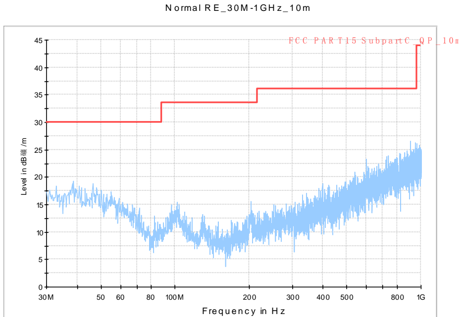
Fig. 78 Radiated Spurious Emission (802.11n-HT40, Ch159, 30 MHz-1 GHz)
