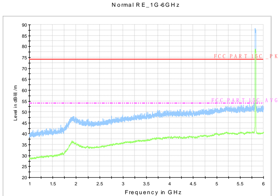
Fig. 72 Radiated Spurious Emission (802.11n-HT20, Ch165, 1 GHz-6 GHz)
