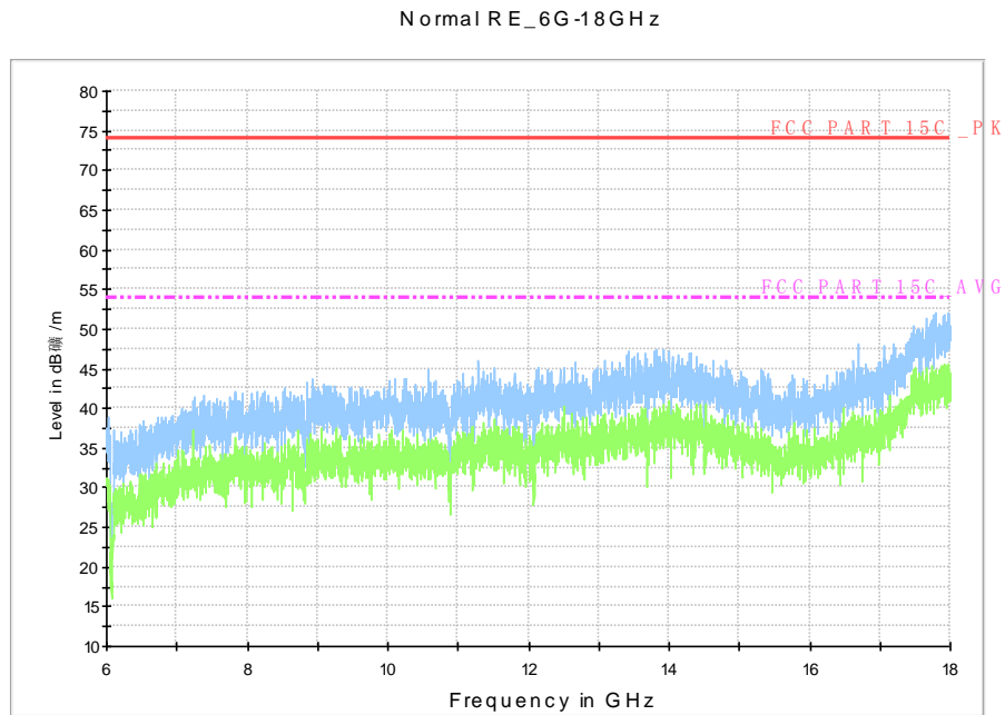
Fig. 57 Radiated Spurious Emission (802.11a, Ch149, 6 GHz-18 GHz)
