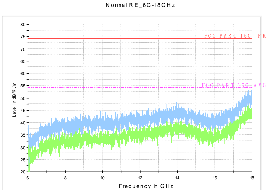
Fig. 84 Radiated Spurious Emission (802.11a, 6 GHz-18 GHz)
