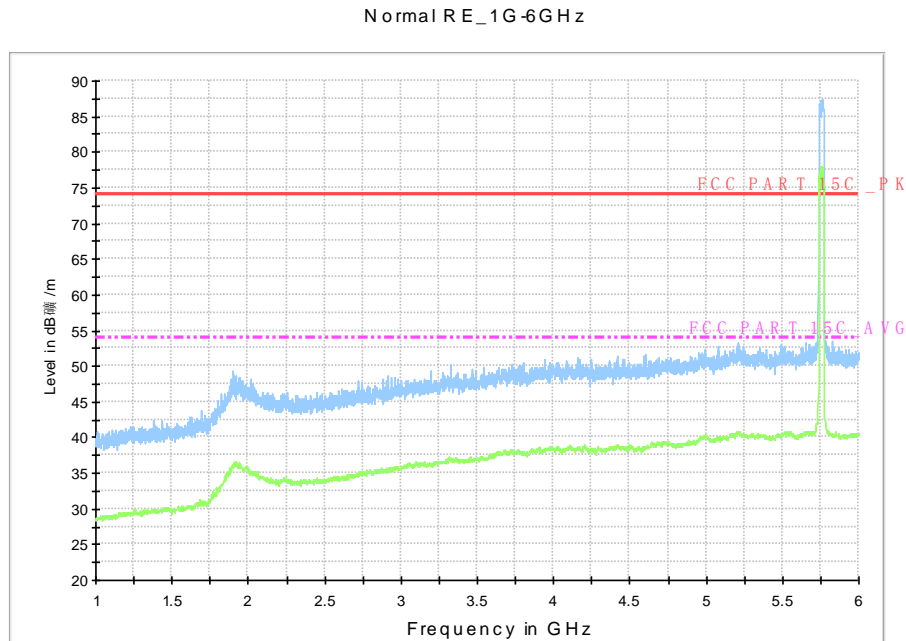
Fig. 76 Radiated Spurious Emission (802.11n-HT40, Ch151, 1 GHz-6 GHz)
