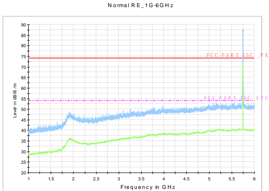
Fig. 56 Radiated Spurious Emission (802.11a, Ch149, 1 GHz-6 GHz)
