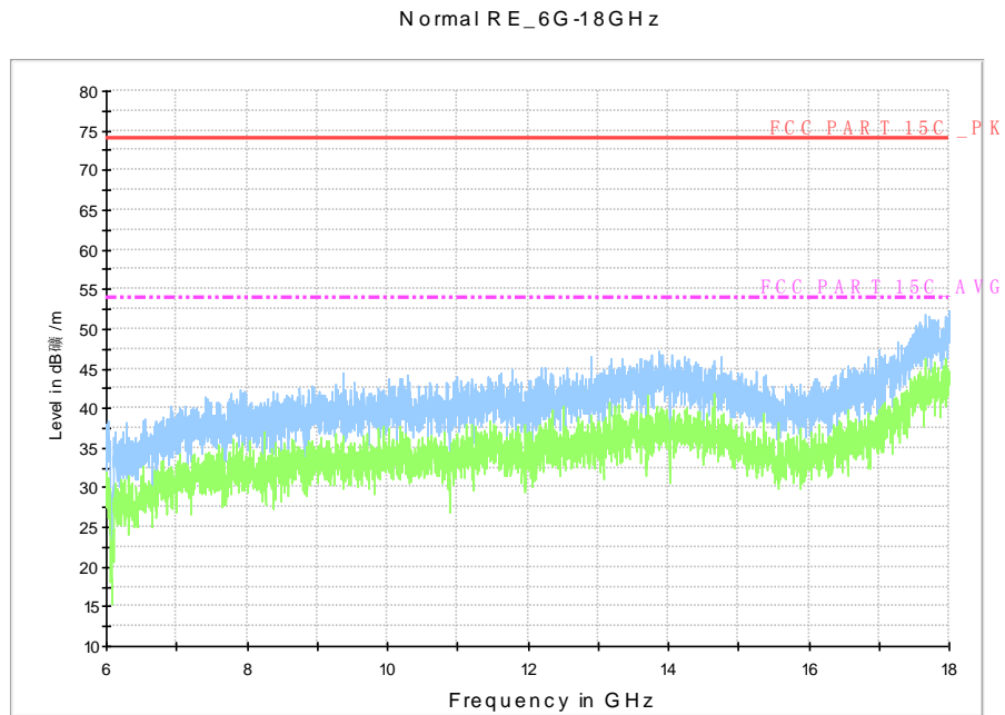
Fig. 67 Radiated Spurious Emission (802.11n-HT20, Ch149, 6 GHz-18 GHz)
