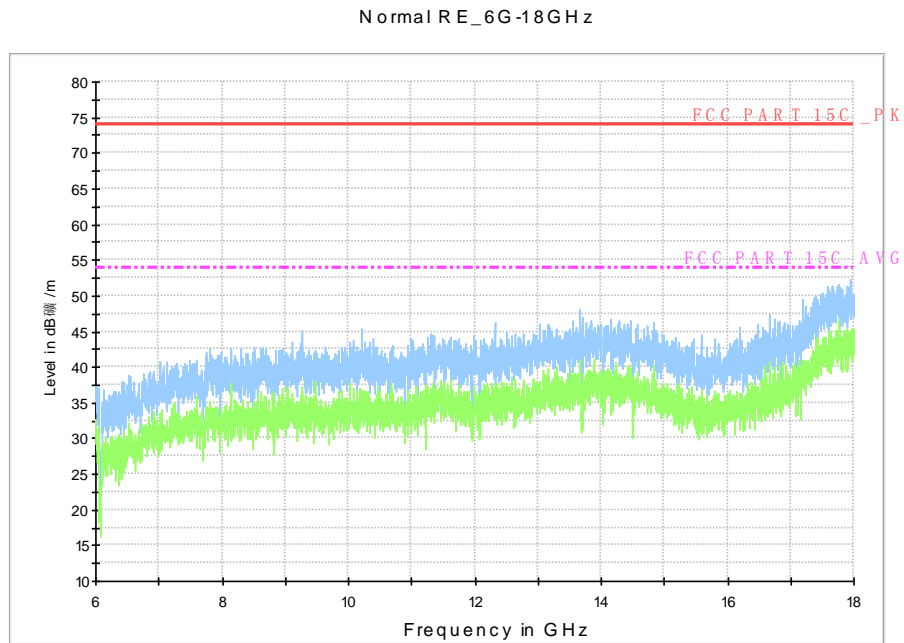
Fig. 63 Radiated Spurious Emission (802.11a, Ch165, 6 GHz-18 GHz)
