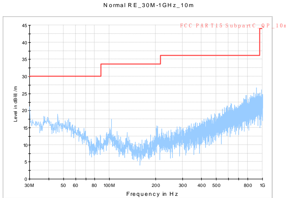
Fig. 71 Radiated Spurious Emission (802.11n-HT20, Ch165, 30 MHz-1 GHz)
