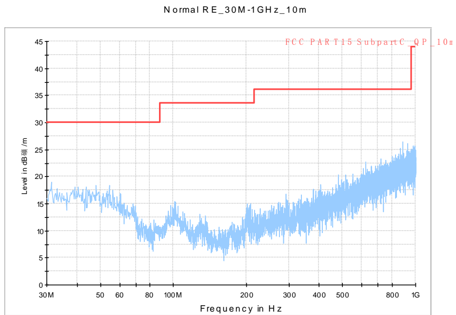
Fig. 61 Radiated Spurious Emission (802.11a, Ch165, 30 MHz-1 GHz)
