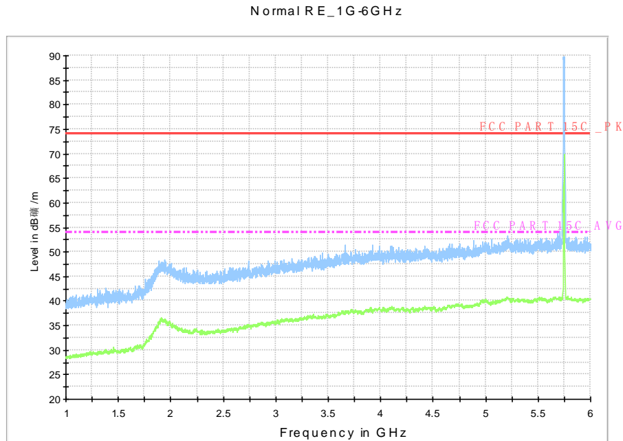
Fig. 66 Radiated Spurious Emission (802.11n-HT20, Ch149, 1 GHz-6 GHz)
