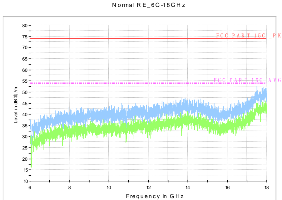
Fig. 80 Radiated Spurious Emission (802.11n-HT40, Ch159, 6 GHz-18 GHz)
