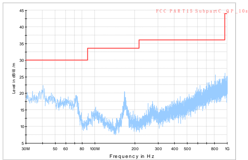
Normal RE_30M-1GHz_10m
