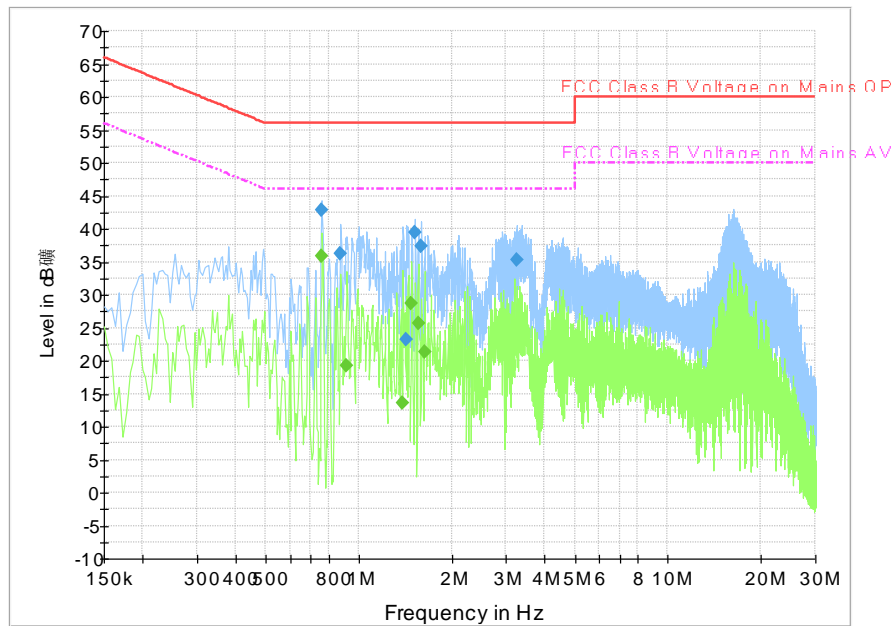
Fig. 88 AC Powerline Conducted Emission-802.11a mode
