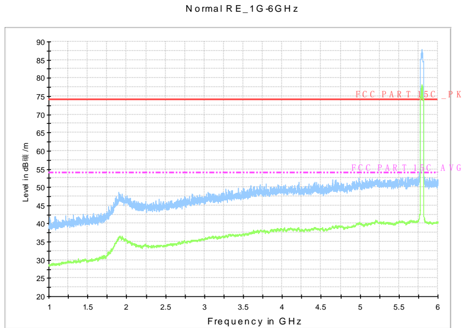
Fig. 79 Radiated Spurious Emission (802.11n-HT40, Ch159, 1 GHz-6 GHz)
