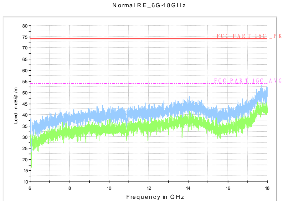
Fig. 73 Radiated Spurious Emission (802.11n-HT20, Ch165, 6 GHz-18 GHz)
