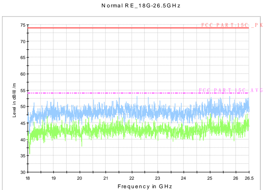
Fig. 85 Radiated Spurious Emission (802.11a, 18 GHz-26.5 GHz)
