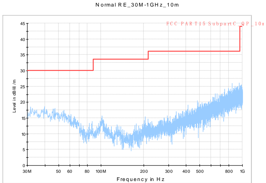
Fig. 65 Radiated Spurious Emission (802.11n-HT20, Ch149, 30 MHz-1 GHz)
