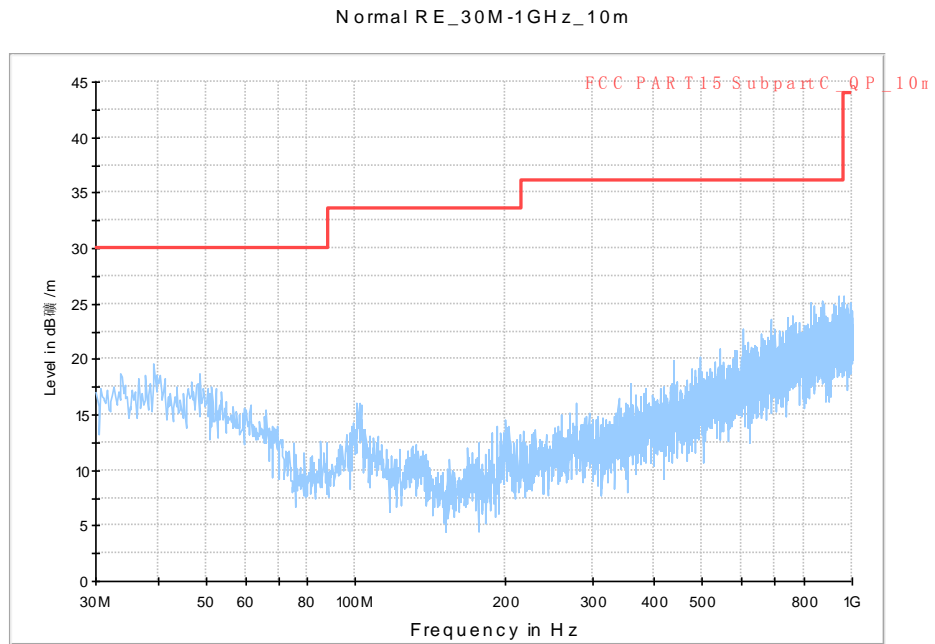
Fig. 55 Radiated Spurious Emission (802.11a, Ch149, 30 MHz-1 GHz)
