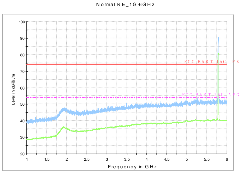
Fig. 69 Radiated Spurious Emission (802.11n-HT20, Ch157, 1 GHz-6 GHz)
