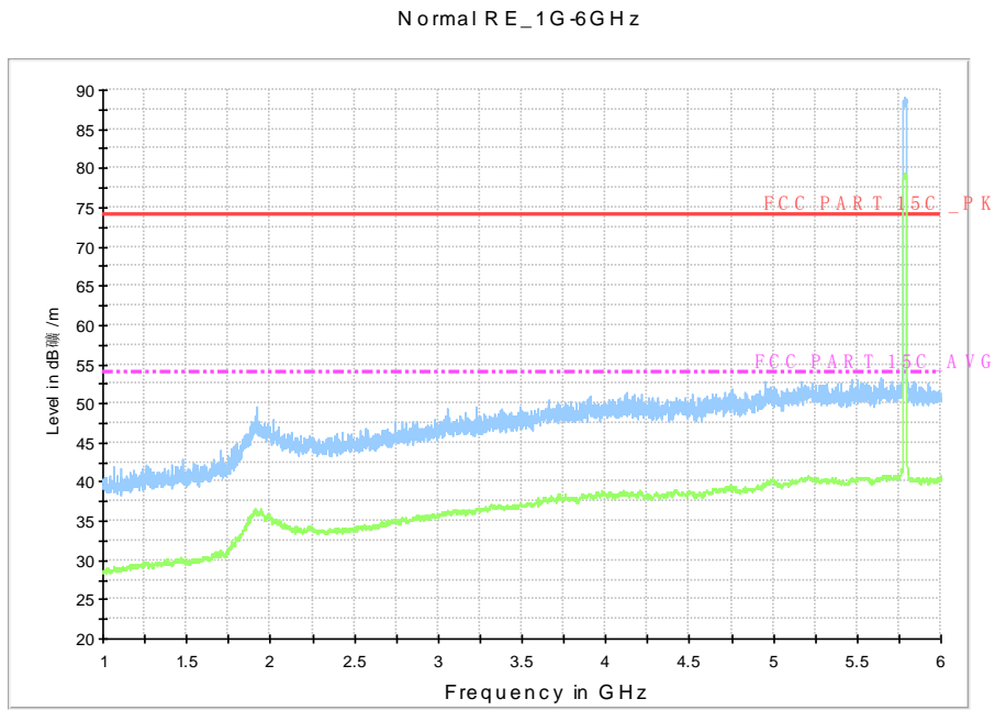
Fig. 59 Radiated Spurious Emission (802.11a, Ch157, 1 GHz-6 GHz)
