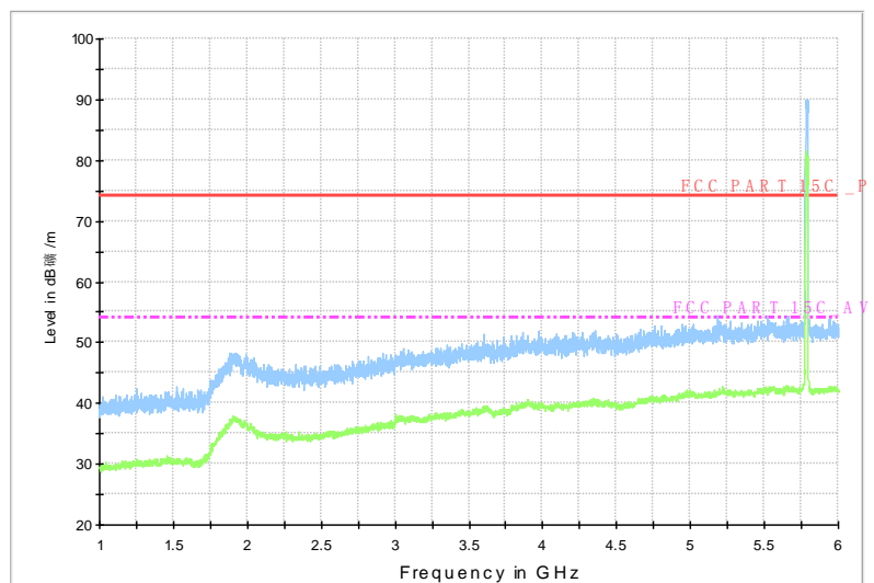
Normal RE_1G-6GHz
