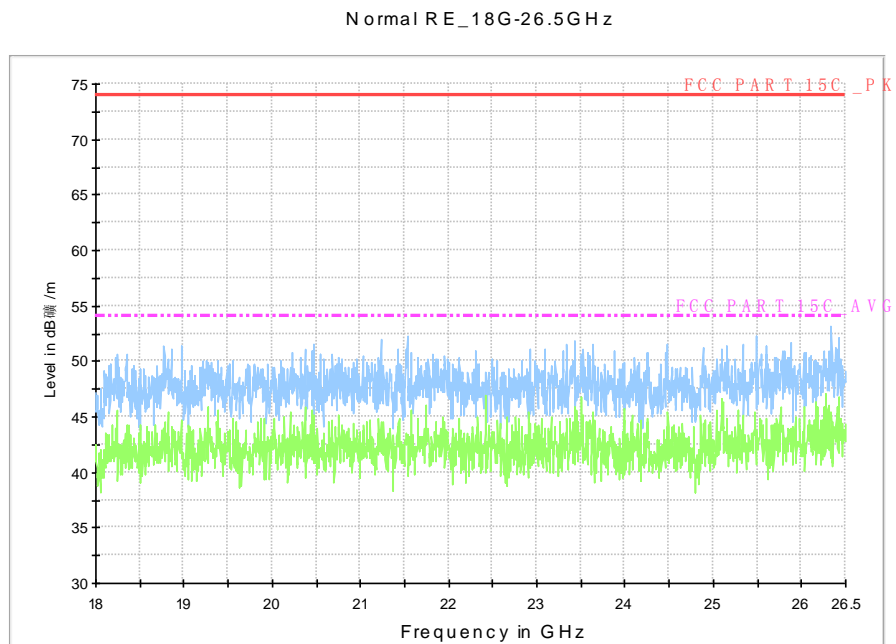
Fig. 64 Radiated Spurious Emission (802.11a, 18 GHz-26.5 GHz)
