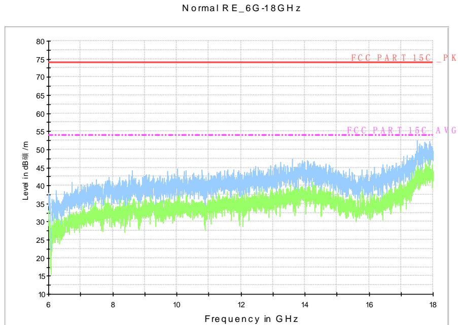
Fig. 70 Radiated Spurious Emission (802.11n-HT20, Ch157, 6 GHz-18 GHz)
