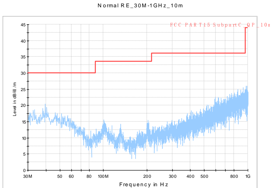
Fig. 68 Radiated Spurious Emission (802.11n-HT20, Ch157, 30 MHz-1 GHz)
