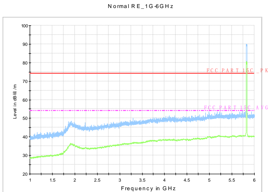
Fig. 62 Radiated Spurious Emission (802.11a, Ch165, 1 GHz-6 GHz)
