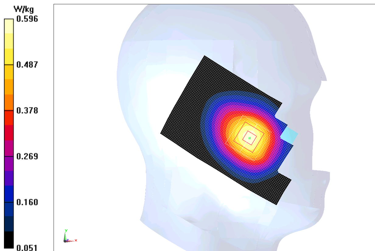
Fig.I.1 850MHz CH190
