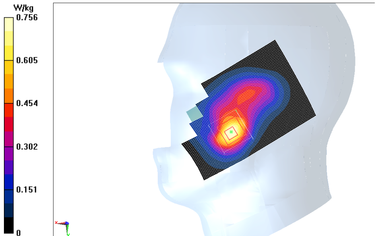
Fig.I.3 1900 MHz CH661
