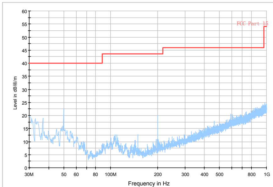
RE 30MHz-1GHz
