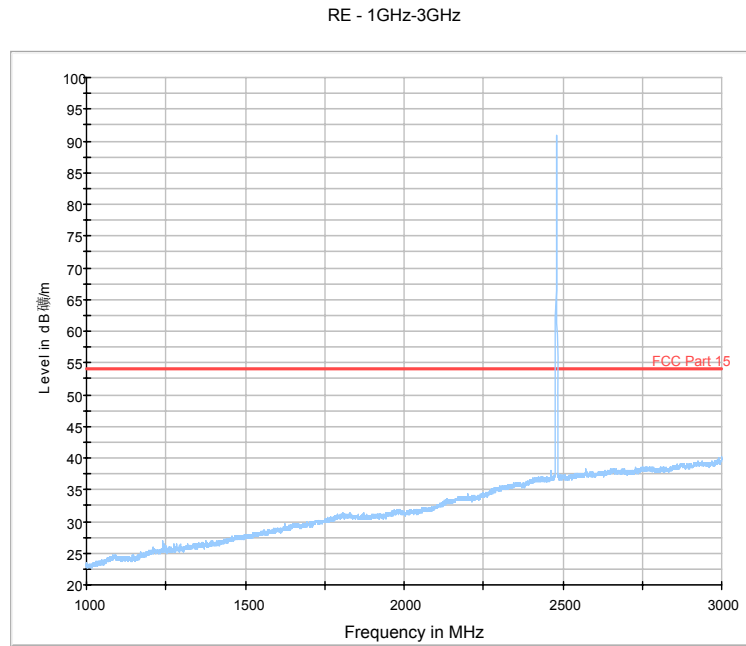
Fig.26. Radiated emission: GFSK, 2480MHz, 1 GHz - 3 GHz
