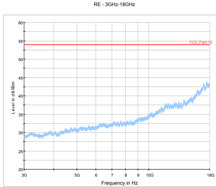
Fig.24. Radiated emission: GFSK, 2440MHz, 3 GHz - 18 GHz
