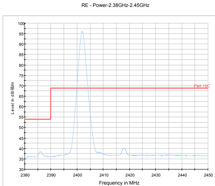
Fig.28. Radiated emission (Power): GFSK low channel
