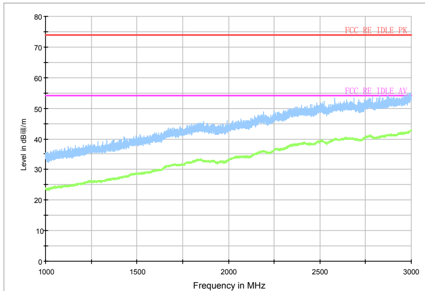
RE - 1GHz-3GHz
