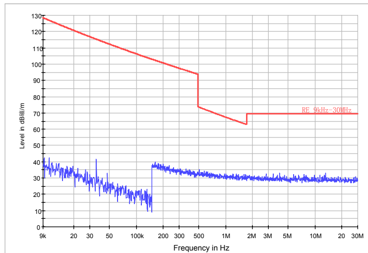
Fig.21. Radiated emission: GFSK, 2440MHz, 9KHz – 30MHz
