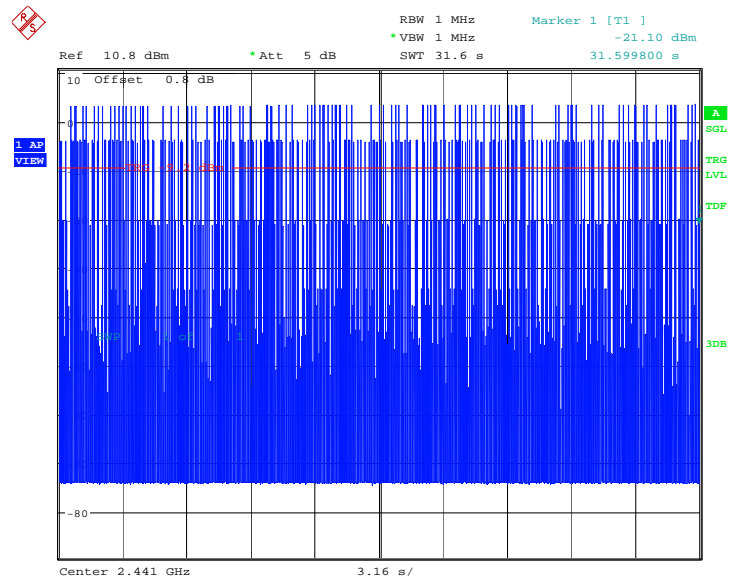
Fig.99. Time of occupancy (Dwell Time): Channel 39, Packet DH3
