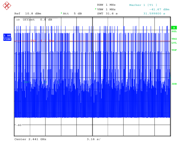
Fig.113. Time of occupancy (Dwell Time): Channel 39, Packet 3-DH5
