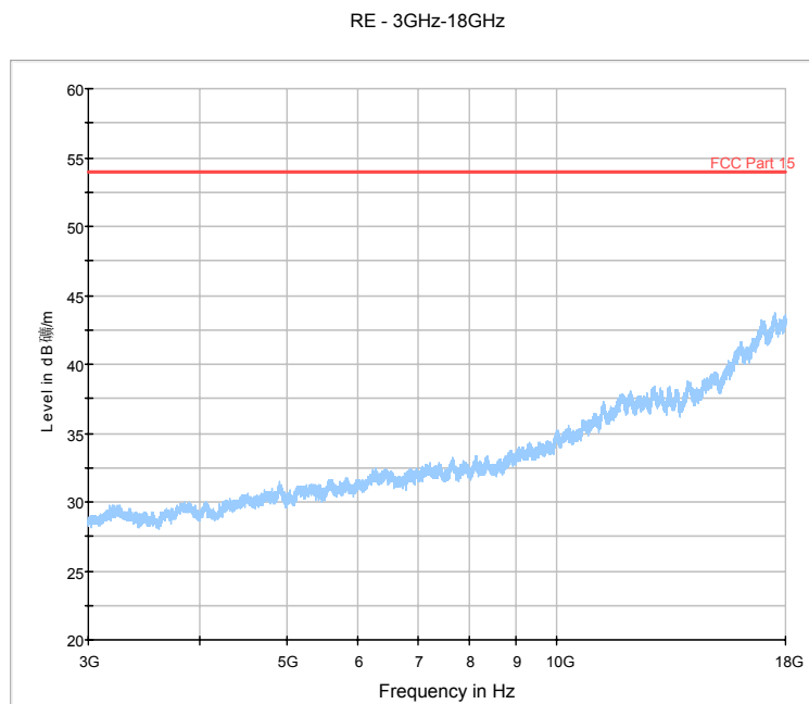
Fig.67. Radiated emission: GFSK, Channel 78, 3 GHz - 18 GHz
