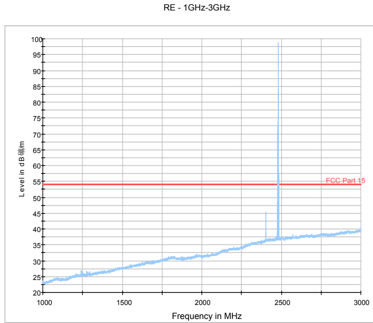
Fig.66. Fig.47 Radiated emission: GFSK, Channel 78, 1 GHz - 3 GHz
