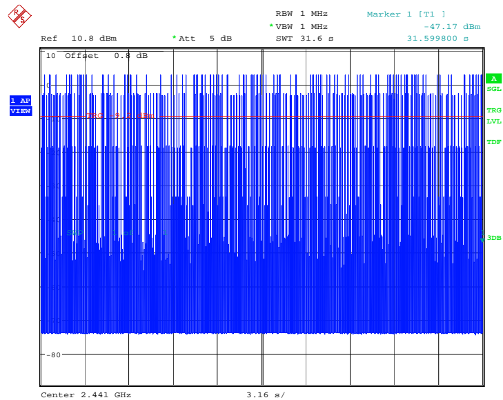
Fig.105. Time of occupancy (Dwell Time): Channel 39, Packet 2-DH3
