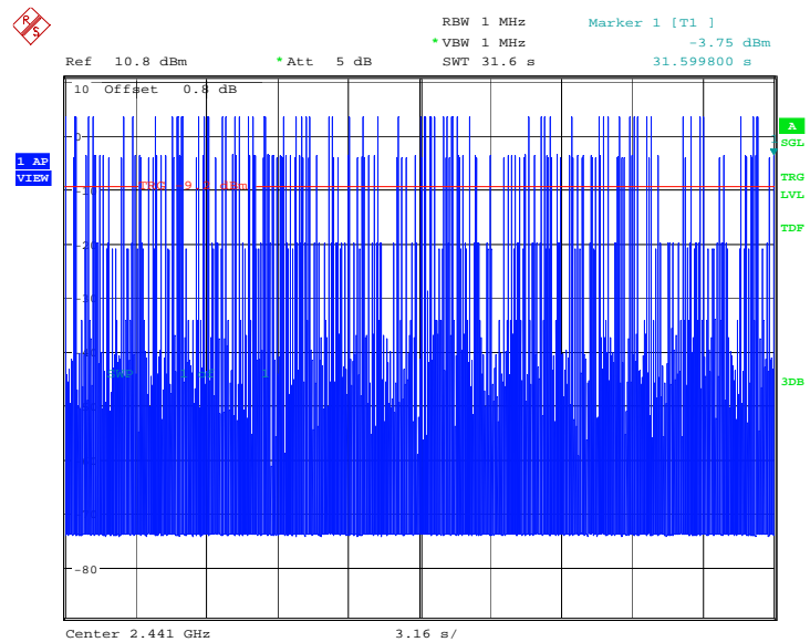
Fig.101. Time of occupancy (Dwell Time): Channel 39, Packet DH5
