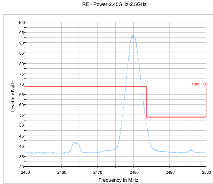
Fig.82. Radiated emission (Power): \pi/4 DQPSK, high channel
