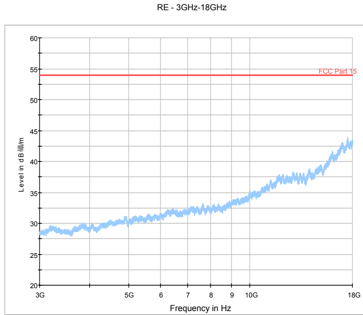
Fig.86. Radiated emission: 8DPSK, Channel 0, 3 GHz - 18 GHz
