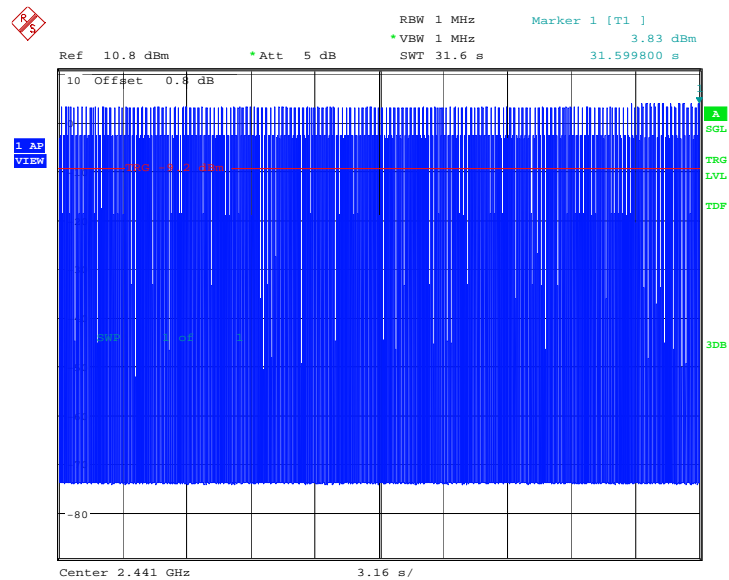
Fig.109. Time of occupancy (Dwell Time): Channel 39, Packet 3-DH1
