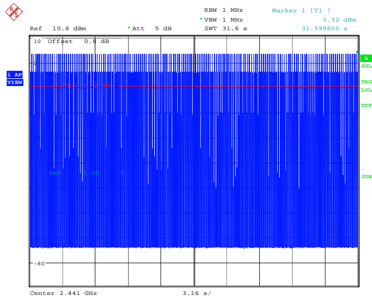
Fig.97. Time of occupancy (Dwell Time): Channel 39, Packet DH1
