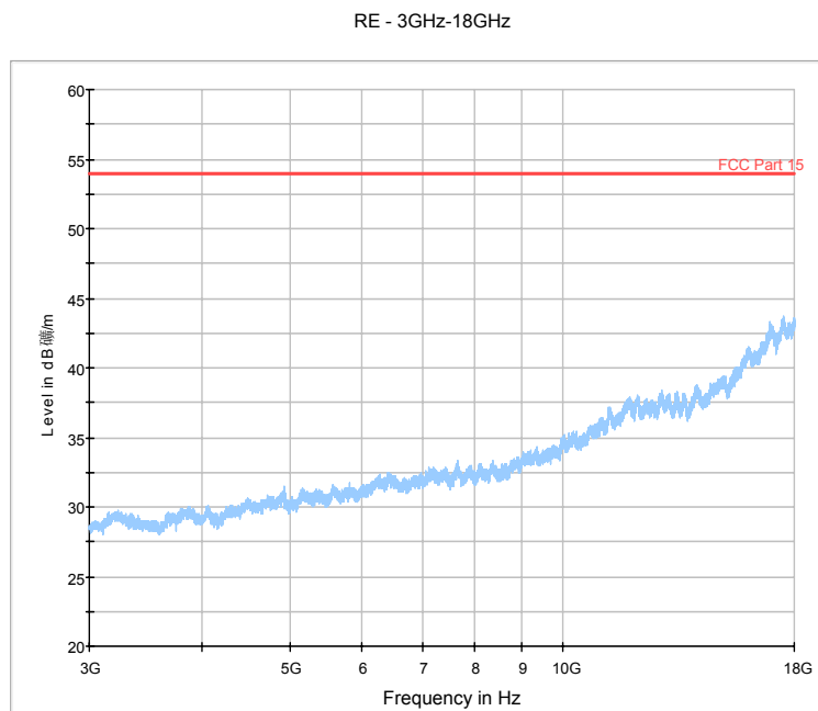
Fig.93. Radiated emission: 8DPSK, Channel 78, 3 GHz - 18 GHz
