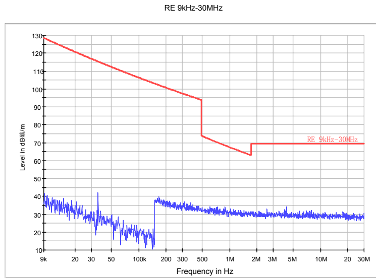
Fig.74. Radiated emission: \pi/4 DQPSK, Channel 39, 9KHz – 30MHz
