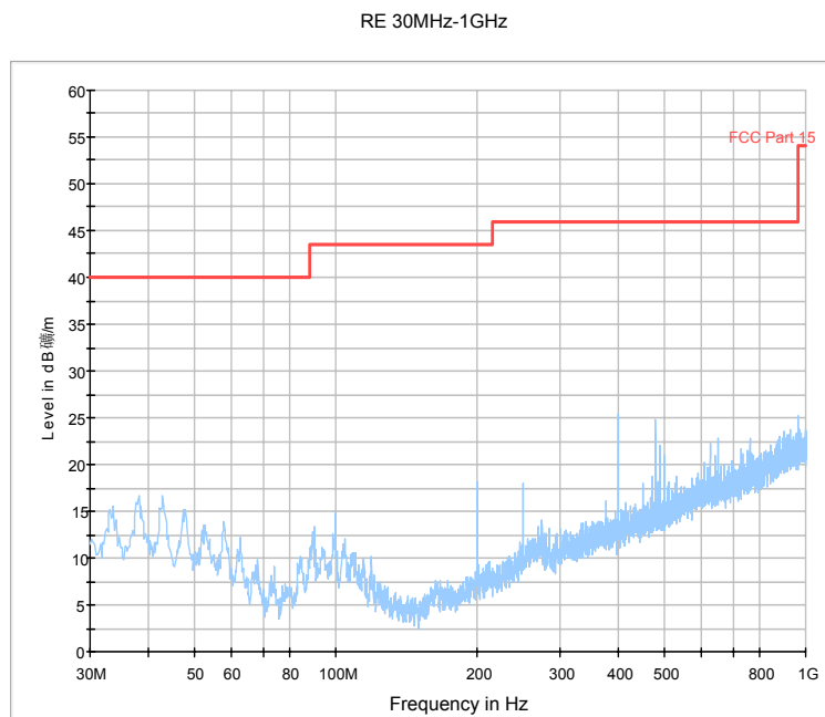
Fig.91. Radiated emission: 8DPSK, Channel 78, 30 MHz - 1 GHz
