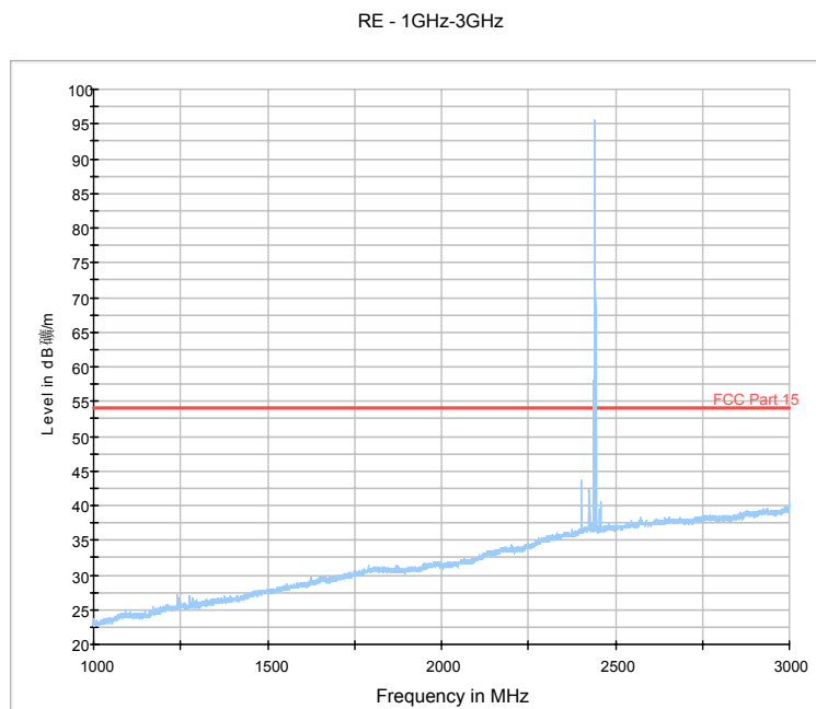
Fig.89. Radiated emission: 8DPSK, Channel 39, 1 GHz - 3 GHz
