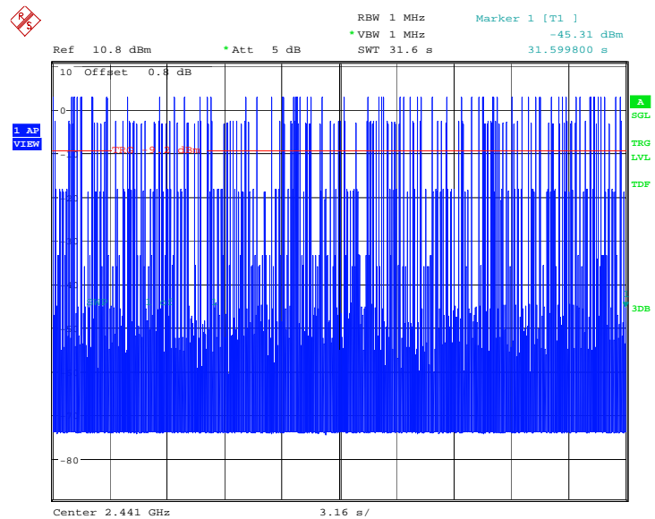
Fig.107. Time of occupancy (Dwell Time): Channel 39, Packet 2-DH5
