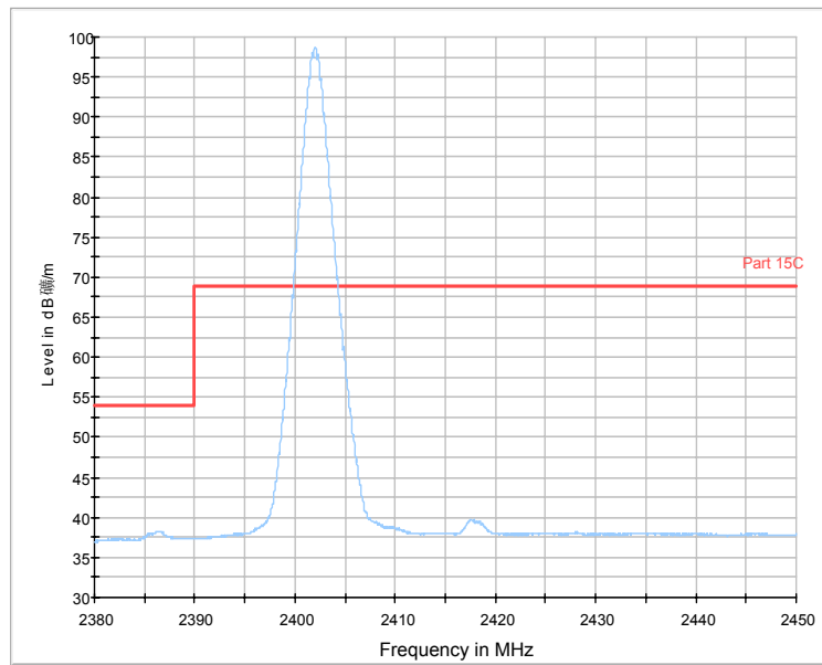
RE - Power-2.38GHz-2.45GHz
