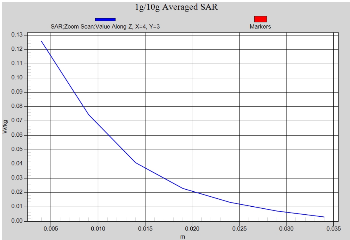
Fig. 10-1 Z-Scan at power reference point (2450 MHz CH1)
