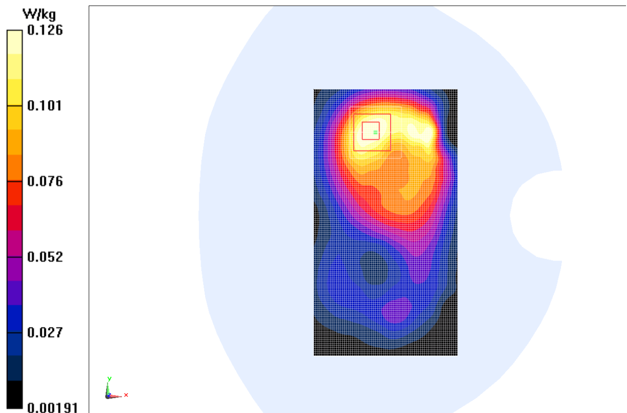
Fig.10 2450 MHz CH1
