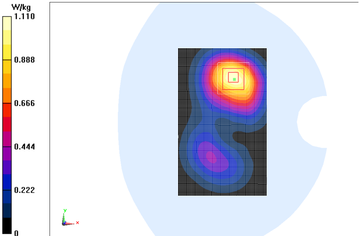
Fig.4 1900 MHz CH810
