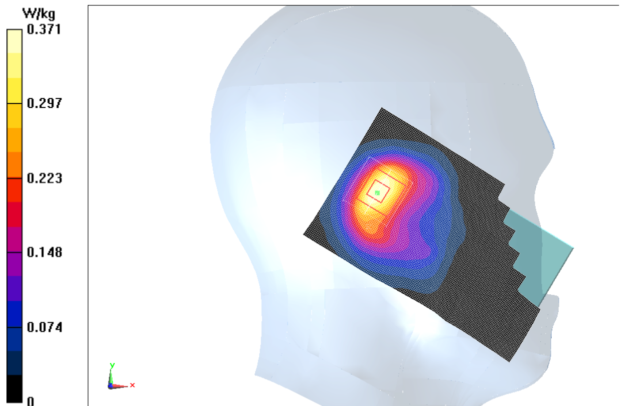
Fig.9 2450 MHz CH1
