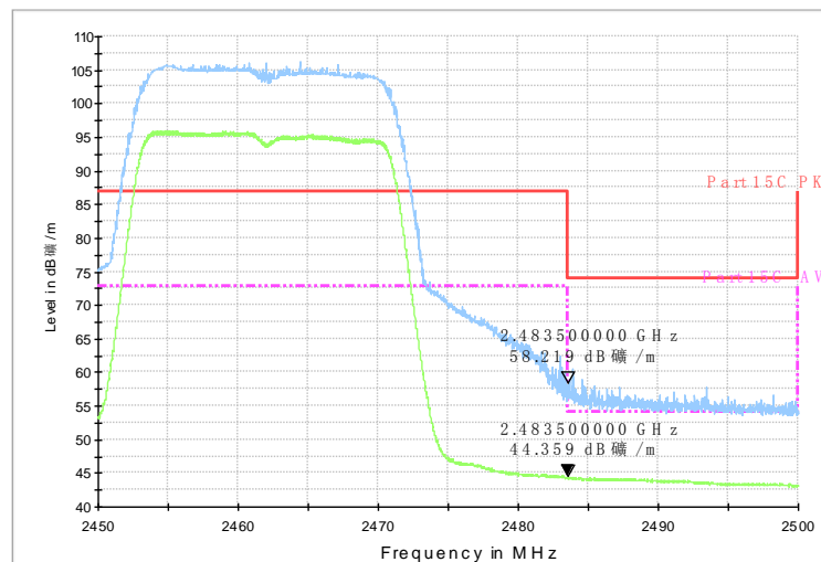
RE - Power-2.45GHz-2.5GHz
