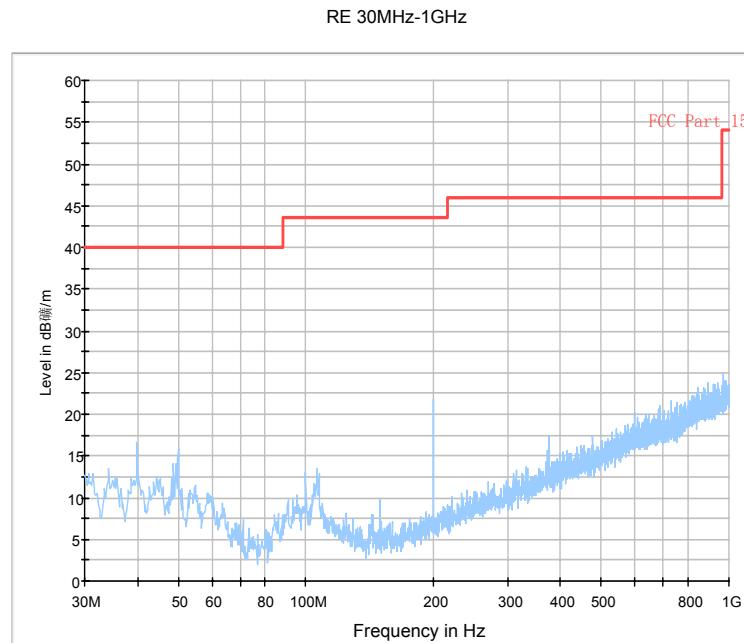
Fig.28. Radiated emission: GFSK, 2480MHz, 30 MHz - 1 GHz
