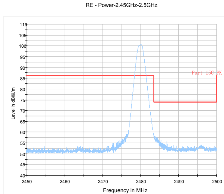
Fig.34. Radiated emission (Power): GFSK high channel (VBW=1MHz)
