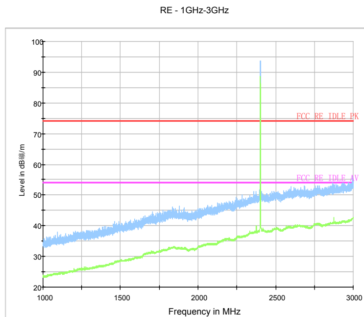
Fig.23. Radiated emission: GFSK, 2402MHz, 1 GHz - 3GHz
