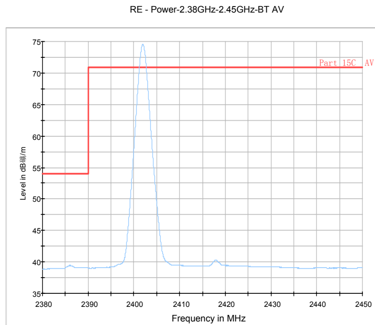
Fig.31. Radiated emission (Power): GFSK low channel (VBW=10Hz)
