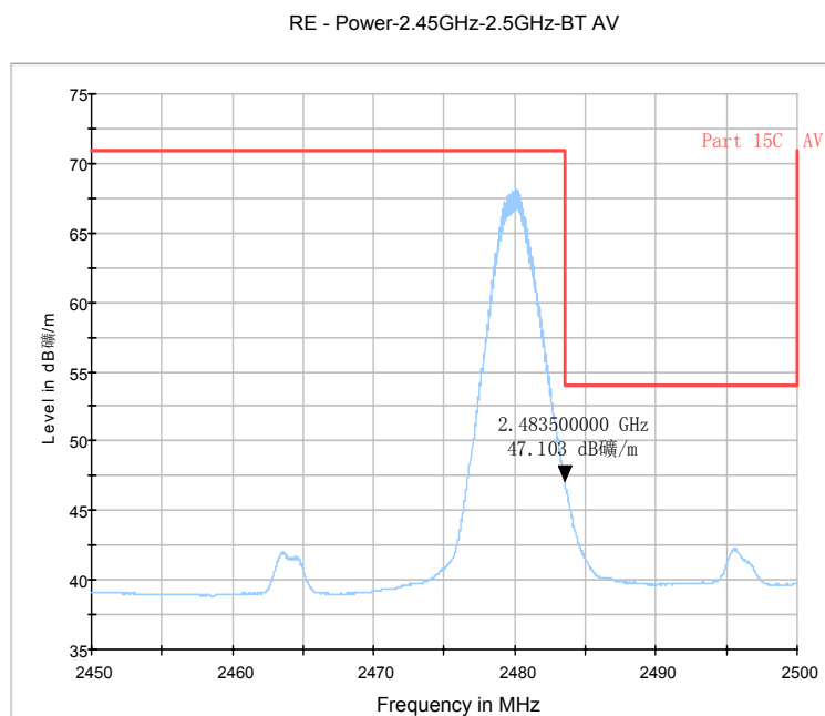
Fig.97. Radiated emission (Power): 8DPSK, high channel(VBW=10Hz)
