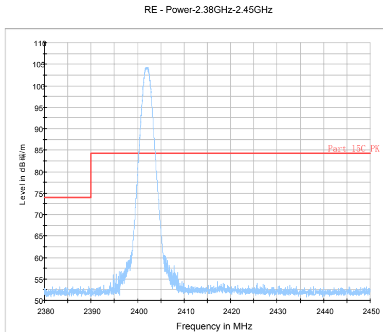
Fig.96. Radiated emission (Power): 8DPSK, low channel(VBW=1MHz)
