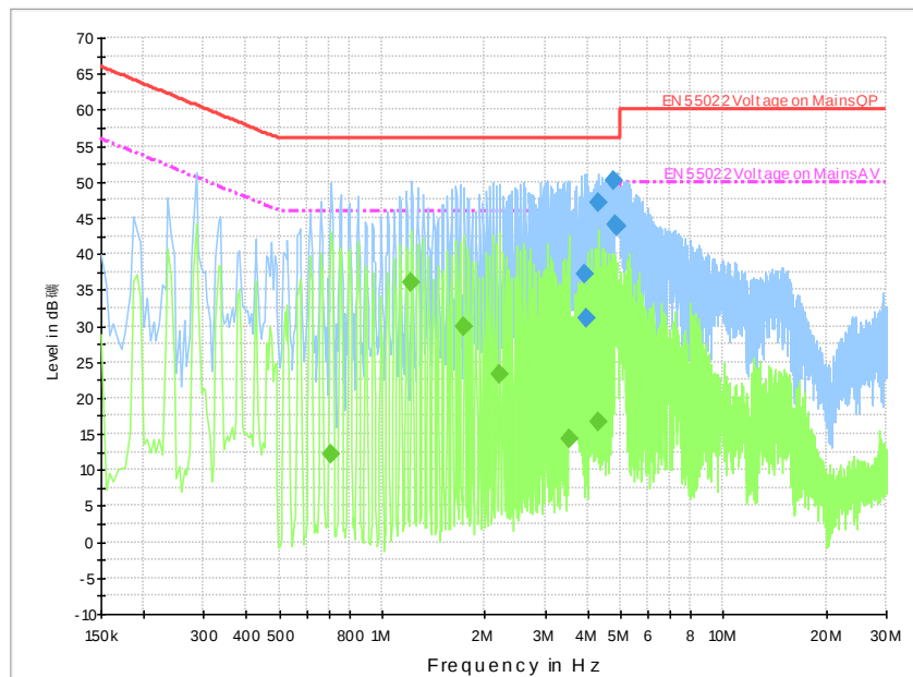
Fig. 293 AC Powerline Conducted Emission-IDLE with charger2
