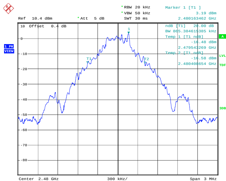
Fig.113. 20dB Bandwidth: GFSK, Channel 39
