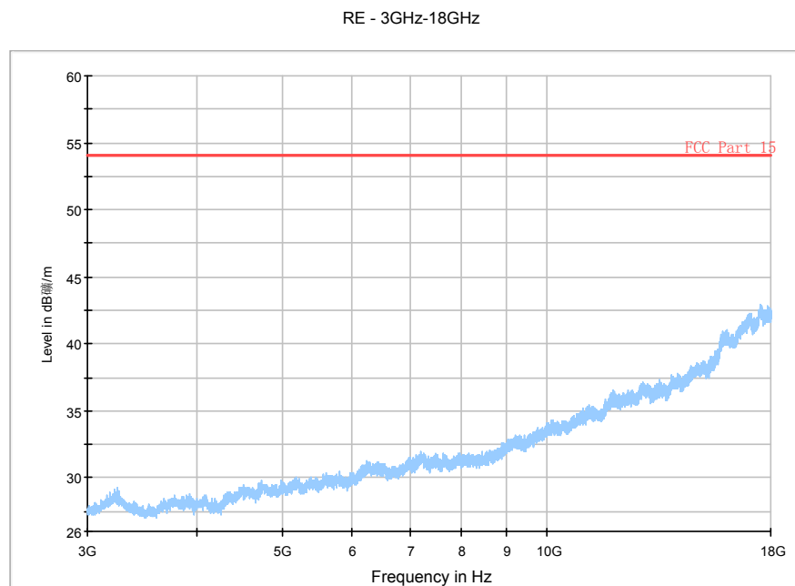
Fig. 139 Radiated Spurious Emission (802.11b, Ch11, 3 GHz-18 GHz)
