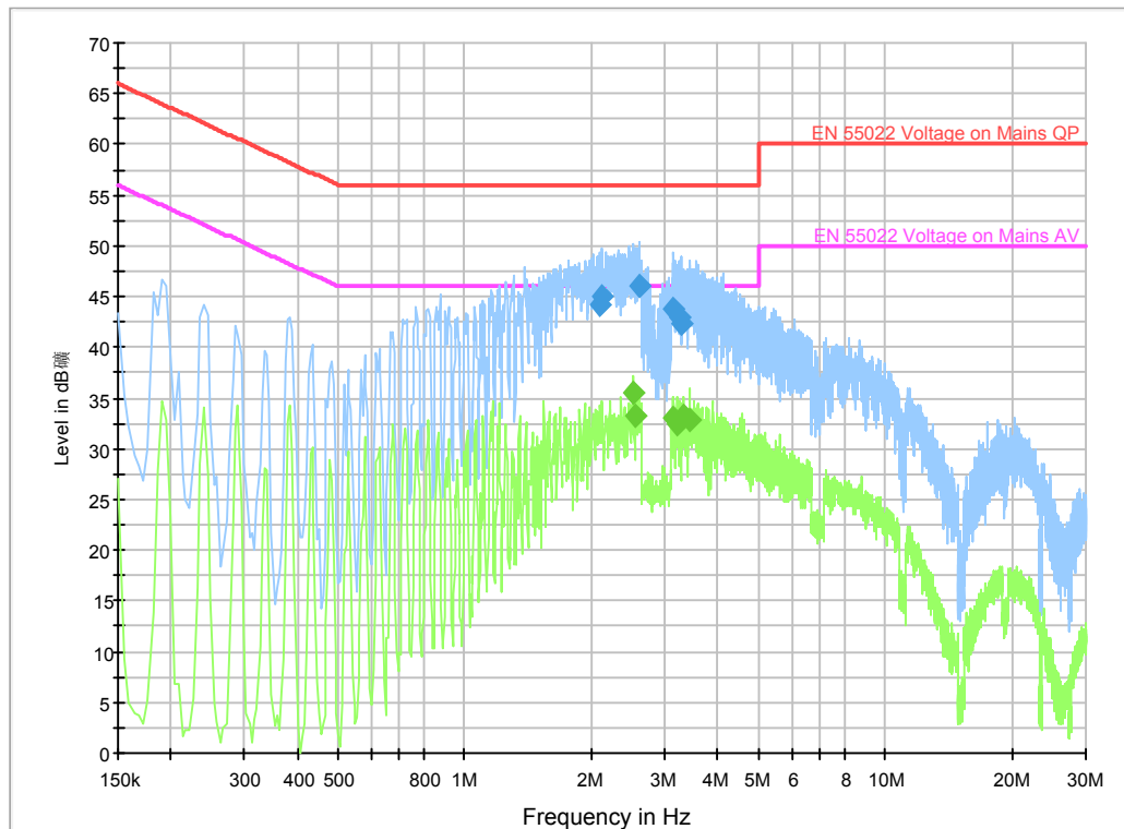
Fig. 174 AC Powerline Conducted Emission-802.11b with charger1
