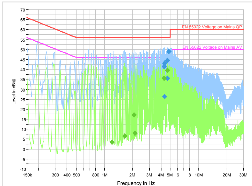
Fig. 176 AC Powerline Conducted Emission-802.11b with charger2
