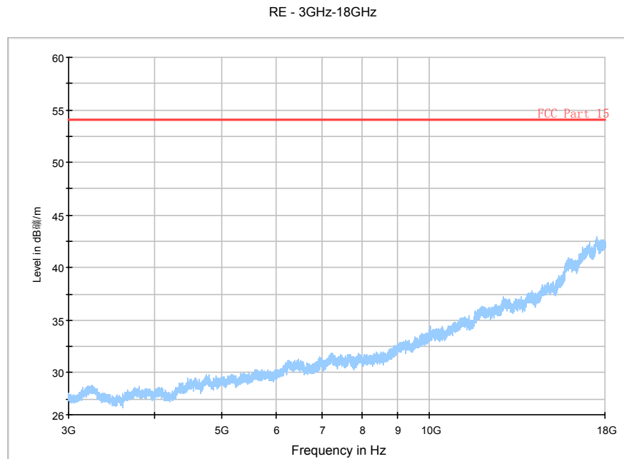
Fig. 157 Radiated Spurious Emission (802.11n-20MHz, Ch6, 3 GHz-18 GHz)
