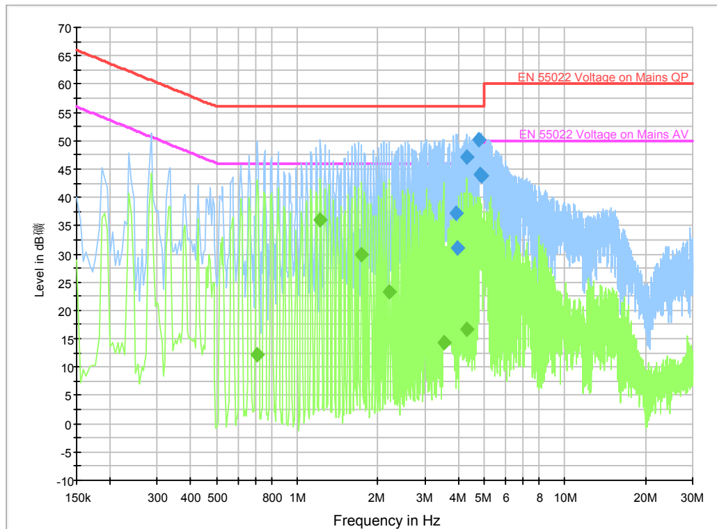
Fig. 177 AC Powerline Conducted Emission-IDLE with charger2
