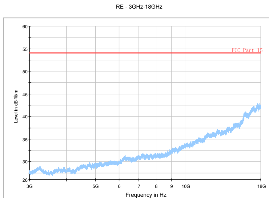
Fig. 146 Radiated Spurious Emission (802.11g, Ch6, 3 GHz-18 GHz)
