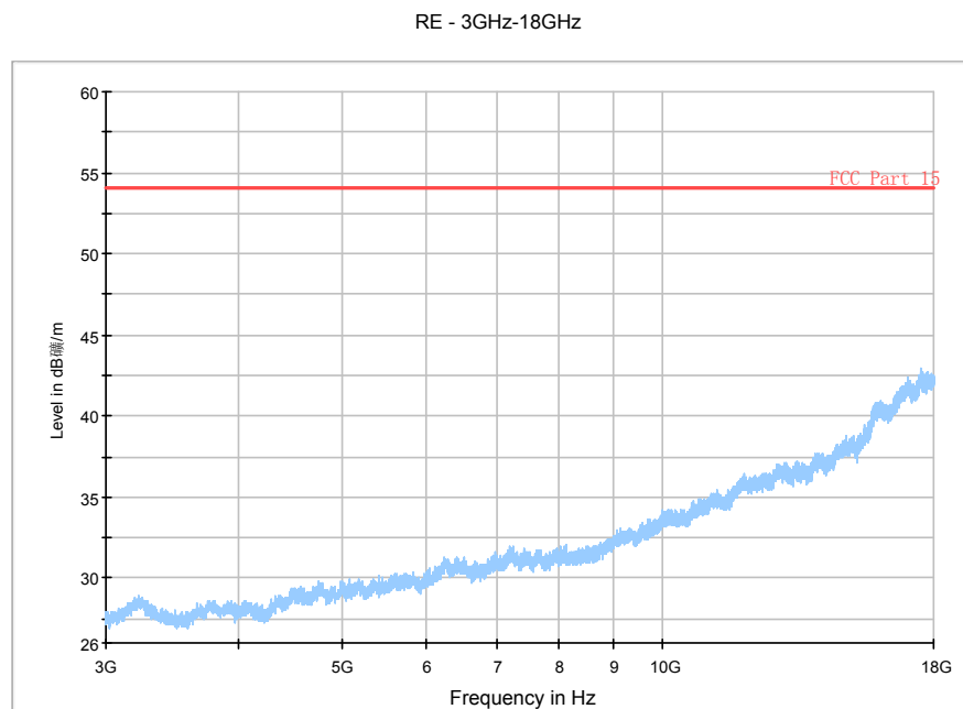
Fig. 143 Radiated Spurious Emission (802.11g, Ch1, 3 GHz-18 GHz)
