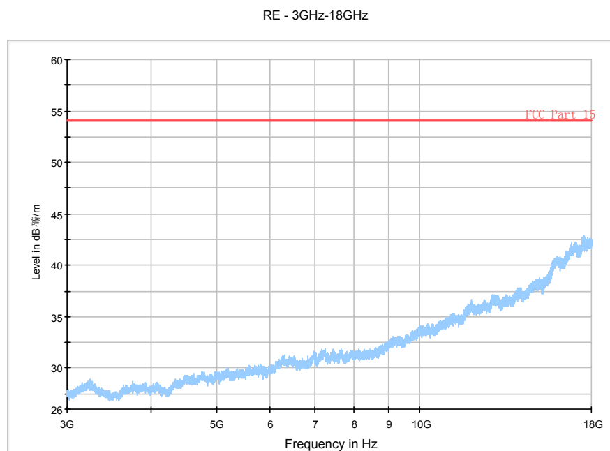
Fig. 154 Radiated Spurious Emission (802.11n-20MHz, Ch1, 3 GHz-18 GHz)
