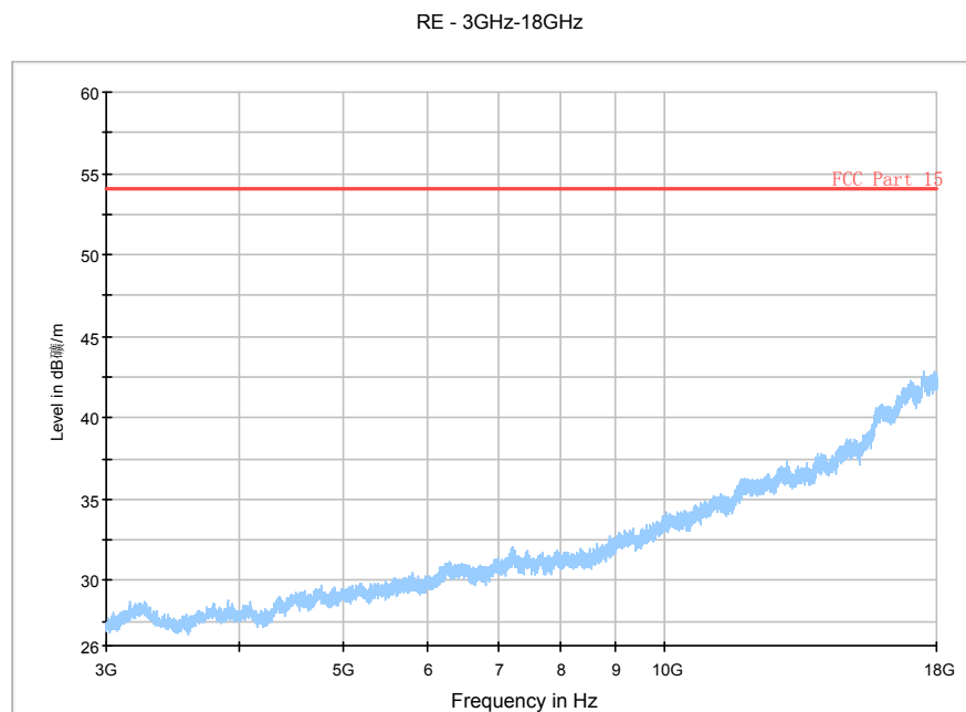
Fig. 161 Radiated Spurious Emission (802.11n-20MHz, Ch11, 3 GHz-18 GHz)
