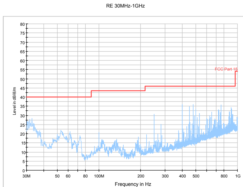
Fig. 130 Radiated Spurious Emission (802.11b, Ch1, 30 MHz-1 GHz)
