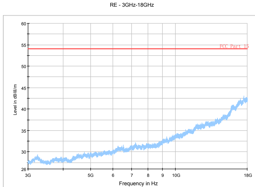
Fig. 135 Radiated Spurious Emission (802.11b, Ch6, 3 GHz-18 GHz)
