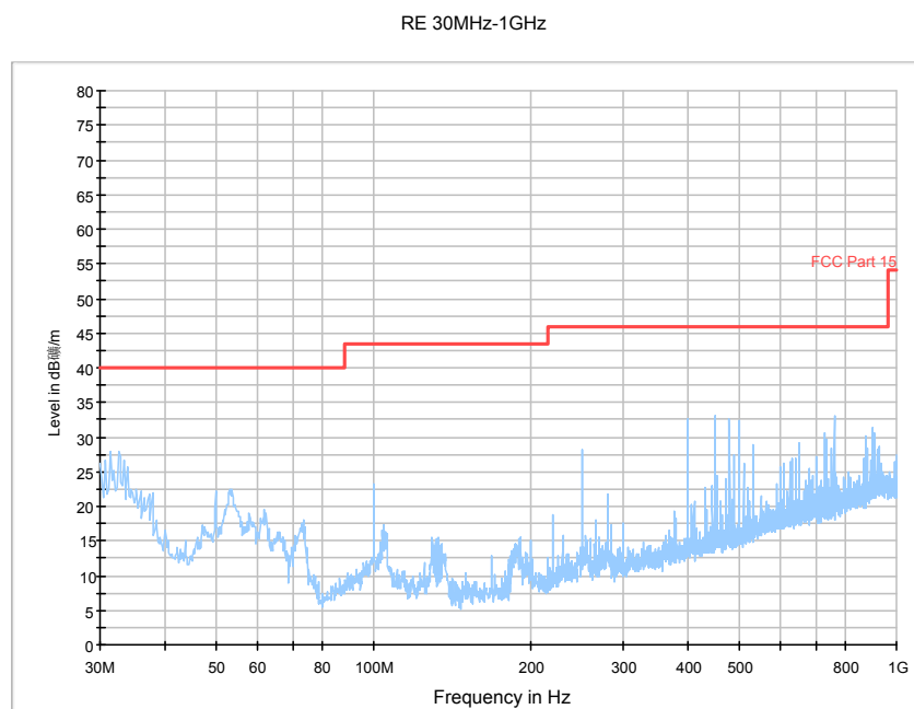
Fig. 166 Radiated Spurious Emission (802.11n-40MHz, Ch6, 30 MHz-1 GHz)
