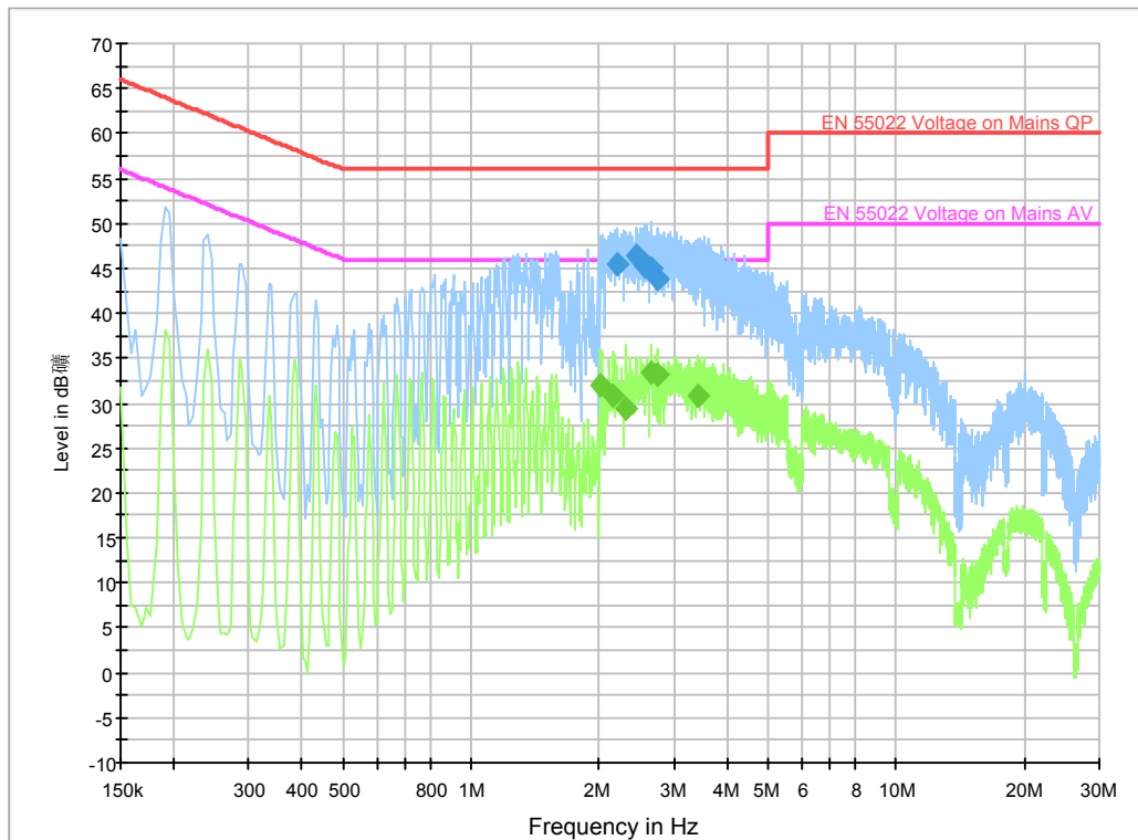
Fig. 175 AC Powerline Conducted Emission-IDLE with charger1
