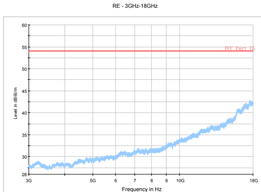
Fig. 132 Radiated Spurious Emission (802.11b, Ch1, 3 GHz-18 GHz)
