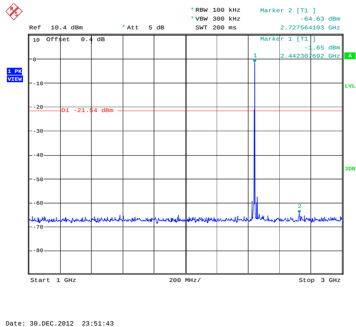
Fig.10. Conducted spurious emission: GFSK, 2440 MHz, 1GHz – 3GHz
