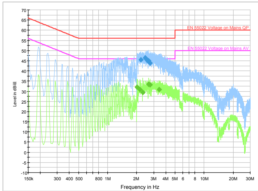
Fig. 175 AC Powerline Conducted Emission-IDLE with charger1
