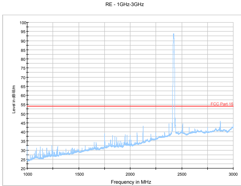
Fig. 131 Radiated Spurious Emission (802.11b, Ch1, 1 GHz-3 GHz)
