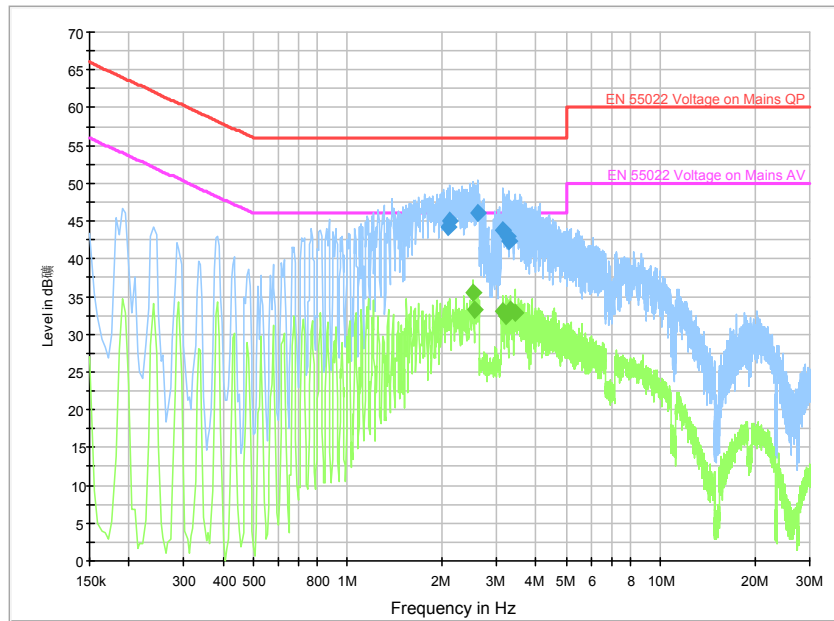
Fig. 174 AC Powerline Conducted Emission-802.11b with charger1
