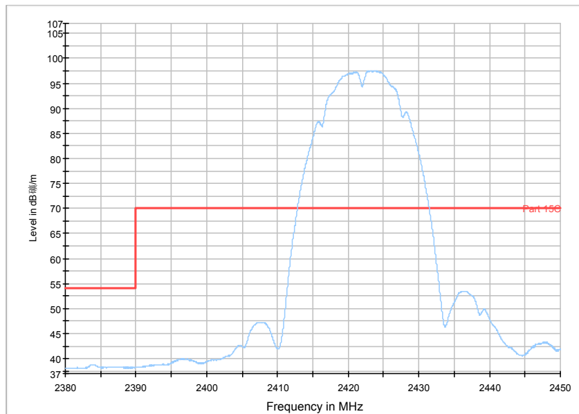
RE - Power-2.38GHz-2.45GHz
