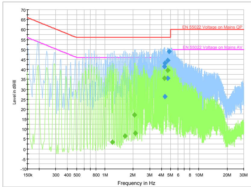
Fig. 176 AC Powerline Conducted Emission-802.11b with charger2
