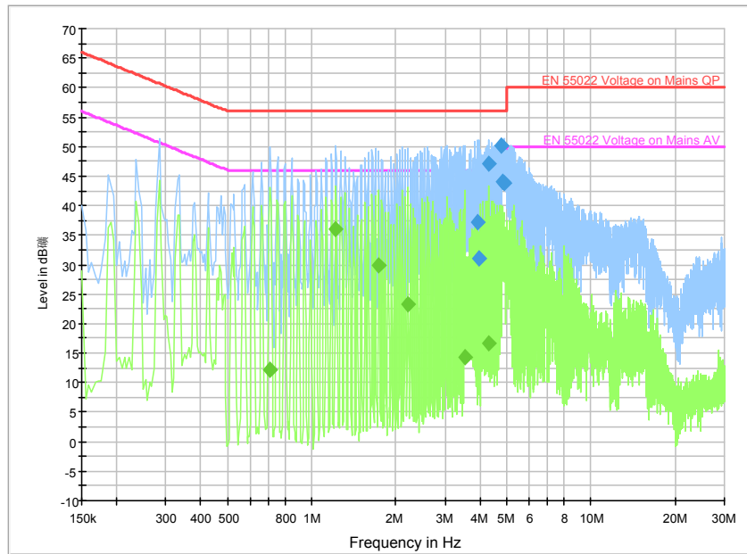
Fig. 177 AC Powerline Conducted Emission-IDLE with charger2
