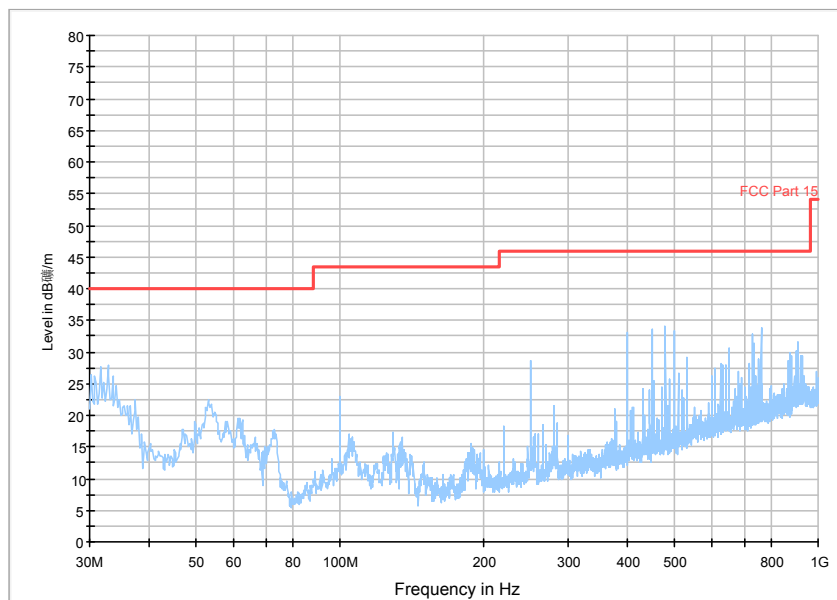
RE 30MHz-1GHz
