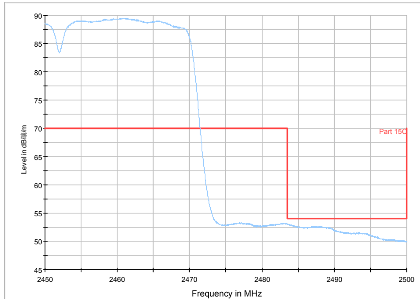
RE - Power-2.45GHz-2.5GHz
