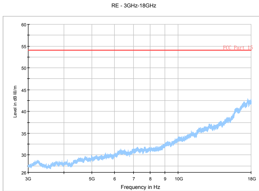
Fig. 150 Radiated Spurious Emission (802.11g, Ch11, 3 GHz-18 GHz)
