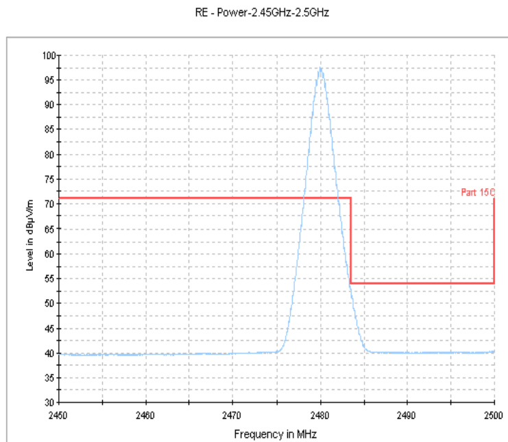
Fig.92. Radiated emission (Power): 8DPSK, high channel
