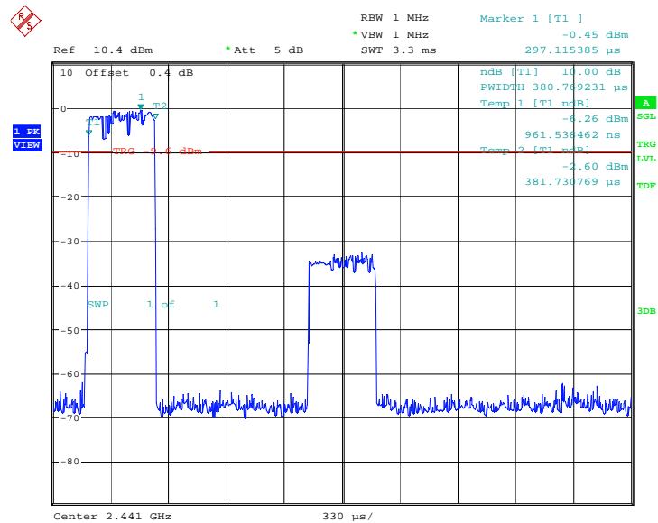
Fig.105. Number of Transmissions Measurement:Channel 39,Packet 2-DH5
