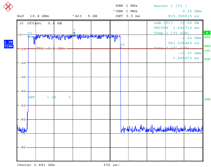
Fig.107. Number of Transmissions Measurement:Channel 39,Packet 3-DH1
