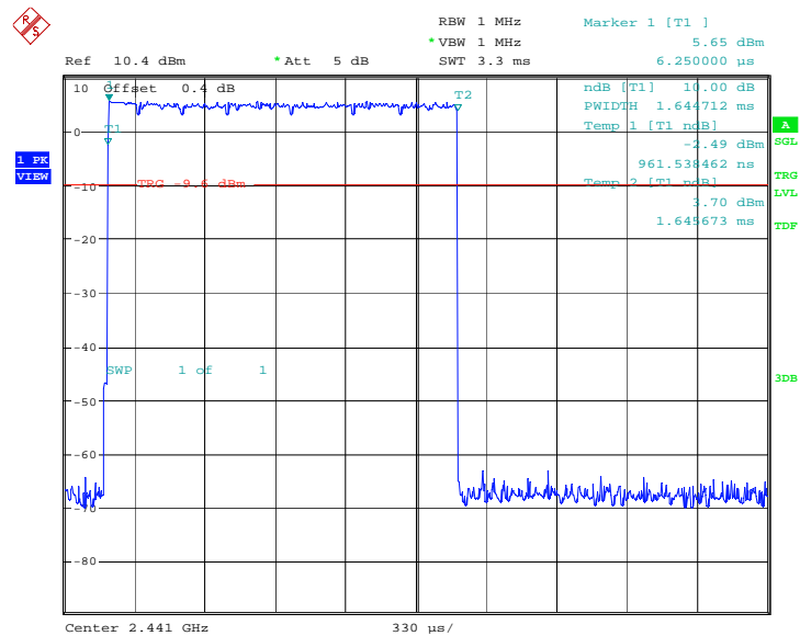
Fig.101. Number of Transmissions Measurement:Channel 39,Packet 2-DH1
