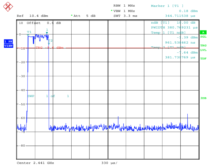
Fig.99. Number of Transmissions Measurement:Channel 39,Packet DH5
