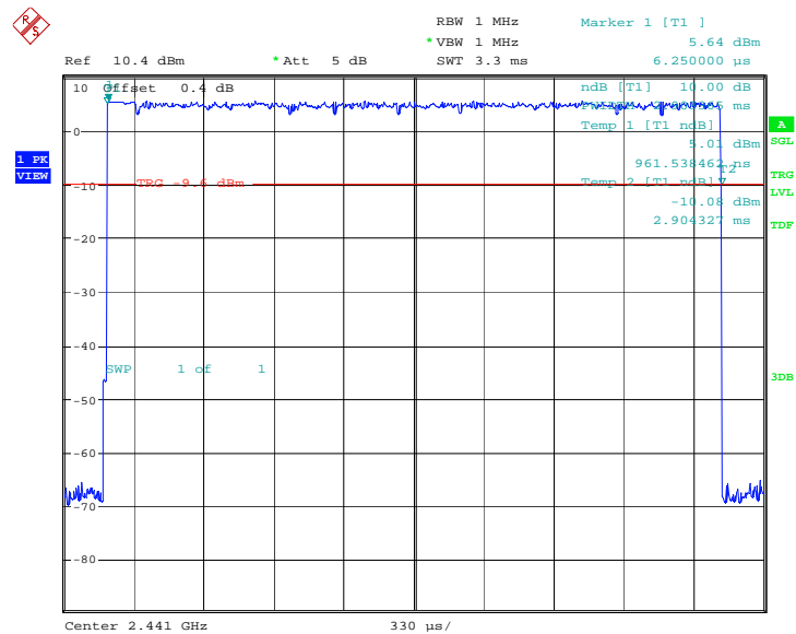
Fig.103. Number of Transmissions Measurement:Channel 39,Packet 2-DH3
