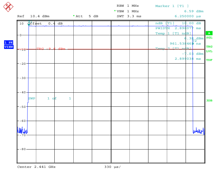
Fig.97. Number of Transmissions Measurement:Channel 39,Packet DH3
