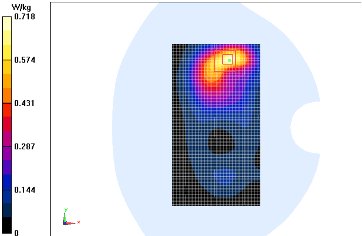
Fig.4 1900 MHz CH810
