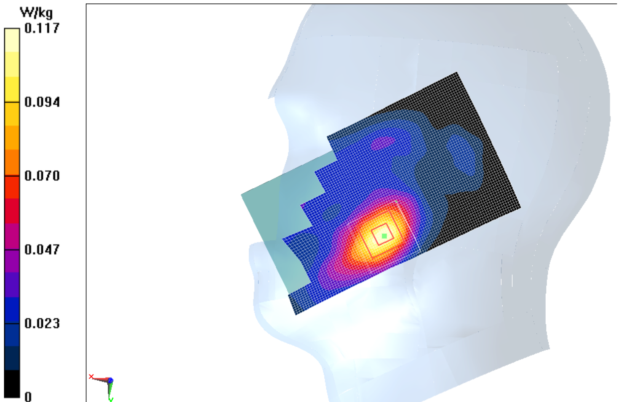
Fig.3 1900 MHz CH810
