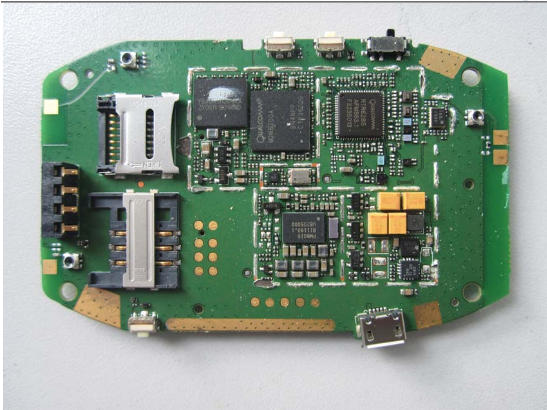
6. GSM/WCDMA chip view
