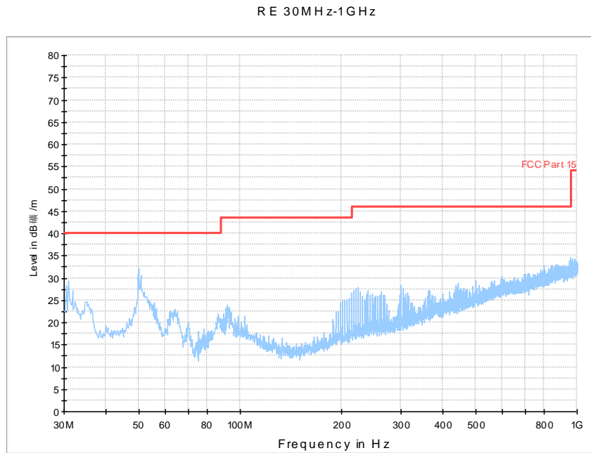
Fig. 23 Radiated Spurious Emission (802.11a, ch36, 30 MHz-1 GHz)
