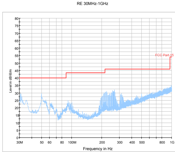
Fig.21. Radiated emission: GFSK, 2440MHz, 30 MHz - 1 GHz
