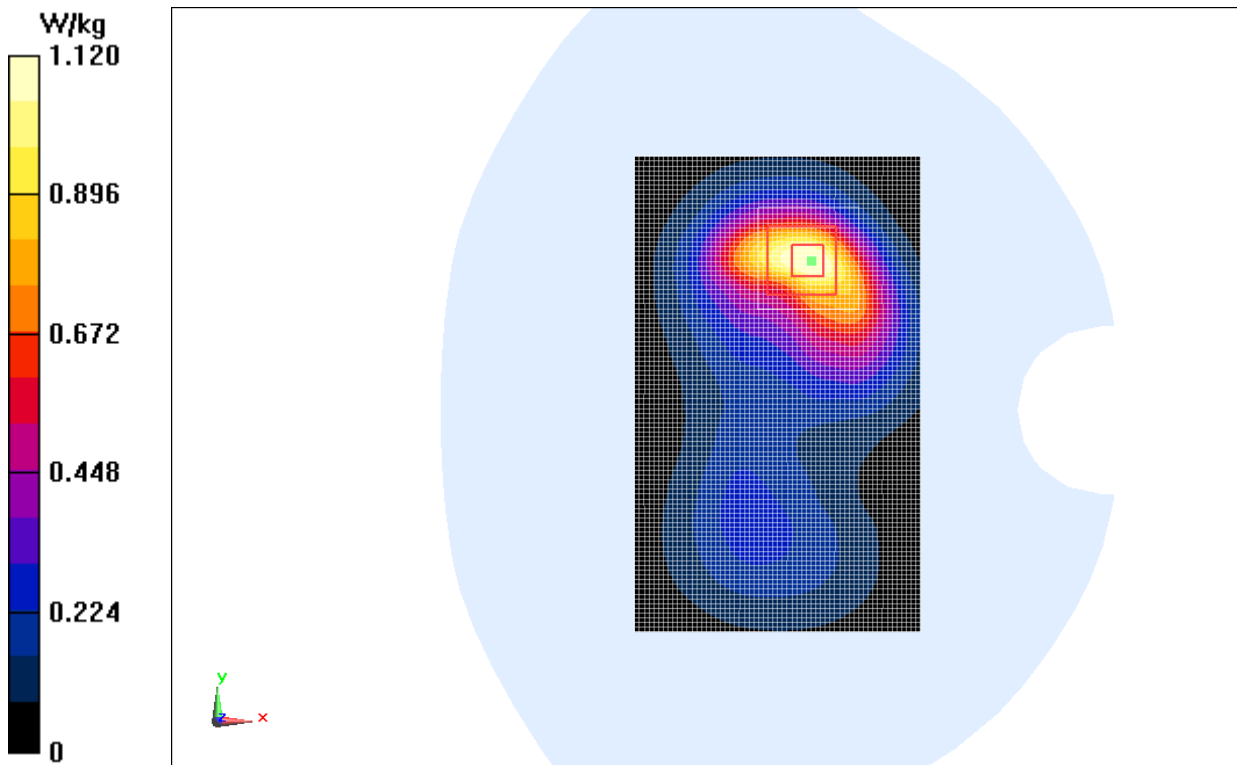
Fig.4 1900 MHz CH810
