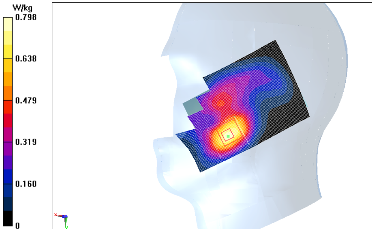
Fig.7 WCDMA 1700 CH1412
