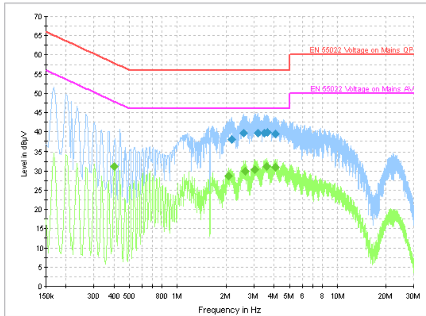
Fig. 175 AC Powerline Conducted Emission-802.11g
