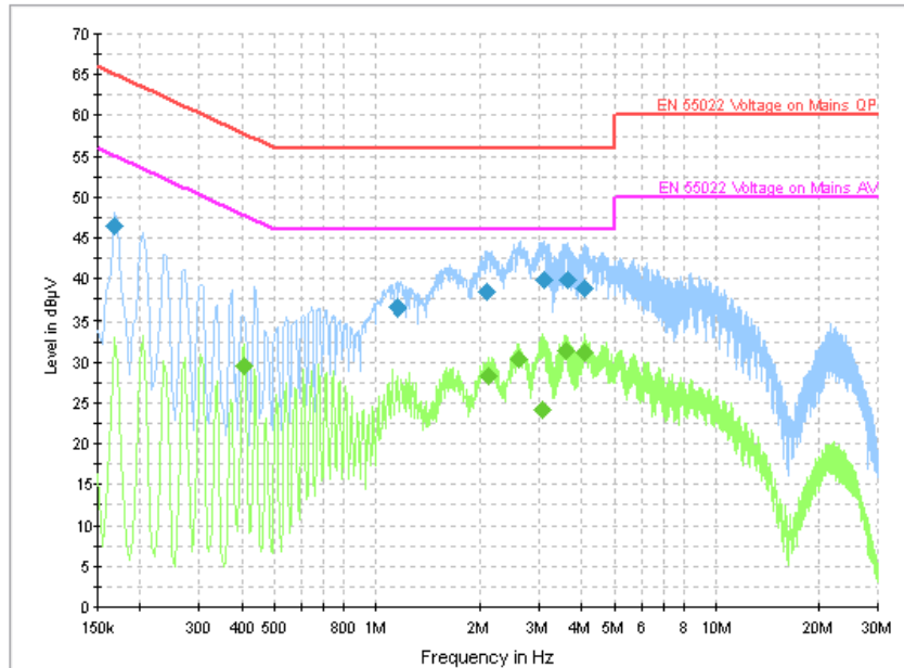
Fig. 177 AC Powerline Conducted Emission-802.11n-HT40
