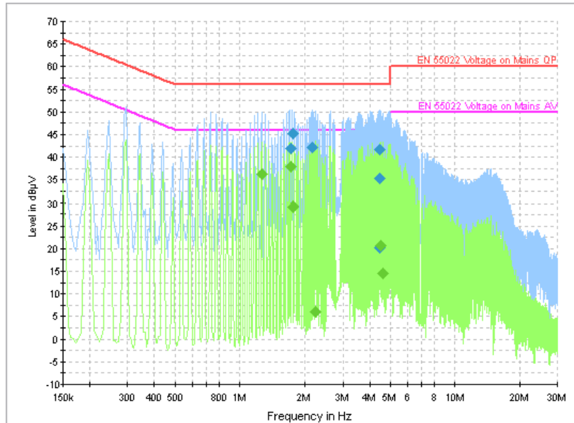
Fig. 179 AC Powerline Conducted Emission-802.11g
