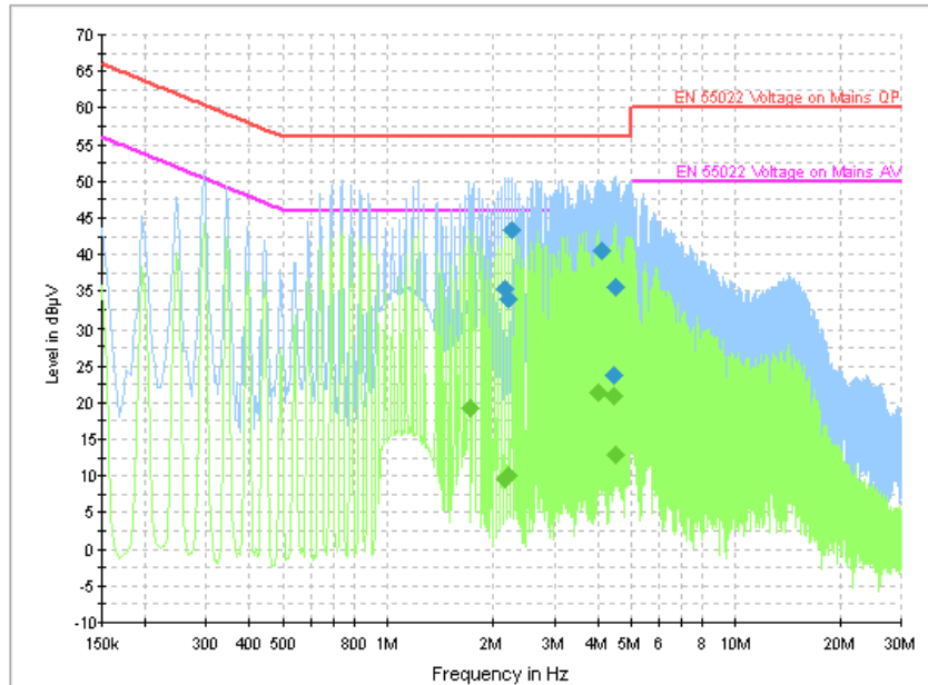
Fig. 180 AC Powerline Conducted Emission-802.11n-HT20
