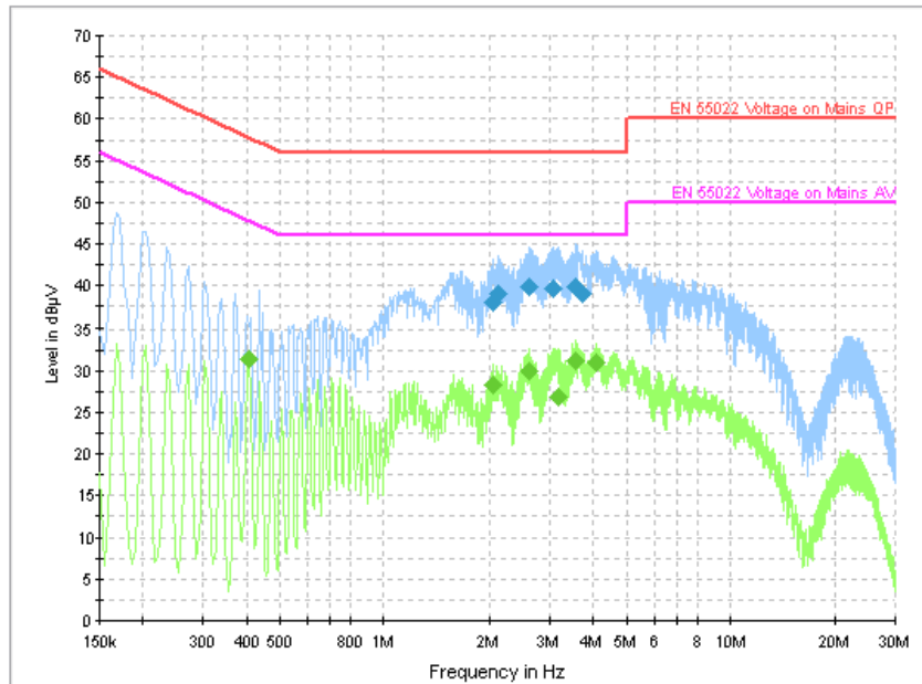
Fig. 176 AC Powerline Conducted Emission-802.11n-HT20
