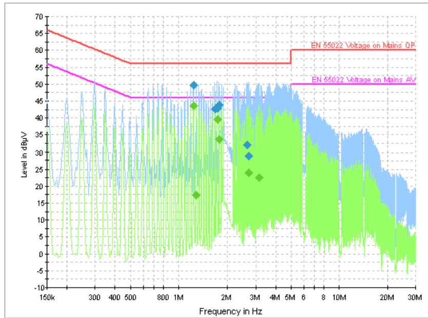
Fig. 181 AC Powerline Conducted Emission-802.11n-HT40
