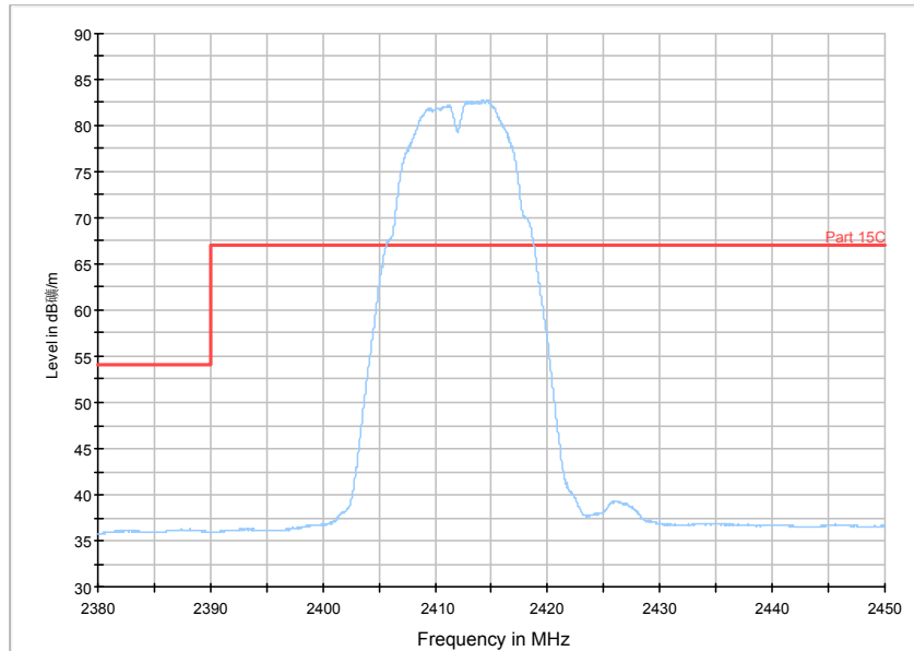
RE - Power-2.38GHz-2.45GHz
