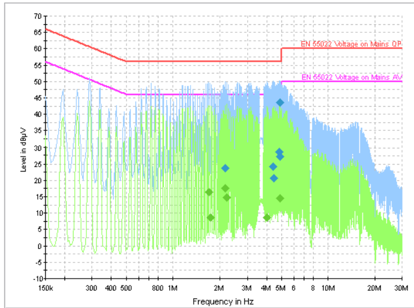
Fig. 178 AC Powerline Conducted Emission-802.11b
