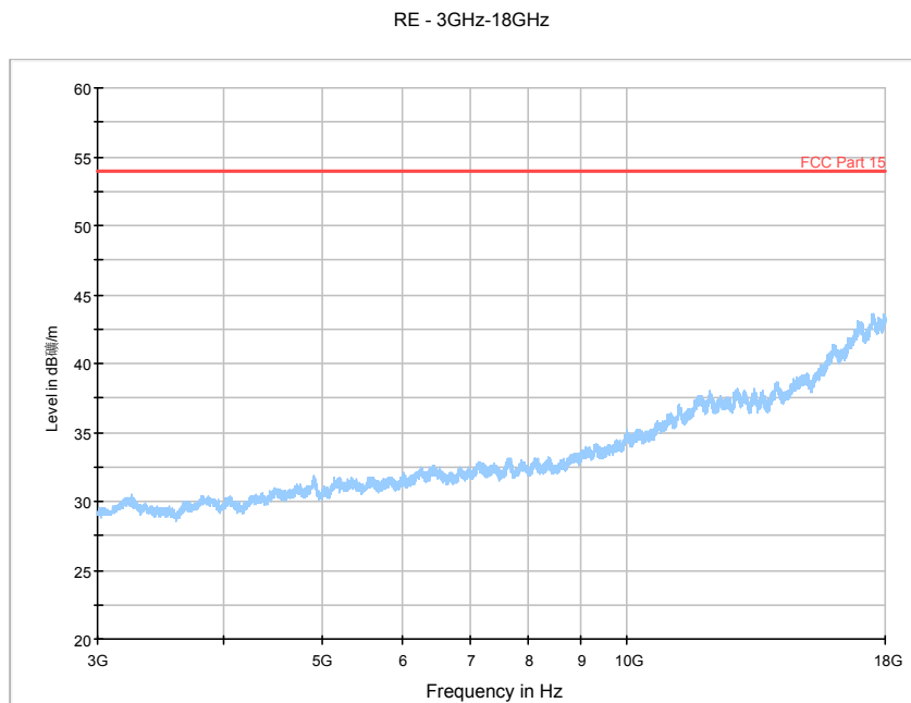
Fig. 161 Radiated Spurious Emission (802.11n-20MHz, Ch11, 3 GHz-18 GHz)
