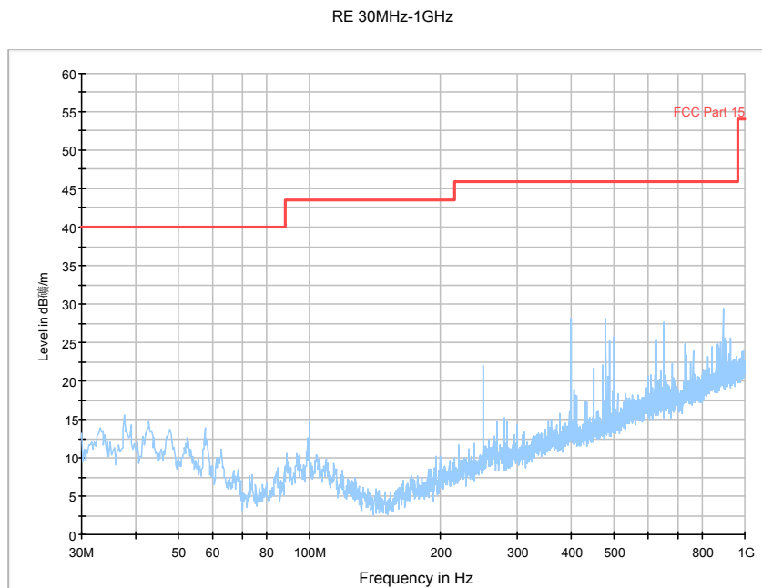
Fig. 159 Radiated Spurious Emission (802.11n-20MHz, Ch11, 30 MHz-1 GHz)
