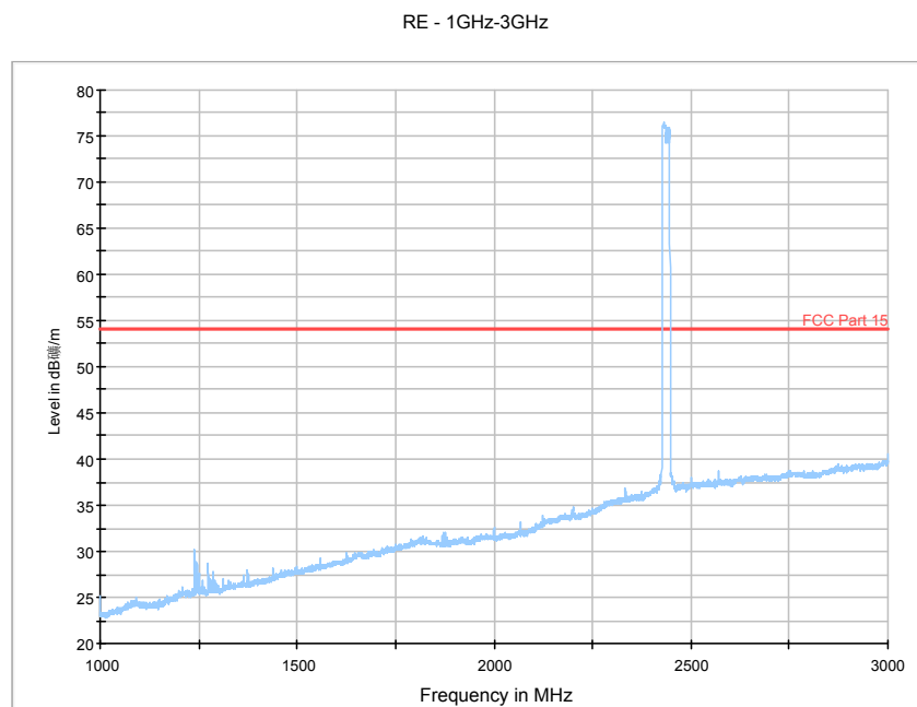
Fig. 156 Radiated Spurious Emission (802.11n-20MHz, Ch6, 1 GHz-3 GHz)
