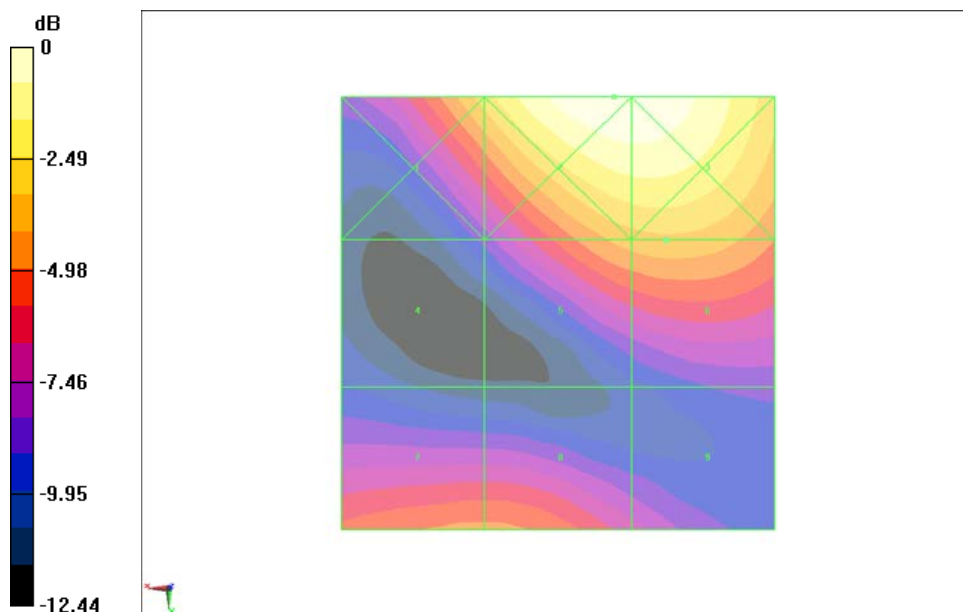
Fig B.11 HAC RF E-Field WCDMA 1700 Middle
