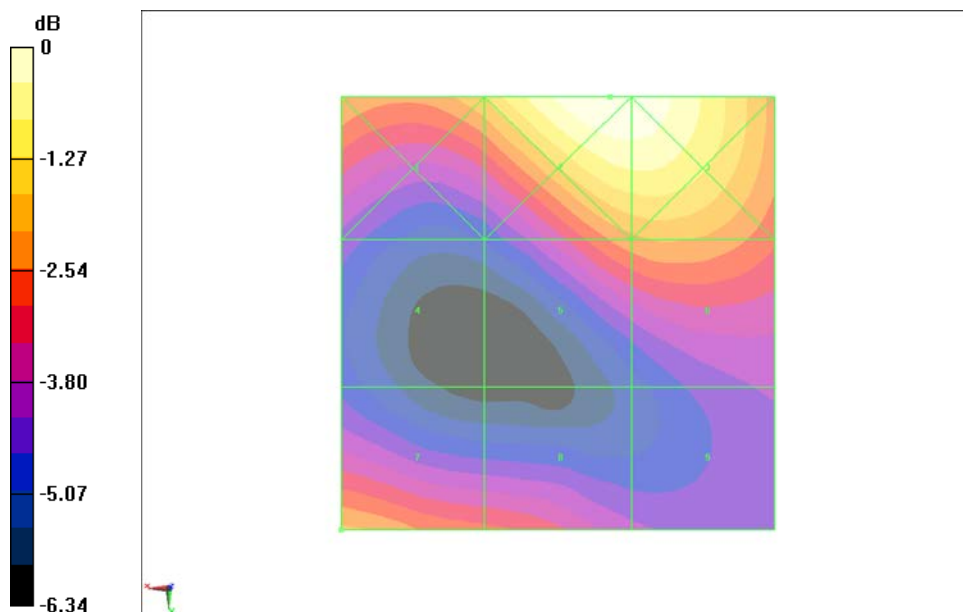
Fig B.13 HAC RF E-Field WCDMA 1900 High
