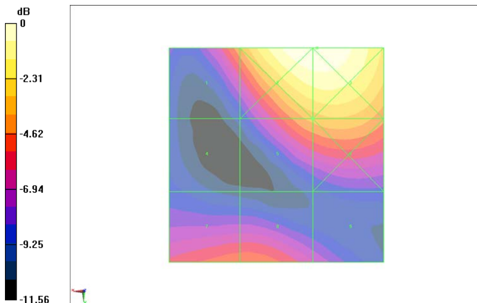
Fig B.10 HAC RF E-Field WCDMA 1700 High
