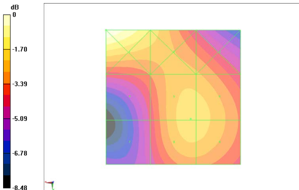
Fig B.27 HAC RF H-Field WCDMA 1700 Low
