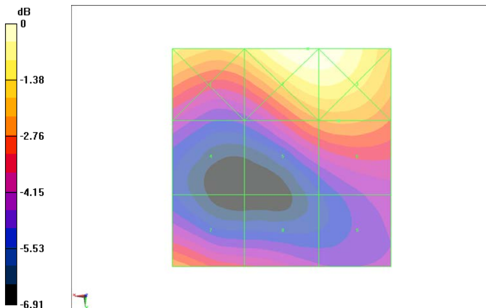
Fig B.15 HAC RF E-Field WCDMA 1900 Low
