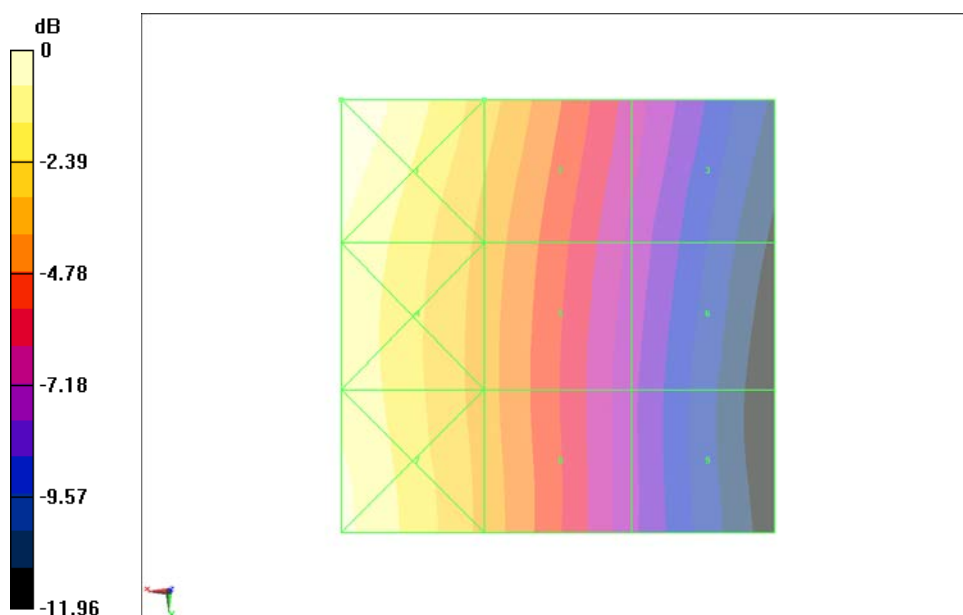
Fig B.22 HAC RF H-Field WCDMA 850 High
