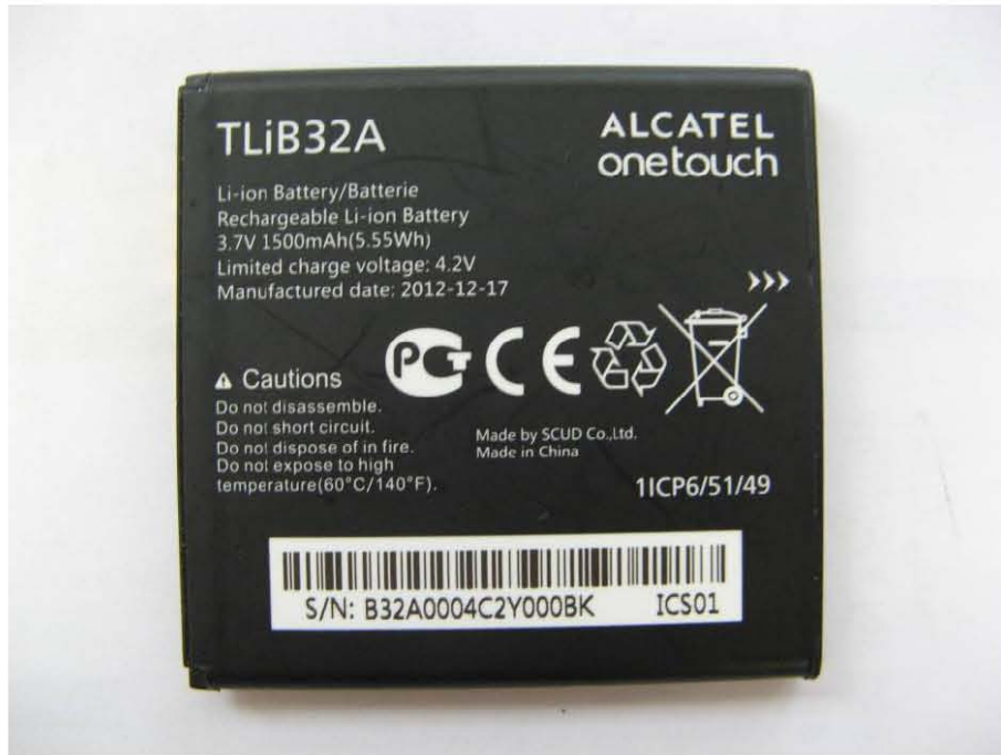
Picture B-9: Battery AE2
