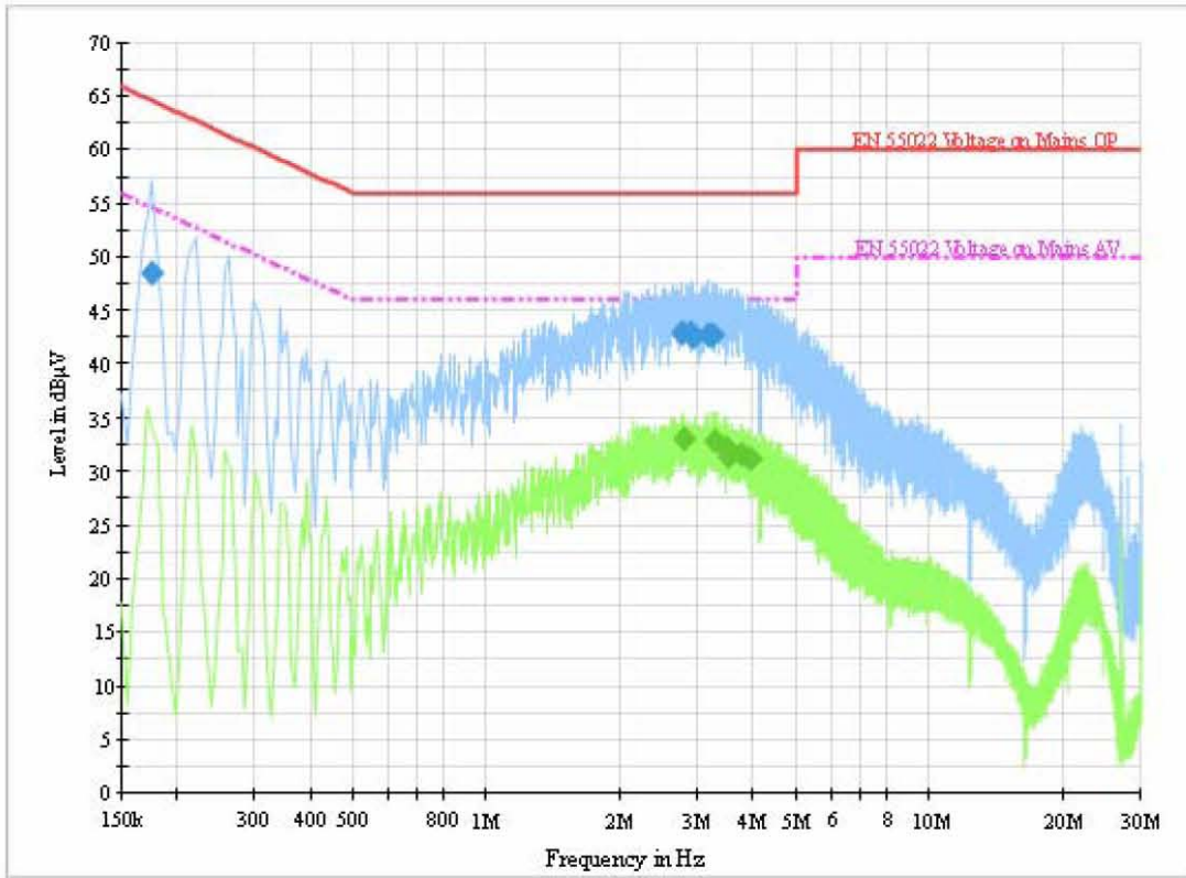
Figure A-9: Test result of EUT1 at test set. NFC02
