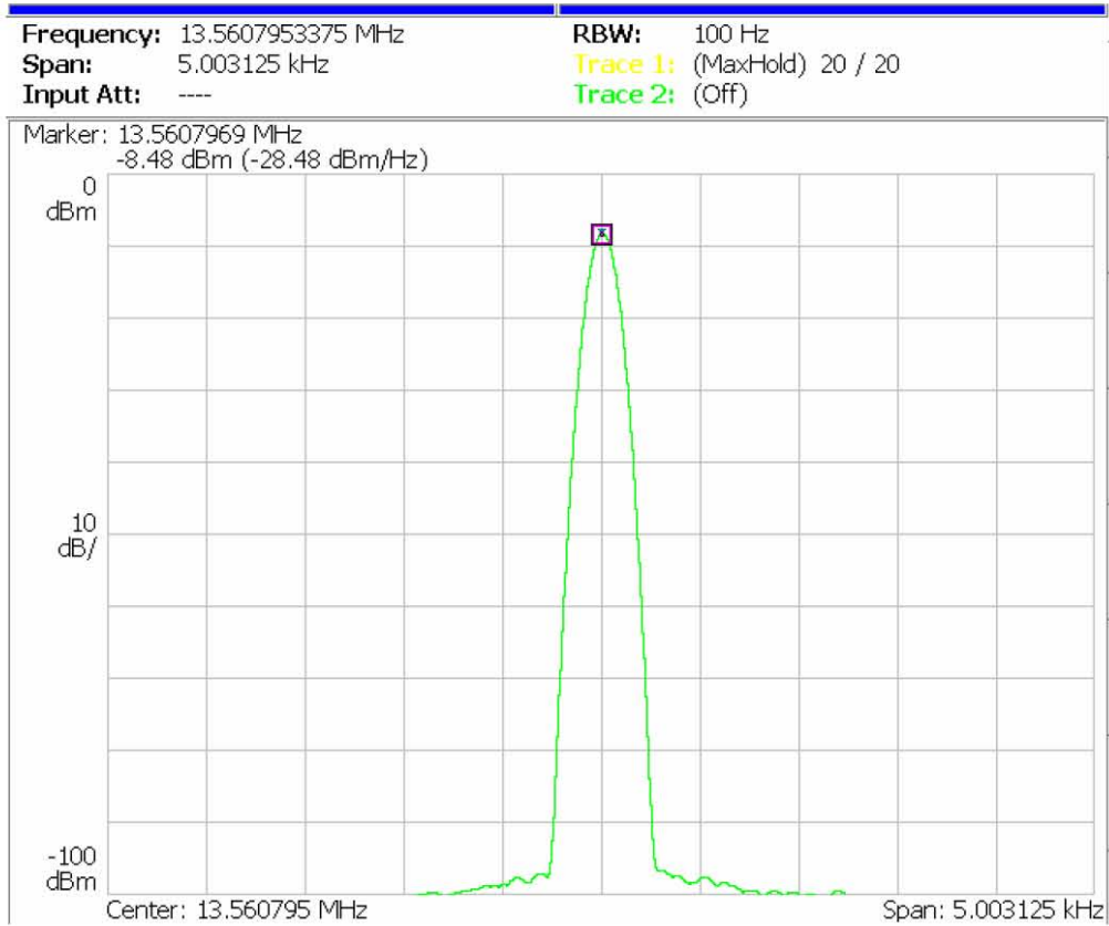
Figure A-6: Test result of EUT1 at test set. NFC03
