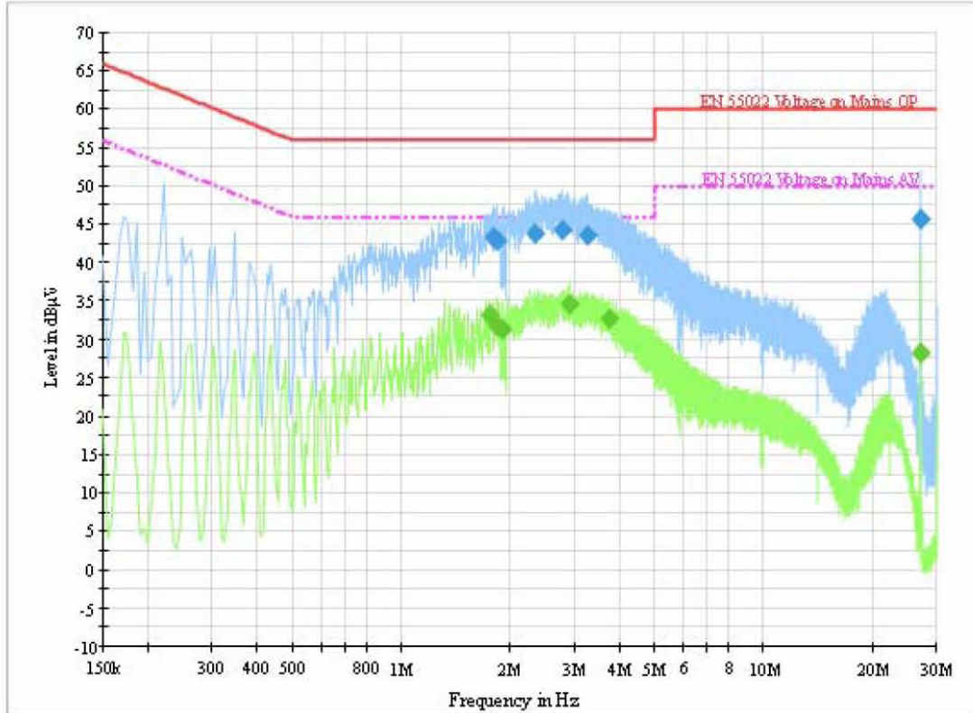
Figure A-8: Test result of EUT1 at test set. NFC01
