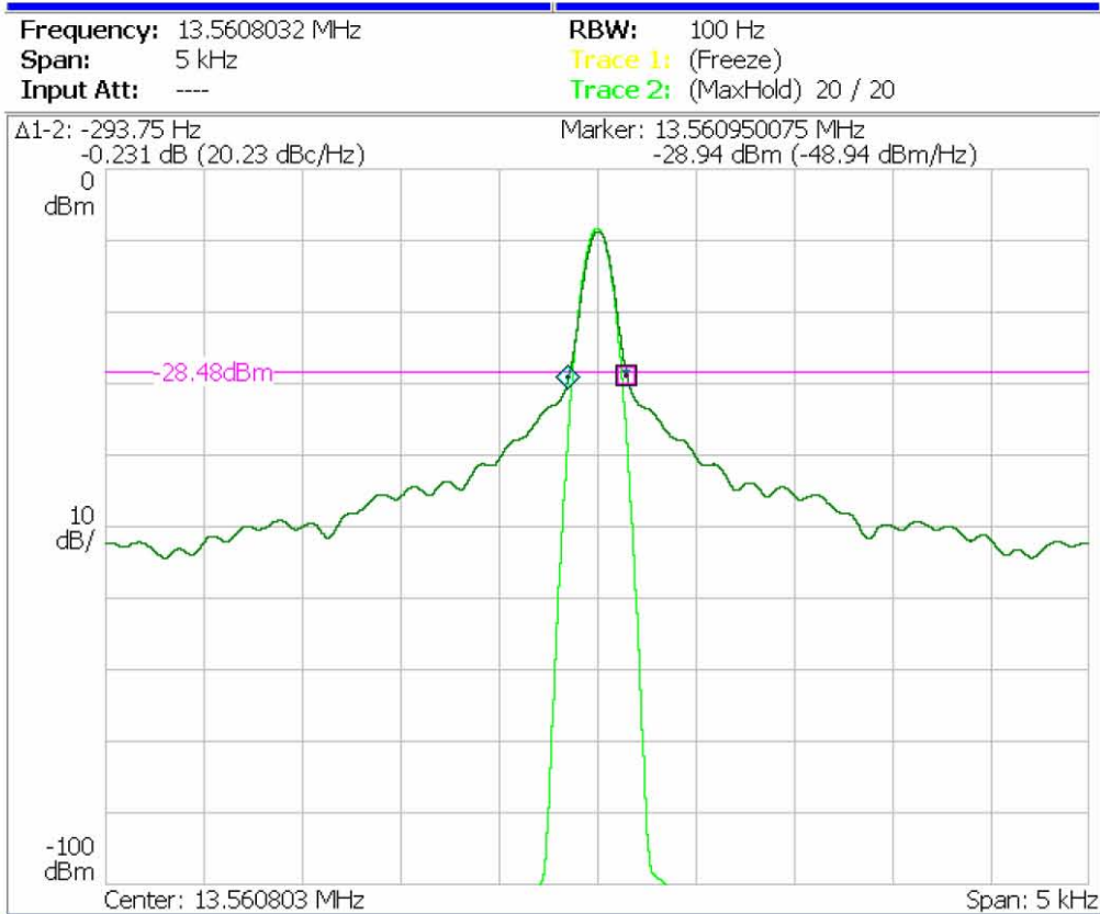
Figure A-7: Test result of EUT1 at test set. NFC04
