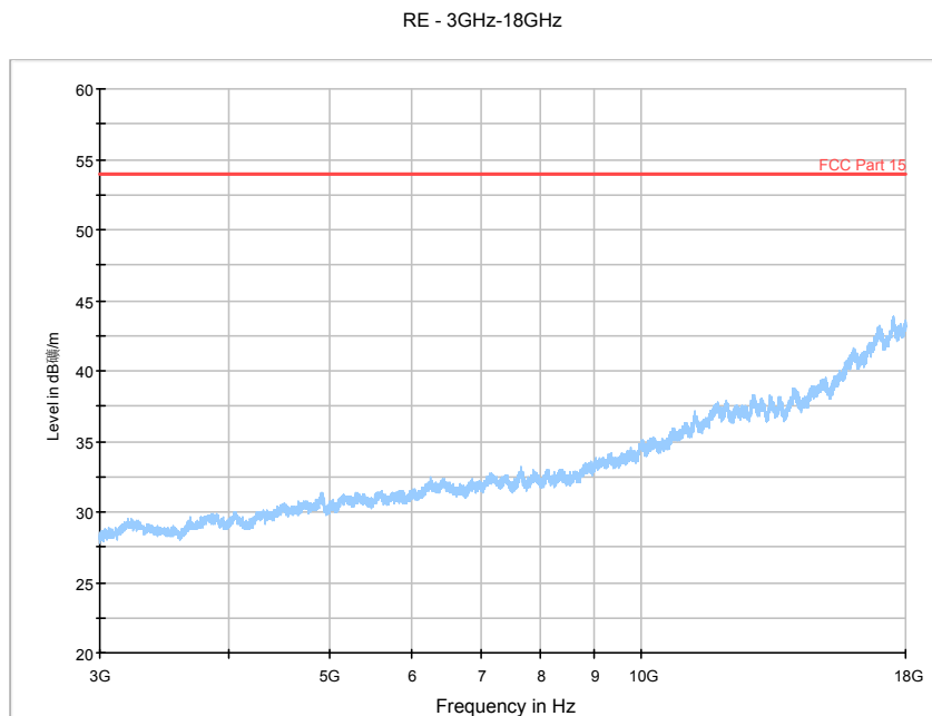
Fig. 168 Radiated Spurious Emission (802.11n-HT40, Ch6, 3 GHz-18 GHz)
