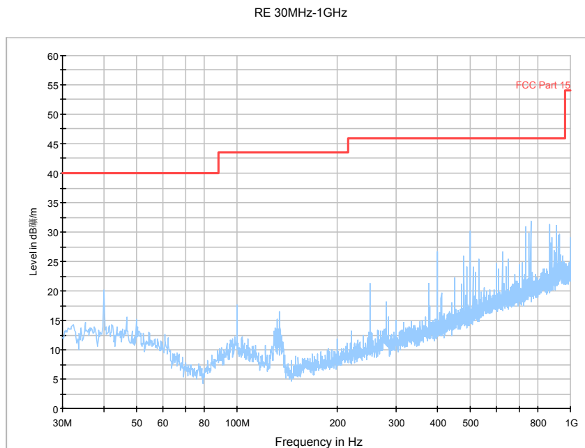
Fig. 170 Radiated Spurious Emission (802.11n-HT40, Ch9, 30 MHz-1 GHz)
