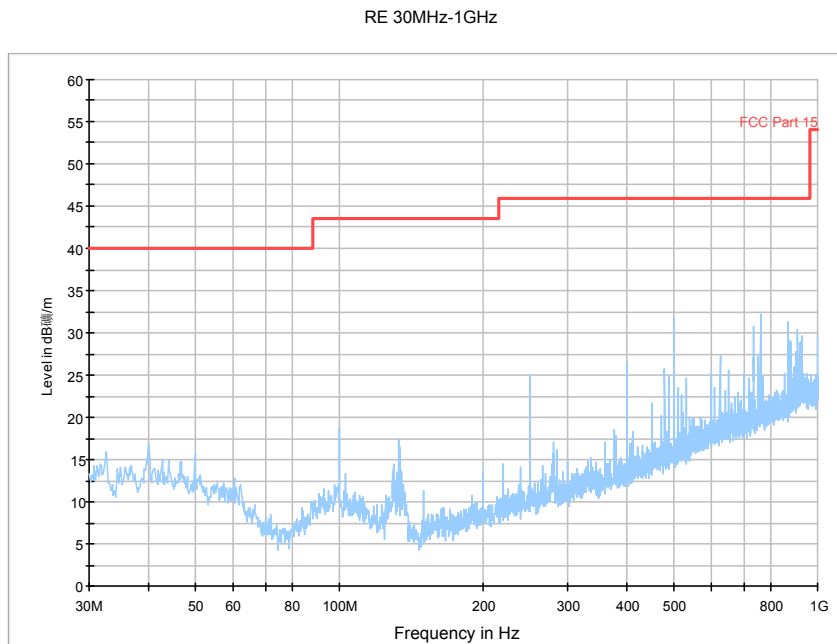
Fig. 166 Radiated Spurious Emission (802.11n-HT40, Ch6, 30 MHz-1 GHz)
