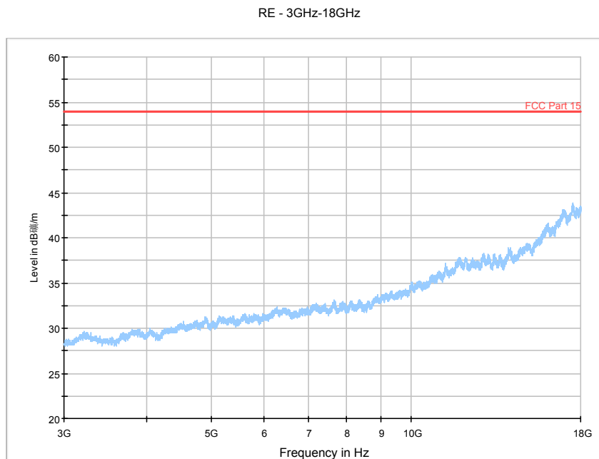
Fig. 154 Radiated Spurious Emission (802.11n-HT20, Ch1, 3 GHz-18 GHz)
