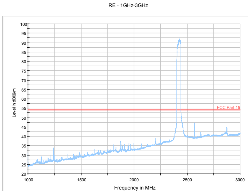
Fig. 164 Radiated Spurious Emission (802.11n-HT40, Ch3, 1 GHz-3 GHz)
