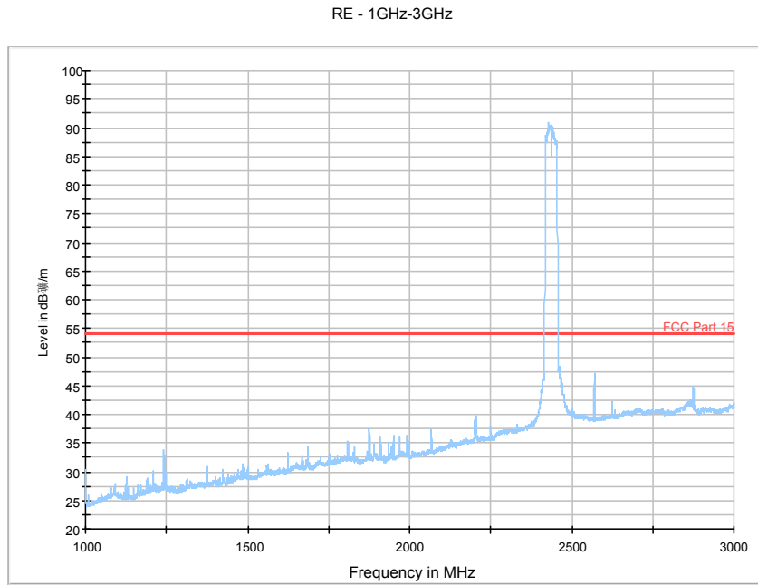
Fig. 167 Radiated Spurious Emission (802.11n-HT40, Ch6, 1 GHz-3 GHz)
