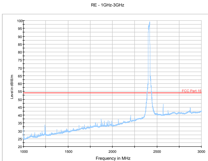
Fig. 142 Radiated Spurious Emission (802.11g, Ch1, 1 GHz-3 GHz)
