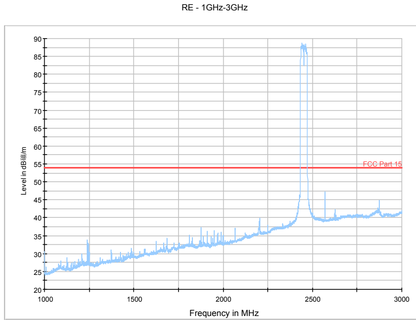
Fig. 171 Radiated Spurious Emission (802.11n-HT40, Ch9, 1 GHz-3 GHz)
