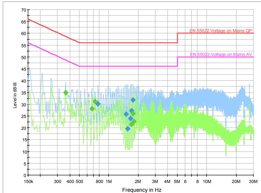
Fig. 174 AC Powerline Conducted Emission-802.11b
