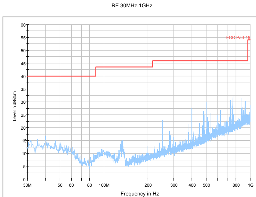
Fig. 163 Radiated Spurious Emission (802.11n-HT40, Ch3, 30 MHz-1 GHz)
