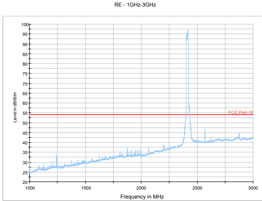
Fig. 153 Radiated Spurious Emission (802.11n-HT20, Ch1, 1 GHz-3 GHz)
