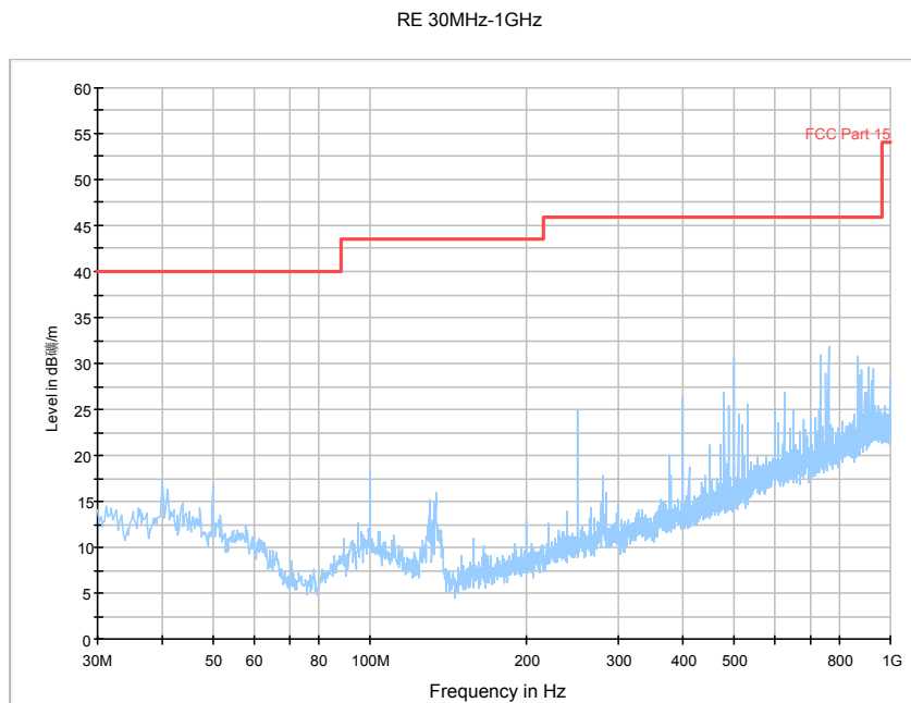
Fig. 141 Radiated Spurious Emission (802.11g, Ch1, 30 MHz-1 GHz)
