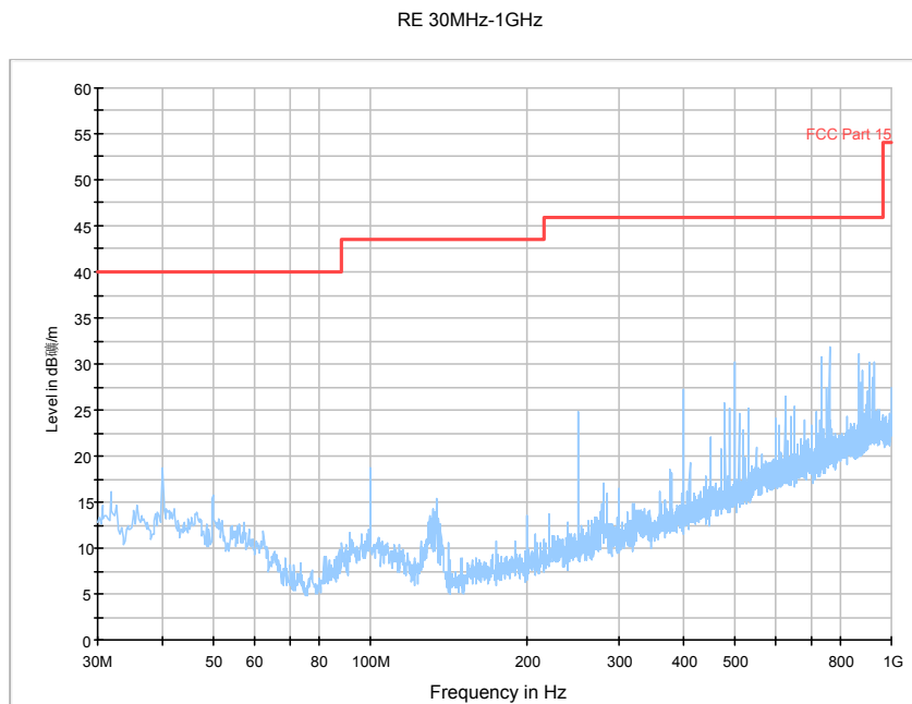
Fig. 159 Radiated Spurious Emission (802.11n-HT20, Ch11, 30 MHz-1 GHz)
