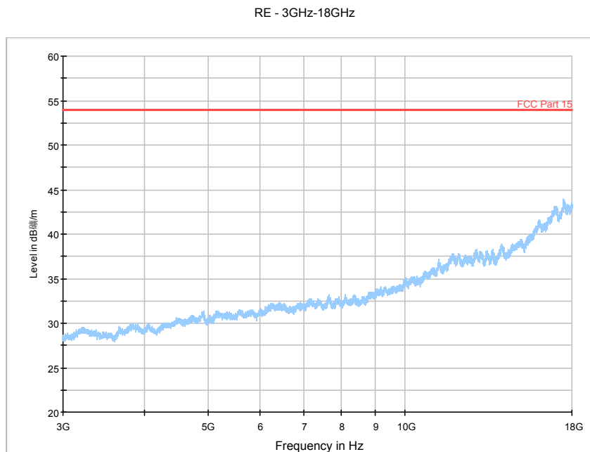
Fig. 172 Radiated Spurious Emission (802.11n-HT40, Ch9, 3 GHz-18 GHz)
