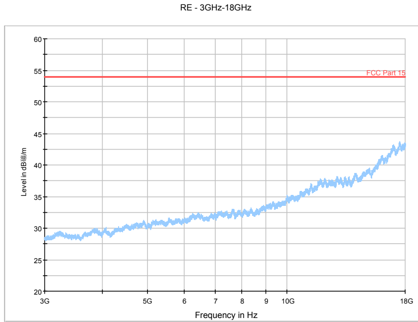
Fig. 165 Radiated Spurious Emission (802.11n-HT40, Ch3, 3 GHz-18 GHz)
