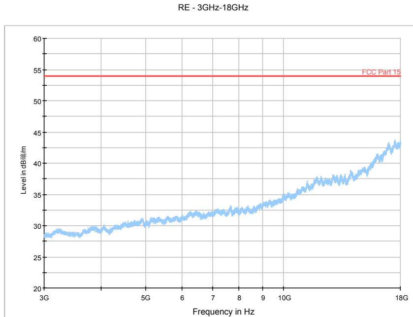
Fig. 157 Radiated Spurious Emission (802.11n-HT20, Ch6, 3 GHz-18 GHz)
