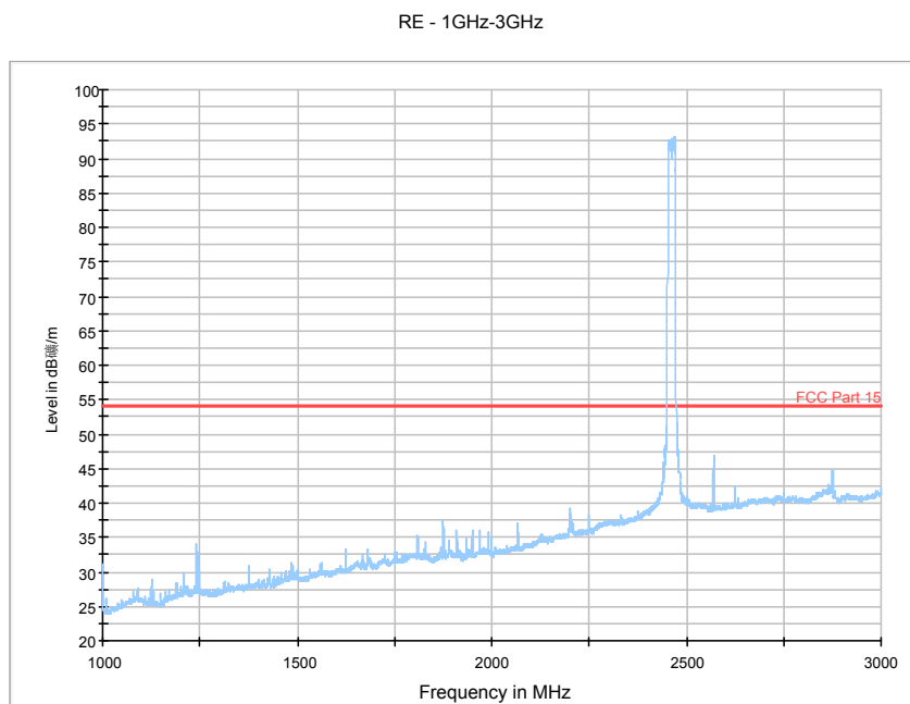
Fig. 160 Radiated Spurious Emission (802.11n-HT20, Ch11, 1 GHz-3 GHz)
