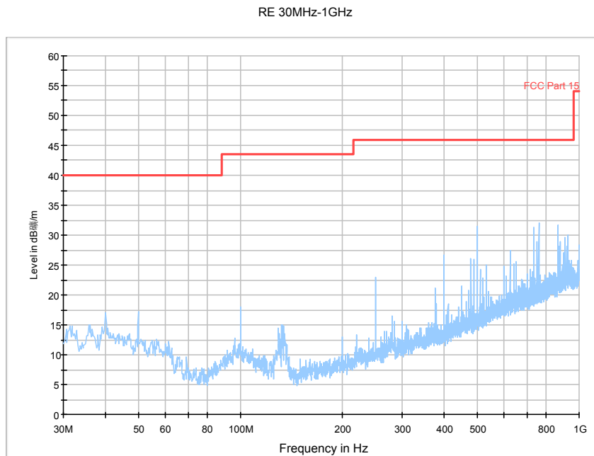
Fig. 155 Radiated Spurious Emission (802.11n-HT20, Ch6, 30 MHz-1 GHz)
