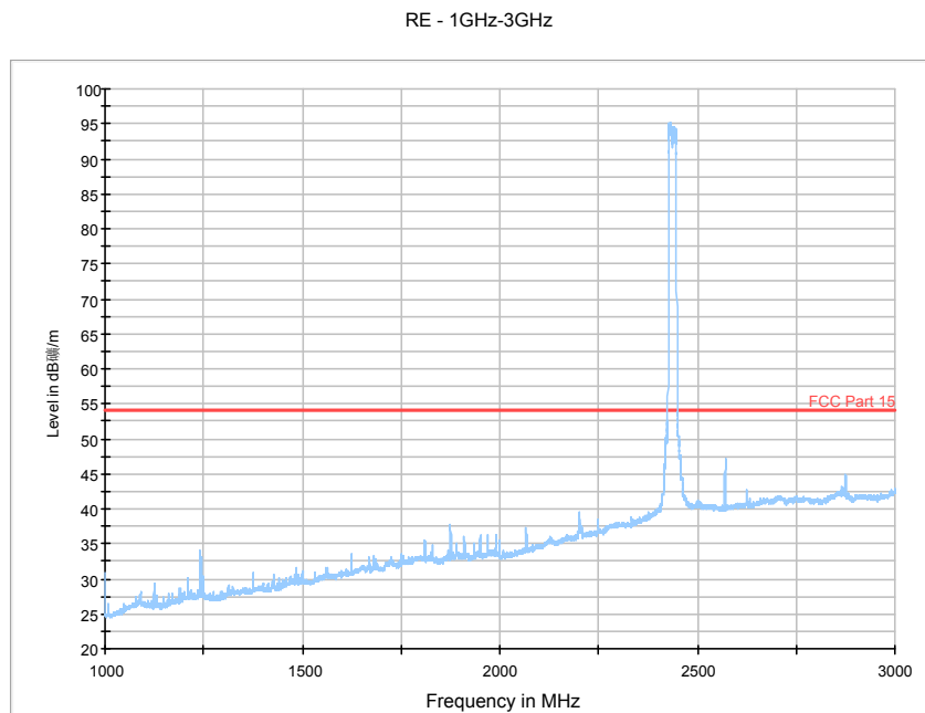
Fig. 156 Radiated Spurious Emission (802.11n-HT20, Ch6, 1 GHz-3 GHz)
