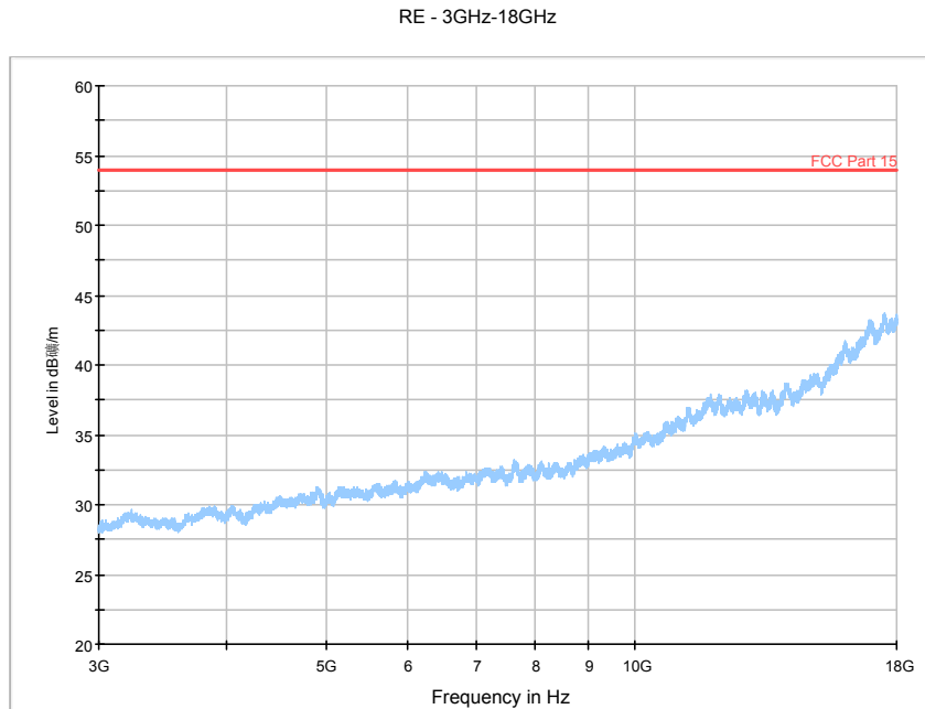
Fig. 161 Radiated Spurious Emission (802.11n-HT20, Ch11, 3 GHz-18 GHz)
