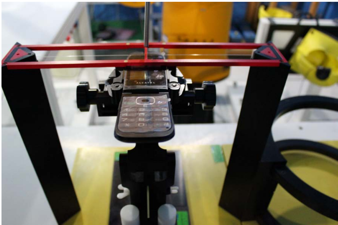
Picture 3: EUT Positioning for T-coil
