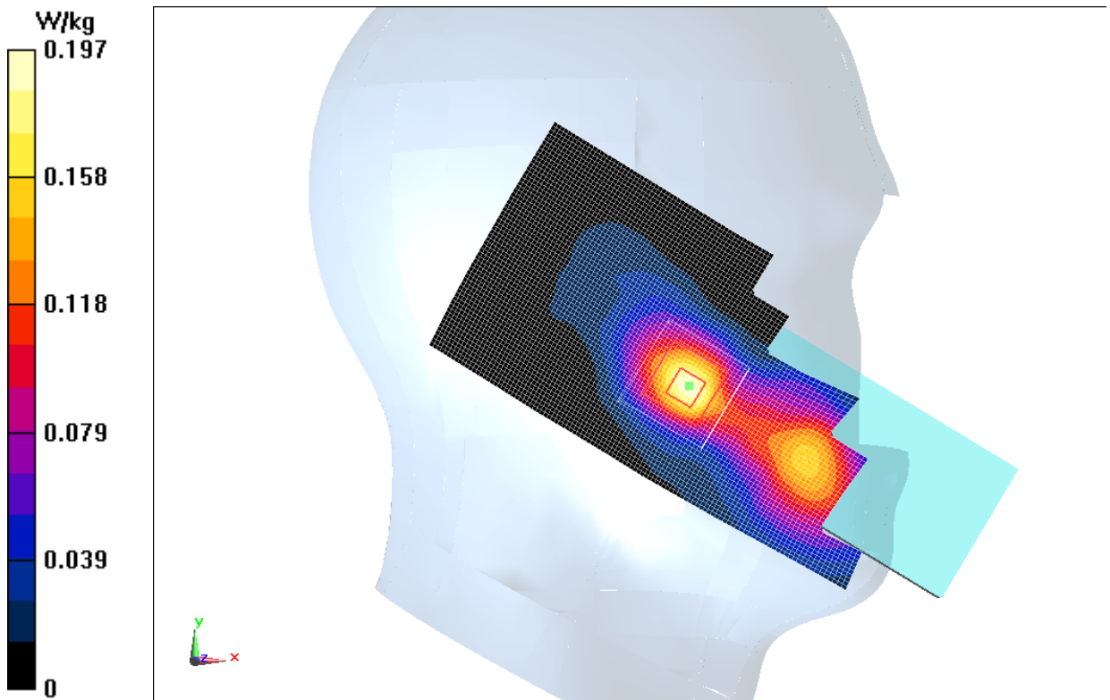
Fig.3 1900 MHz CH810
