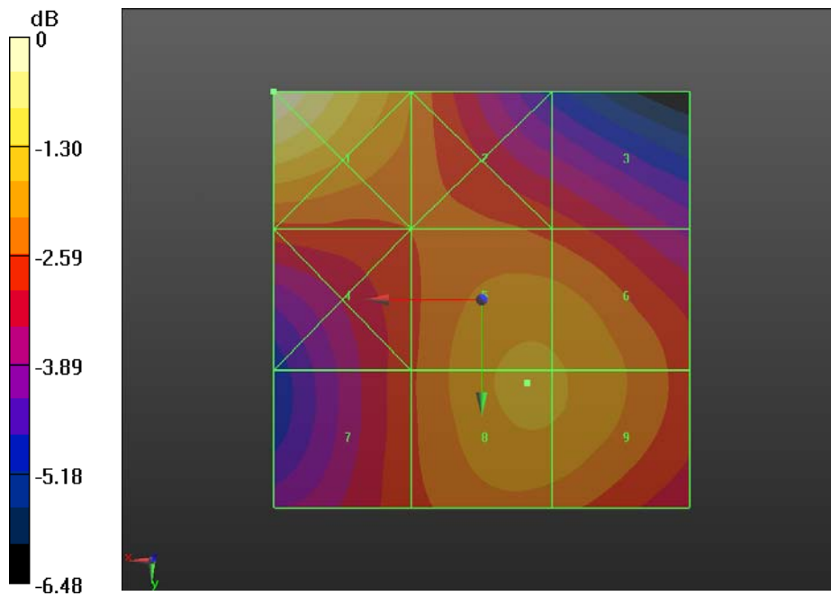
Fig B.17 HAC RF H-Field GSM 1900 Middle
