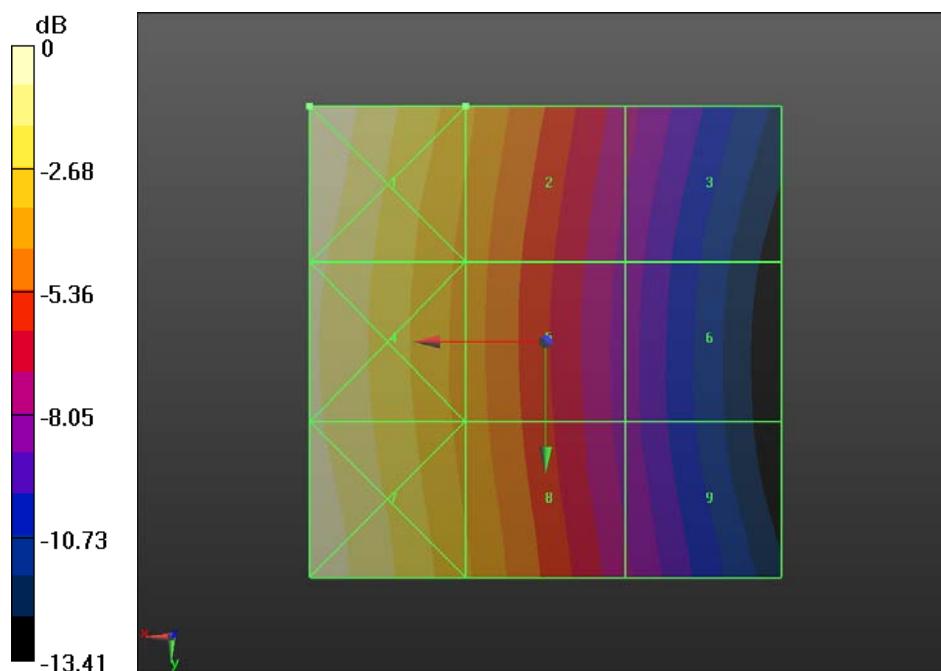
Fig B.13 HAC RF H-Field GSM 850 High
