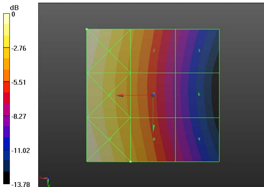
Fig B.20 HAC RF H-Field WCDMA 850 Middle
