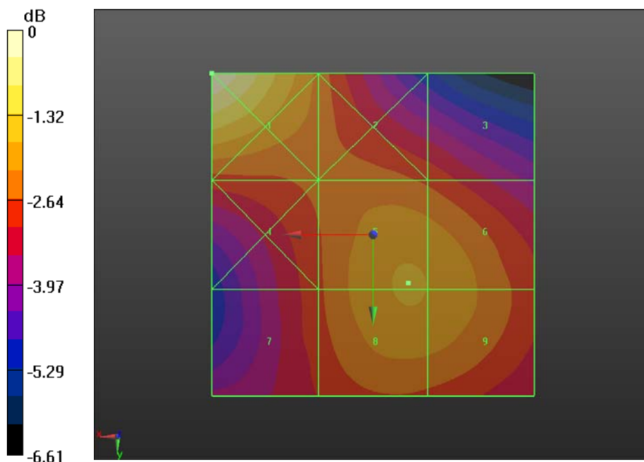
Fig B.18 HAC RF H-Field GSM 1900 Low
