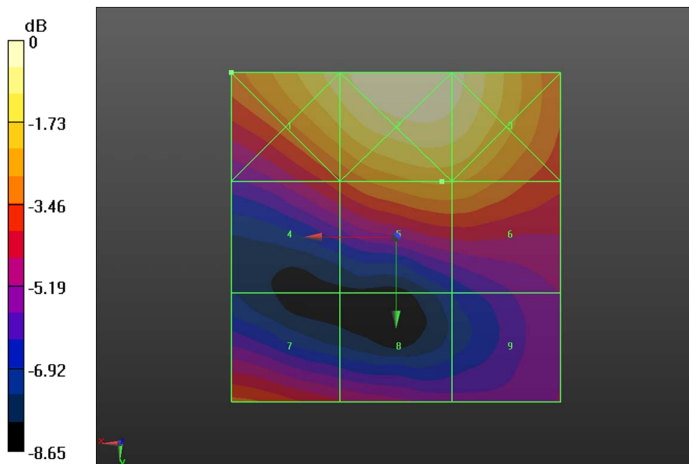
Fig B.4 HAC RF E-Field GSM 1900 High
