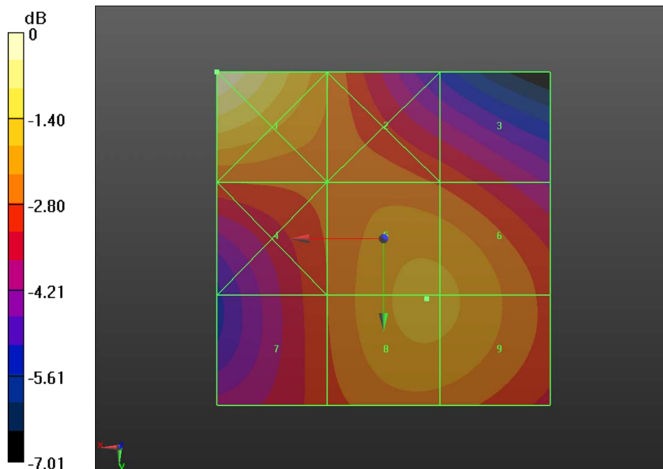
Fig B.24 HAC RF H-Field WCDMA 1900 Low
