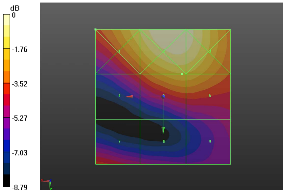
Fig B.10 HAC RF E-Field WCDMA 1900 High
