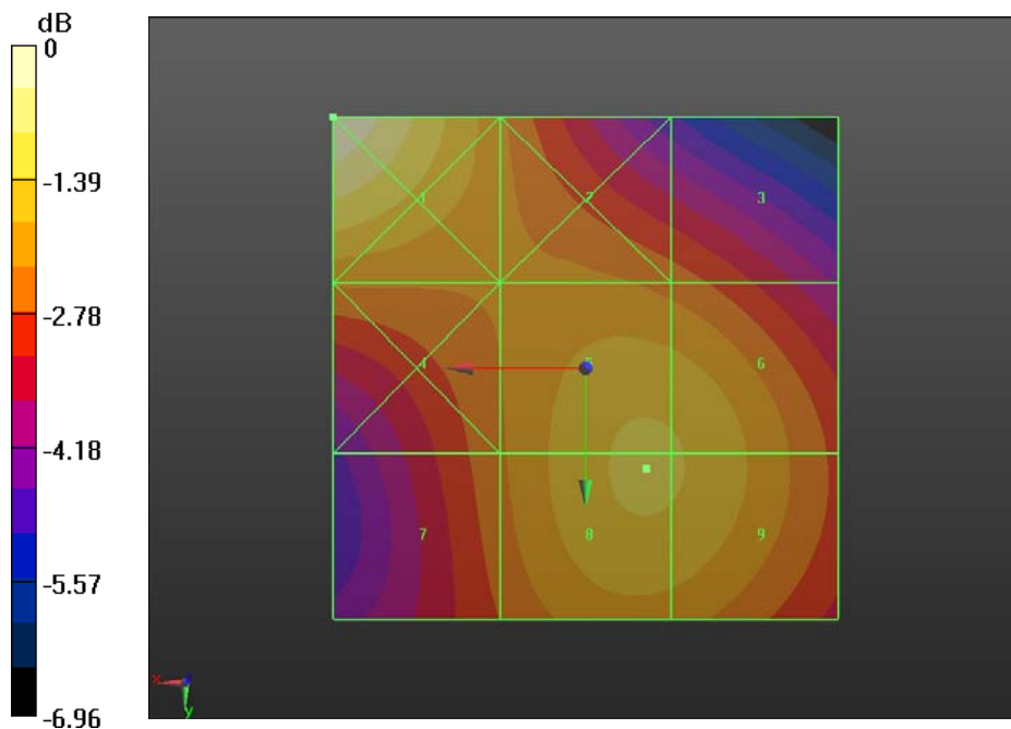
Fig B.22 HAC RF H-Field WCDMA 1900 High
