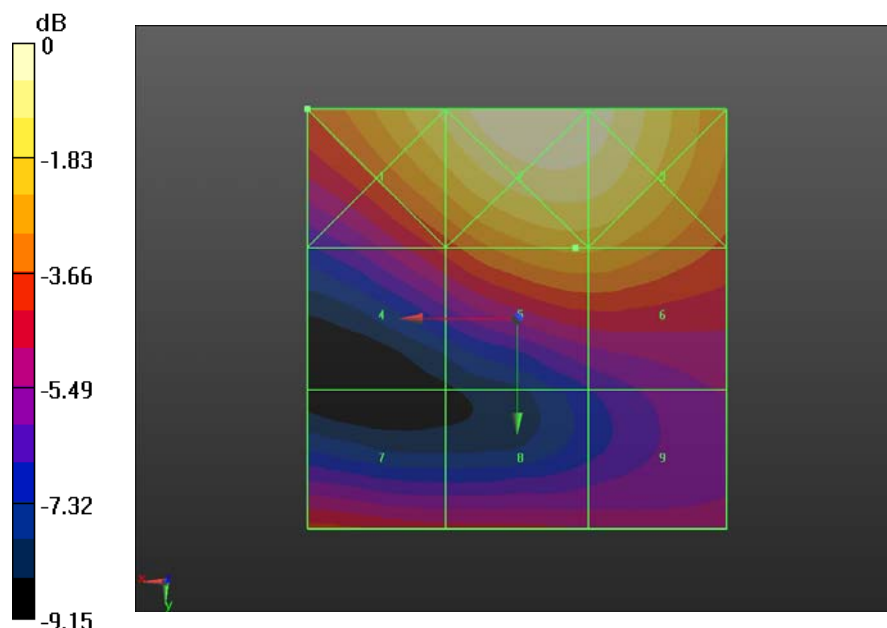
Fig B.12 HAC RF E-Field WCDMA 1900 Low
