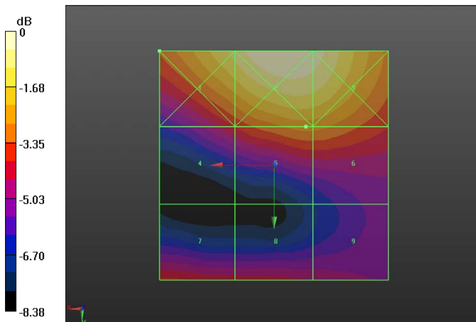
Fig B.6 HAC RF E-Field GSM 1900 Low
