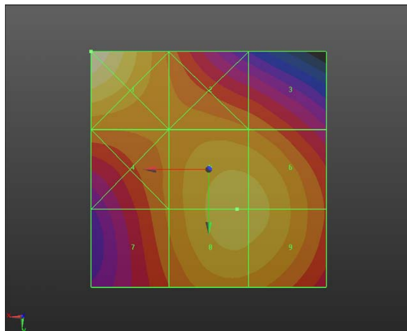
Fig B.16 HAC RF H-Field GSM 1900 High
