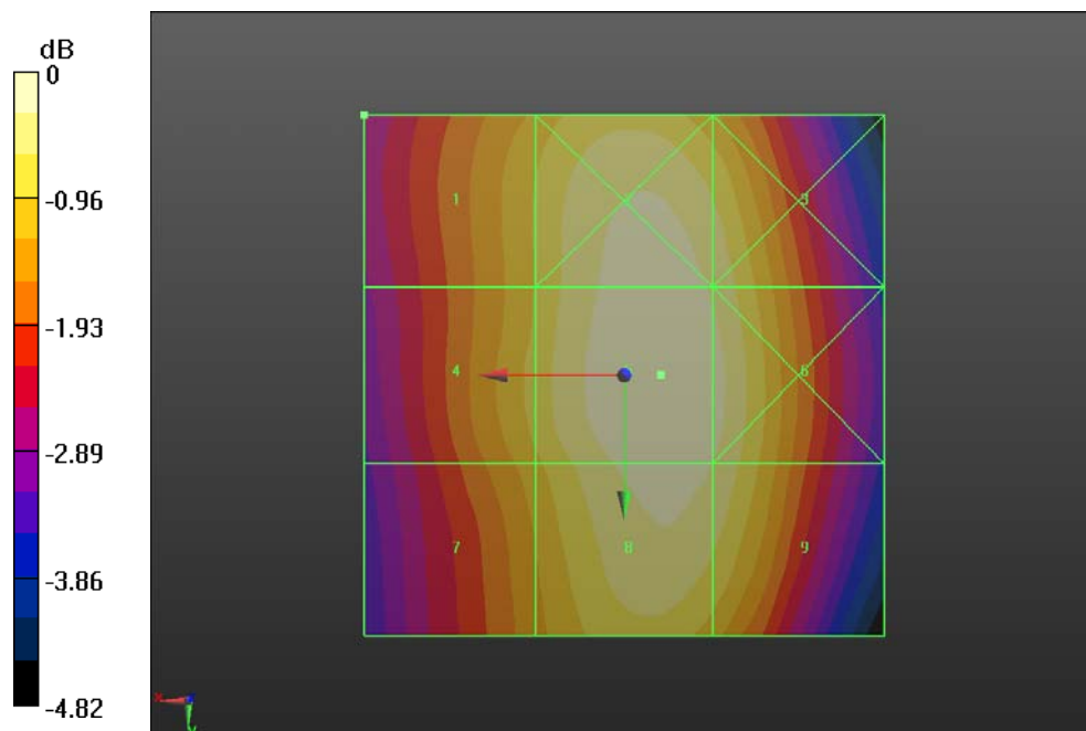
Fig B.9 HAC RF E-Field WCDMA 850 Low
