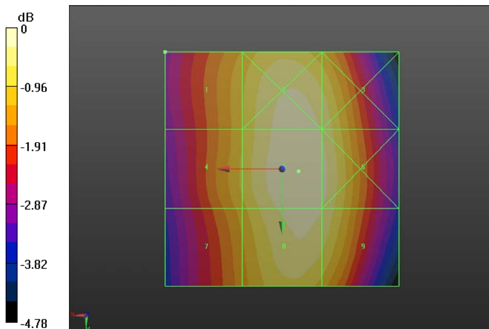
Fig B.7 HAC RF E-Field WCDMA 850 High
