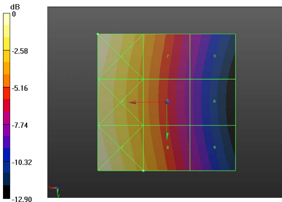
Fig B.19 HAC RF H-Field WCDMA 850 High
