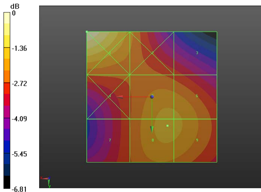
Fig B.23 HAC RF H-Field WCDMA 1900 Middle
