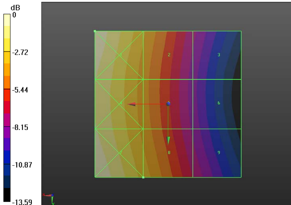
Fig B.21 HAC RF H-Field WCDMA 850 Low
