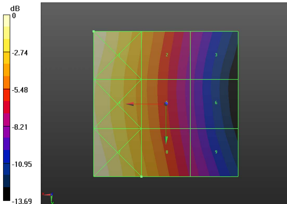
Fig B.15 HAC RF H-Field GSM 850 Low
