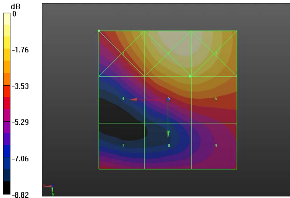
Fig B.11 HAC RF E-Field WCDMA 1900 Middle
