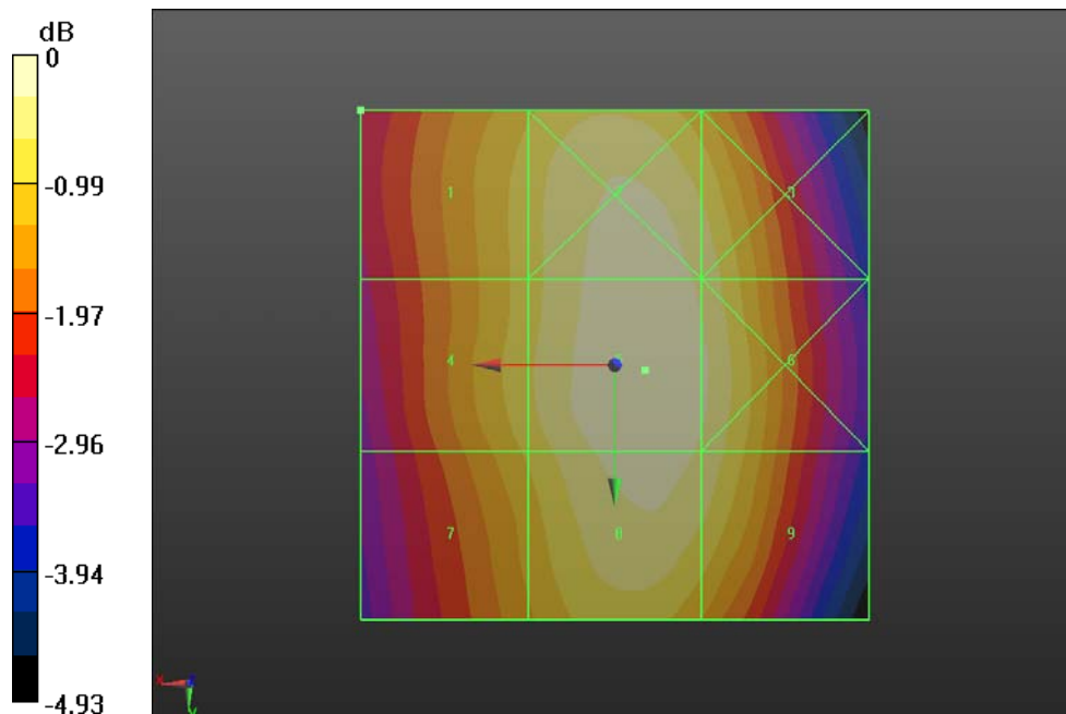
Fig B.3 HAC RF E-Field GSM 850 Low
