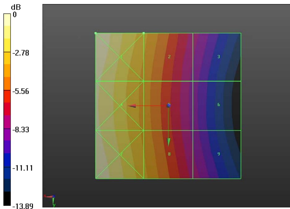
Fig B.14 HAC RF H-Field GSM 850 Middle
