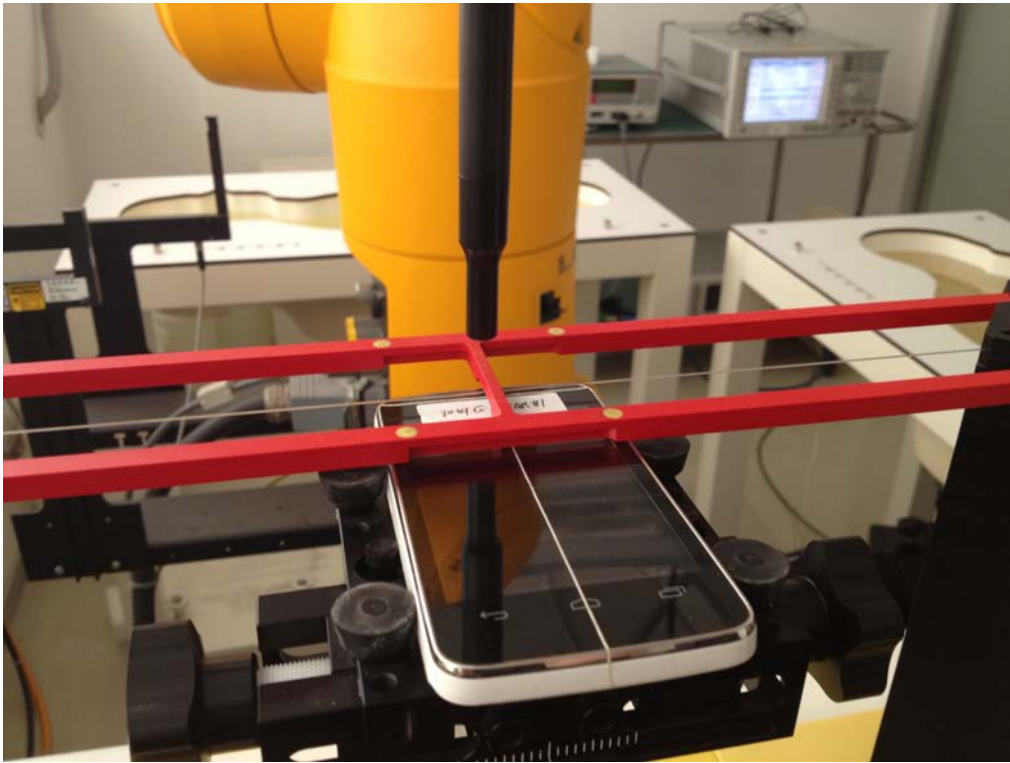
Picture 3: EUT Positioning for RF
