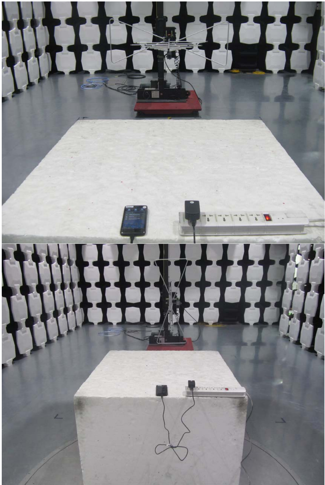
5. Radiated Emission(USB)
