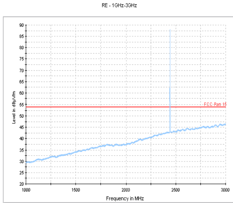
Fig.22. Radiated emission: GFSK, 2440MHz, 1 GHz - 3 GHz
